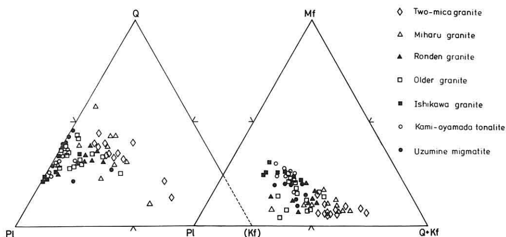
Text-Figure 4 Volumetric proportion of constituent minerals in the migmatite, tonalite and granites. Q: quartz, Pl: plagioclase, Kf: potash feldspar, Mf: biotite and hornblende
