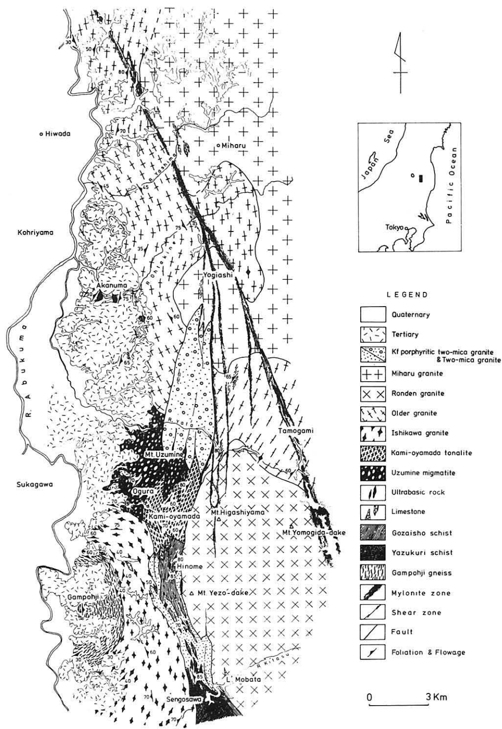
Text-Figure 1 Geological map of the Miharu-Uzumine-Sengosawa district.
