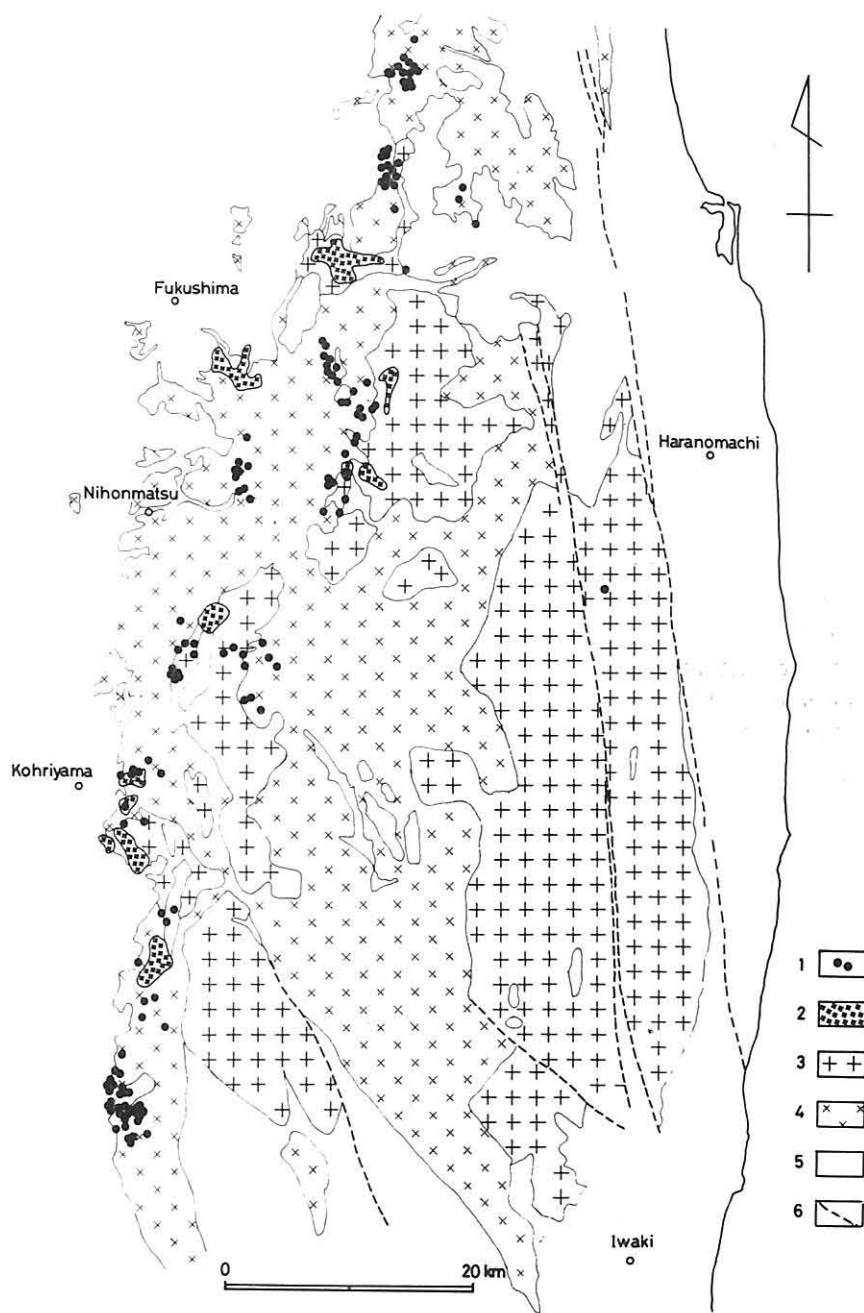
Text-Figure 9 Distribution of two-mica granites and pegmatites in the Abukuma Plateau. The map is modified from the map given by the Nakadohri Collaborating Research Group (in Minato et al. , 1979). 1: pegmatite, 2: two-mica granite, 3: the older granite, 4: the younger granite, 5: metamorphics and Tertiary and Quaternary deposits, 6: sheared zone.
