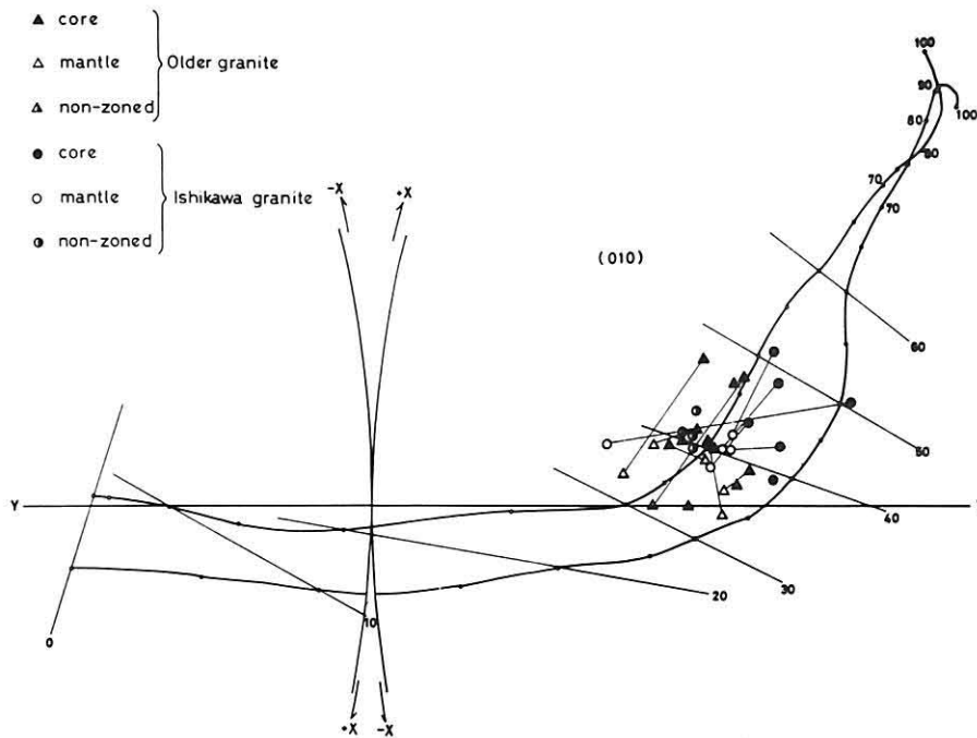
Text-Figure 6 Projection of optical constants of plagioclases of the Ishikawa and the older granites on the Burri et al. 's migration curve.
