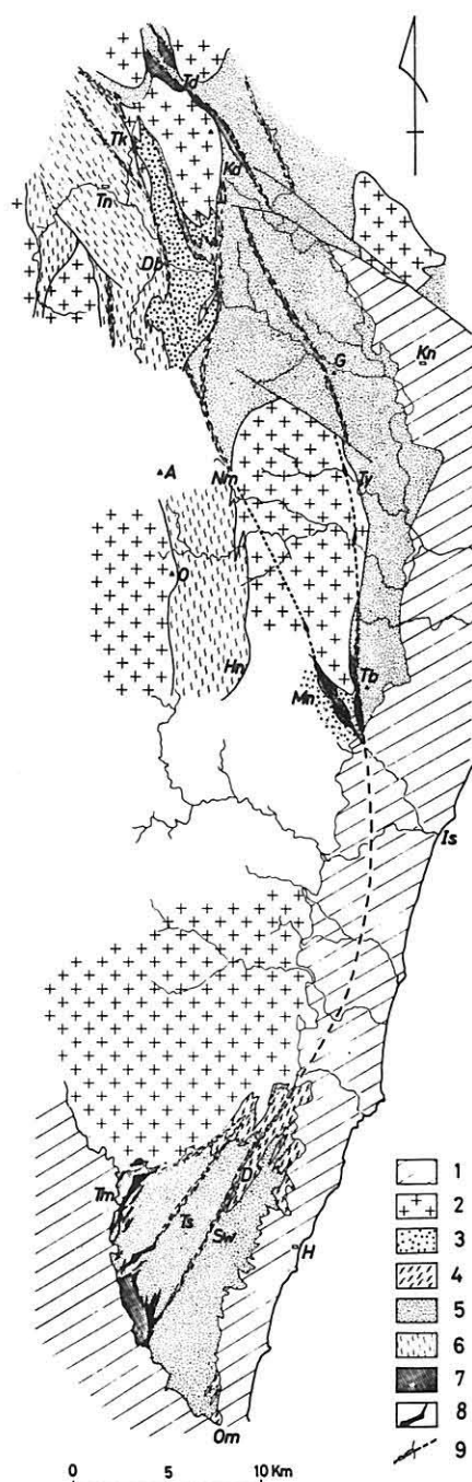
Text-Figure 10 Geologic sketch map of the Koshidai-Takaboyama-Daioh-in structural belt. After Watanabe et al. (1978).
