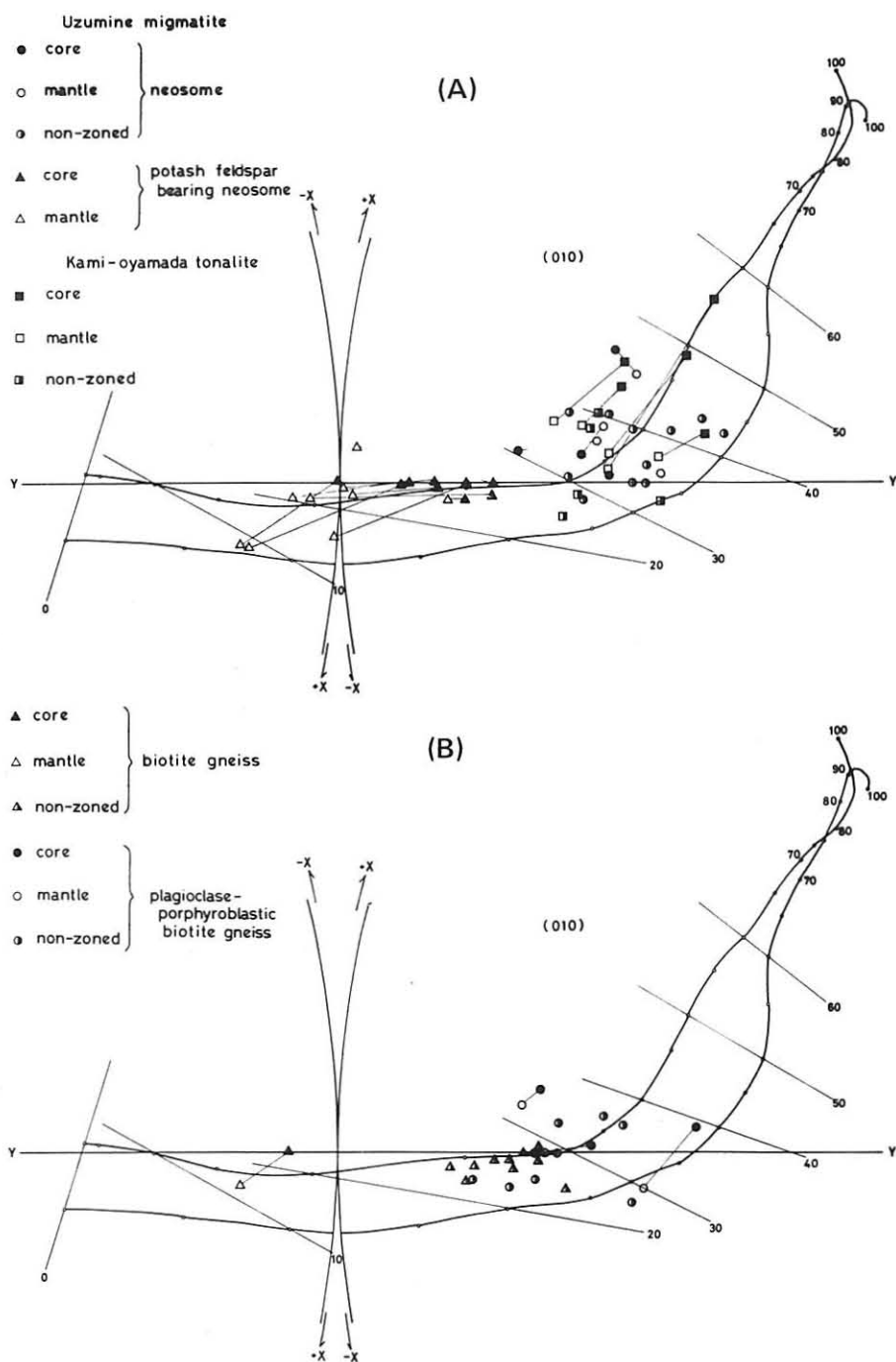
Text-Figure 5 Projection of optical constants of plagioclases of the migmatite and the tonalite on the Burri et al. 's migration curve.
