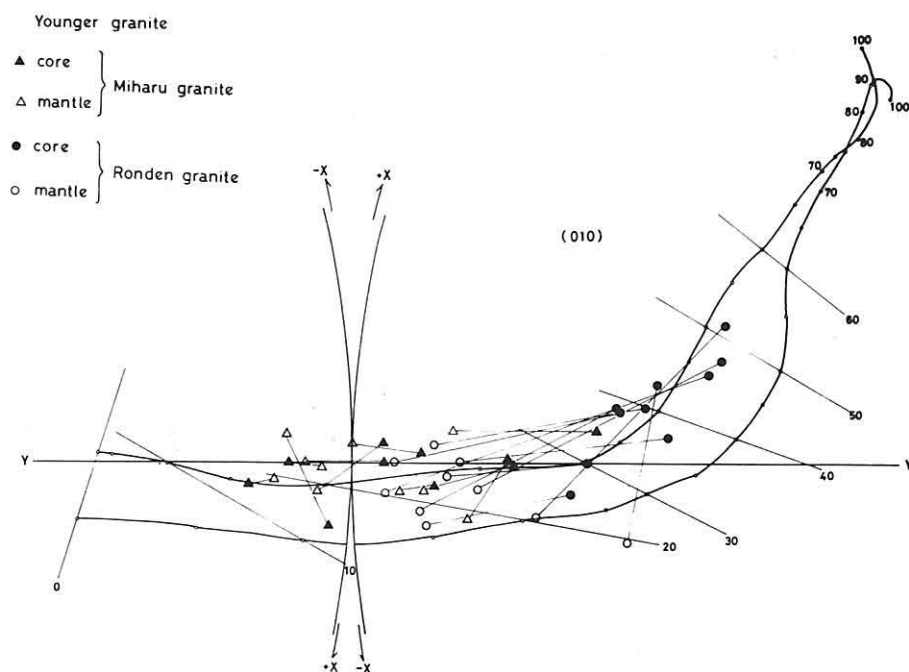
Text-Figure 7 Projection of optical constants of plagioclases of the Miharu and the Ronden granites on the Burri et al. 's migration curve.
