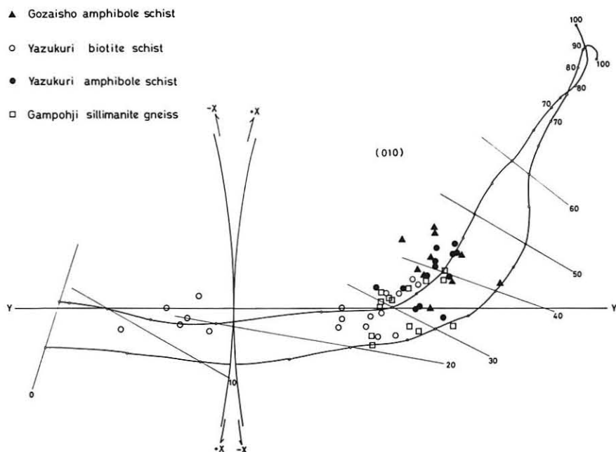
Text-Figure 2 Projection of optical constants of plagioclases of metamorphic rocks on the Burri et al. 's migration curve.
