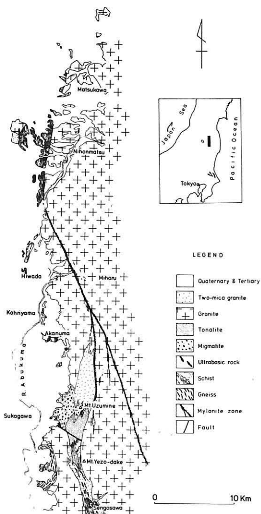
Text-Figure 11 Geologic sketch map of the Nakadohri and Uzumine-Sengosawa districts. The map is compiled based on the map given by the Nakadohri Collaborating Research Group and the present study.
