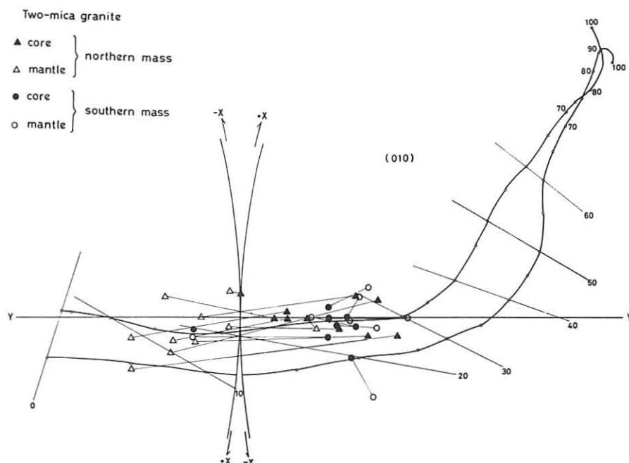
Text-Figure 8 Projection of optical constants of plagioclases of the two-mica granite on the Burri et al. 's migration curve.
