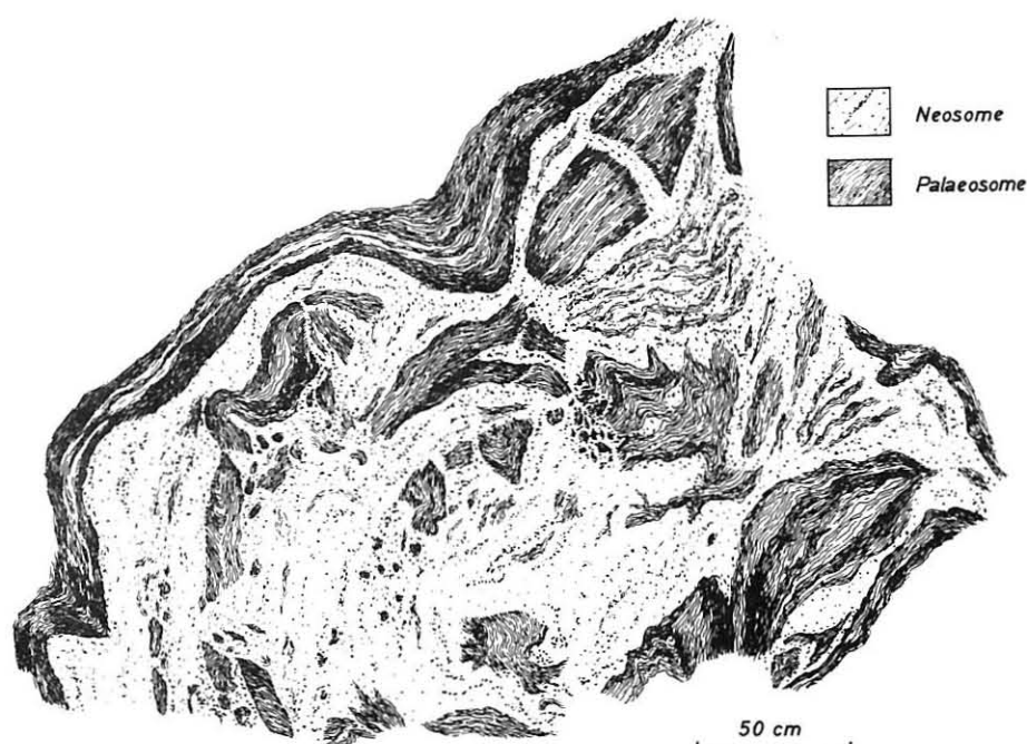
Text-Figure 3 A sketch showing an occurrence of the Uzumine migmatite.
