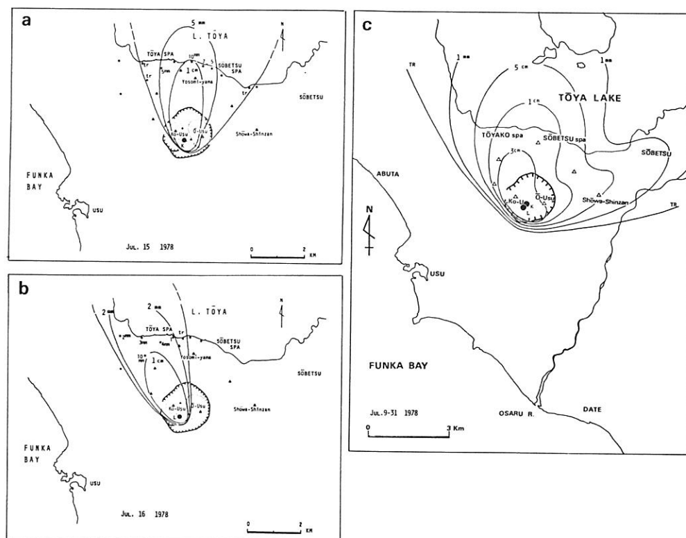
Text-fig. 4 Map showing the distribution and thickness of the ash-fall deposits: (a) July 15, (b) July 16, 1978, and (c) cumulative thickness contour lines of the ash-fall deposits produced in July, 1978.
