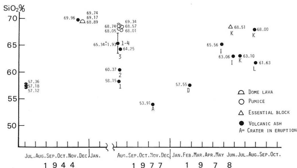
Text-fig. 12 Relation between the sequence of eruption and the \text{SiO}_2 contents of ejecta. Source of data: Minakami et al. (1951), Yagi (1949), Oba (1966), Matsuo et al. (1977), Katsui et al. (1978), Hokkaido Natl. Agric. Exp. Stn. (1978), Kondō et al. (unpubl.)
