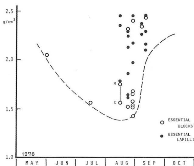
Text-fig. 11 Variation of the apparent densities of the essential dacite blocks and lapilli.
