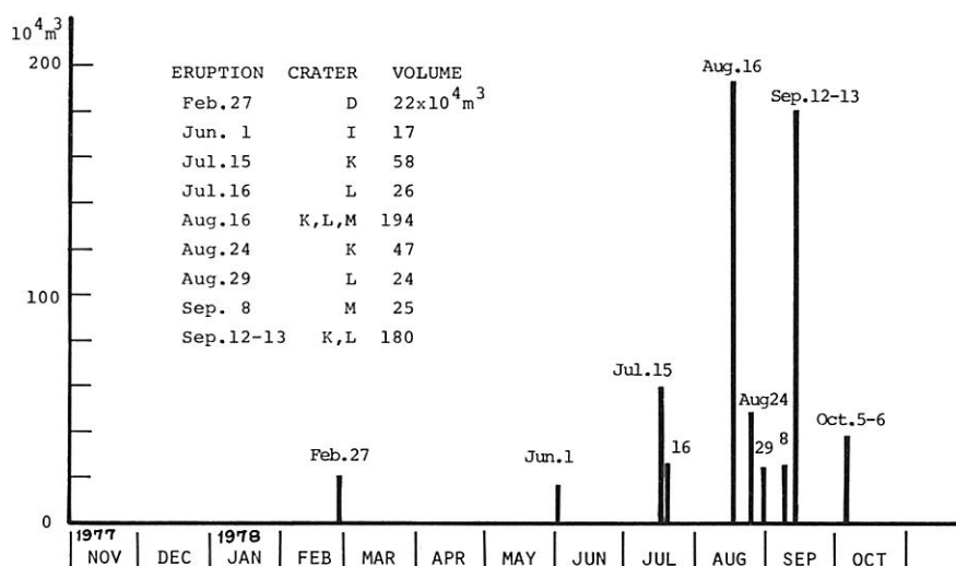
Text-fig. 8 Volume of the ejecta produced by notable eruptions in the Second Stage.
