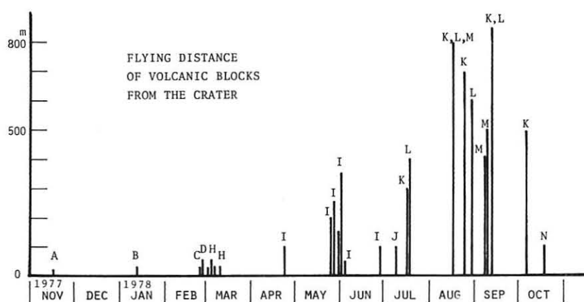
Text-fig. 13 Flying distance of the volcanic blocks from the crater.
