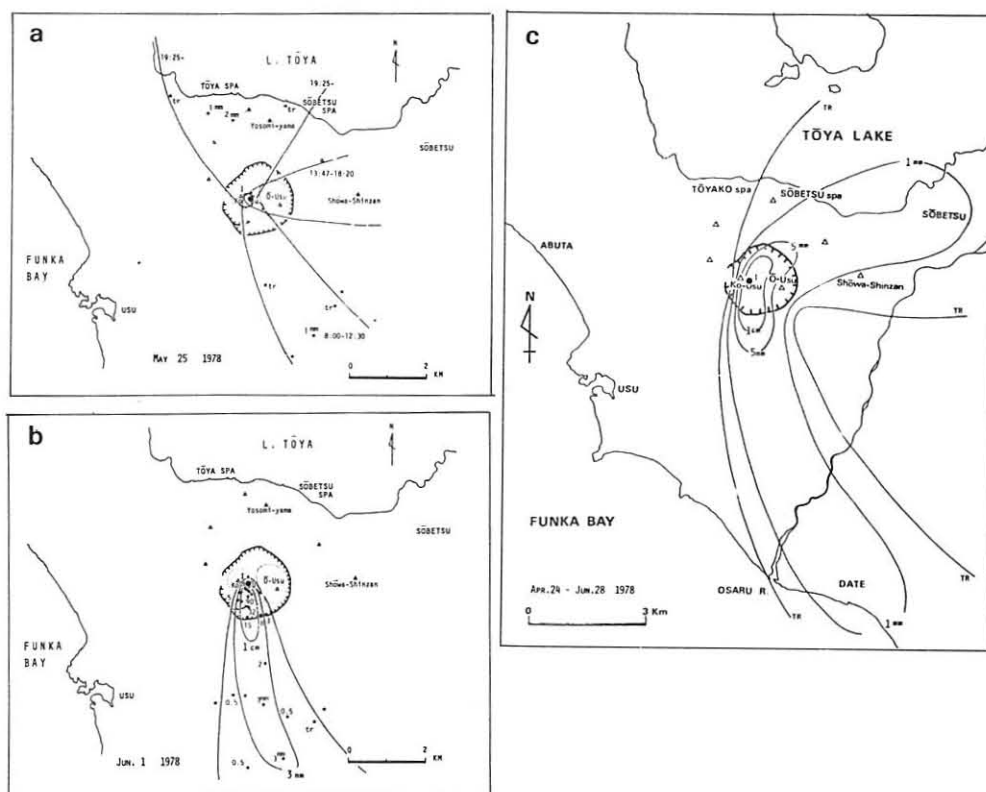
Text-fig. 3 Map showing the distribution and thickness of the ash-fall deposits; (a) May 25, (b) June 1, 1978, and (c) cumulative thickness contour lines of the ash-fall deposits produced during April 24 and June 28, 1978.
