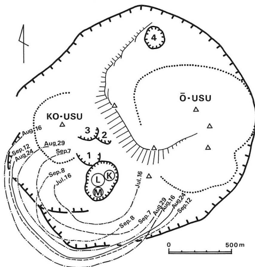
Text-fig. 14 Map showing the distribution limit of the volcanic blocks ejected by the Substage III eruptions.
