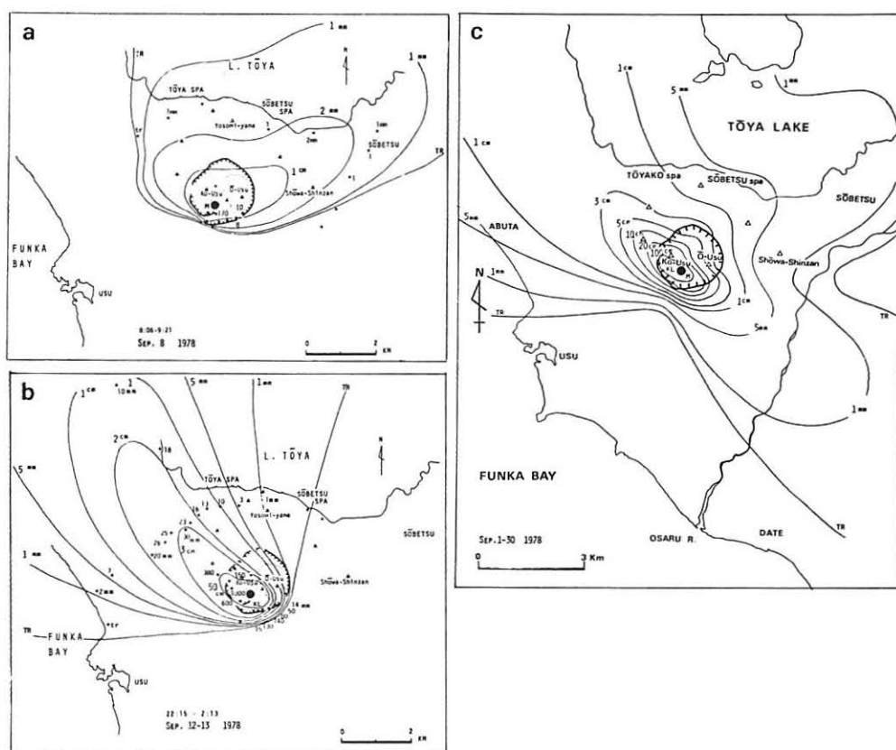
Text-fig. 6 Map showing the distribution and thickness of the ash-fall deposits; (a) September 8, (b) September 12-13, 1978, and (c) cumulative thickness contour lines of the ash-fall deposits produced in September, 1978.
