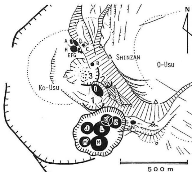
Text-fig. 1 Localities of the craters produced by the Second Stage eruption in 1977-1978.
