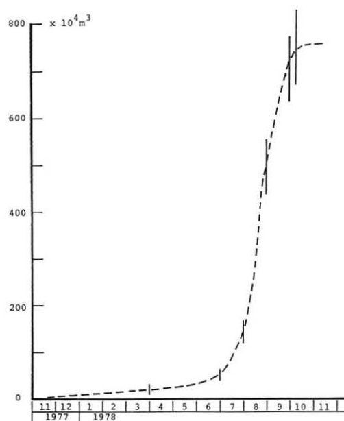
Text-fig. 9 Cumulative curve for the volume of ejecta produced in the Second Stage.
