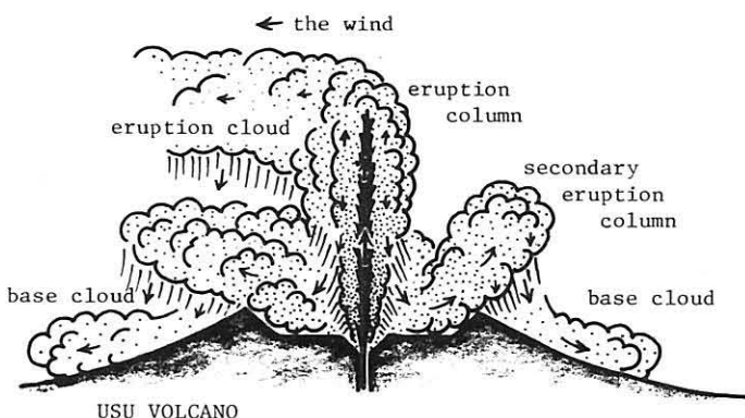
Text-fig. 16 Schematic diagram showing the growth mechanism of secondary eruption column and base cloud occurred on August 16 and September 7 and 8, 1978.
