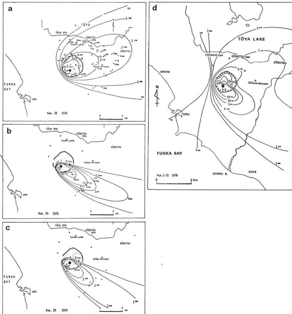
Text-fig. 5 Map showing the distribution and thickness of the ash-fall deposits; (a) August 16, (b) August 24, (c) August 29, 1978, and (d) cumulative thickness contour lines of the ash-fall deposits produced in August, 1978.
