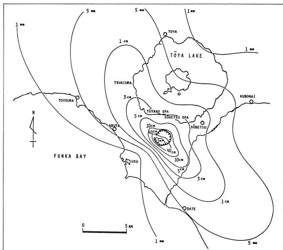
Text-fig. 7 Map showing the cumulative thickness contour lines of the ejecta produced by the Second Stage eruptions in 1977-1978.
