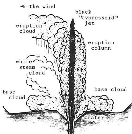
Text-fig. 15 Schematic diagram showing the growth mechanism of base cloud formed by phreatomagmatic eruptions from July to August, 1978.
