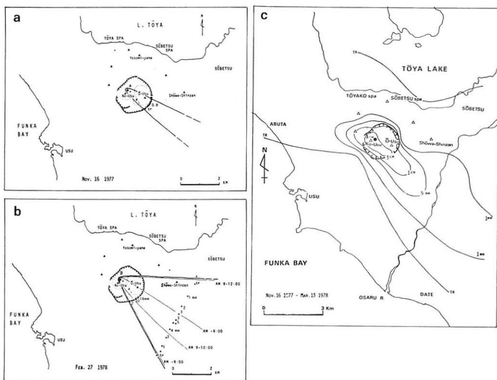
Text-fig. 2 Map showing the distribution and thickness of the ash-fall deposits; (a) November 16, 1977, (b) February 27, 1978, and (c) cumulative thickness contour lines of the ash-fall deposits produced during November 16, 1977, and March 13, 1978.
