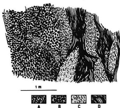
Text-fig. 6 Sketch showing the relation between the massive and foliated types of ultrabasic rocks.
