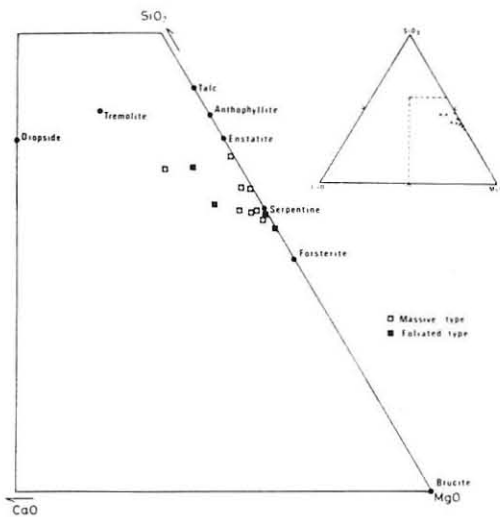
Text-fig. 13 CaO-MgO-SiO 2 diagram for the ultrabasic rocks near Machiya Town. Open squares: massive type, Solid squares: foliated type
