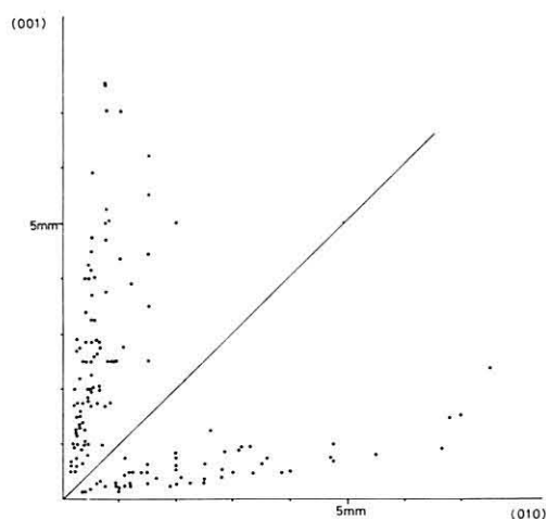
Text-fig. 8 Distribution of elongated olivine porphyroblast in terms of the variation of crystal size in (001)-axis versus (010)-axis.
