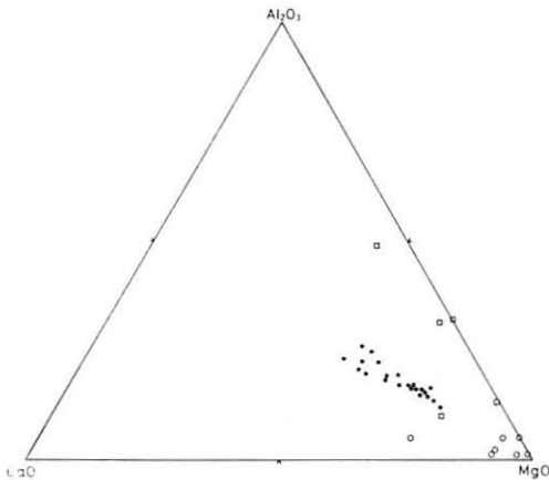
Text-fig. 12 \text{Al}_2\text{O}_3 -CaO-MgO diagram for the ultrabasic rocks. Open circles: massive type of the ultrabasic rocks near Machiya Town, Squares: foliated type of the ultrabasic rocks near Machiya Town, Solid circles: peridotitic komatiite of Belingwe greenstone belt, Rhodesia (Nisbet et al., 1977) and spinifex bearing rocks of Munro Township, Ontario (Pyke et al., 1973)
