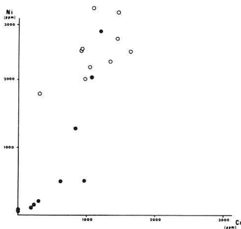
Text-fig. 10 Ni-Cr diagram of the ultrabasic rocks from Machiya Town. Open circles: massive type Solid circles: foliated type
