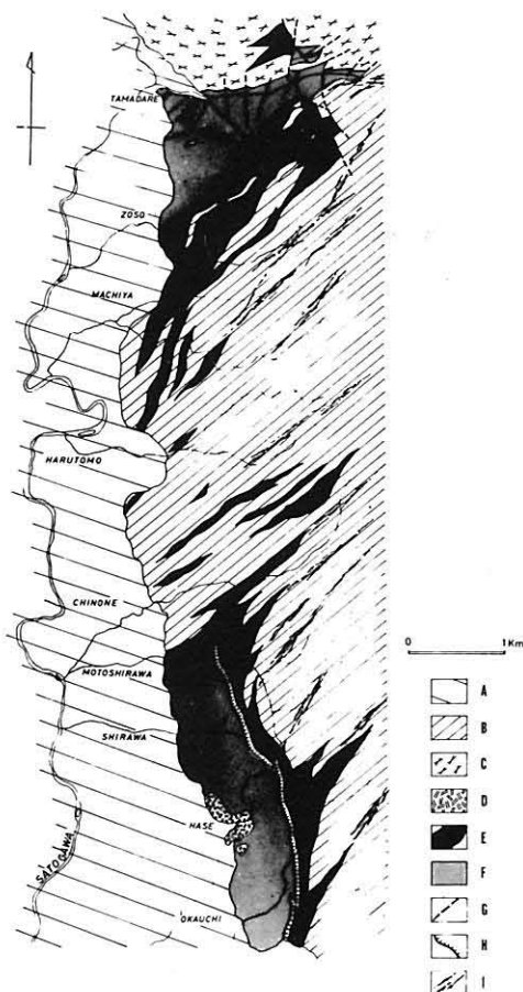
Text-fig. 2 (Right) Map showing the distribution of the ultrabasic rocks in the western Hitachi area.
