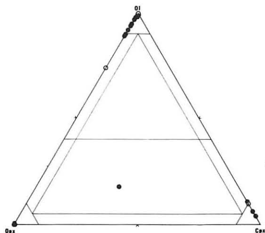
Text-fig. 15 Modal proportions of olivine, orthopyroxene and clinopyroxene of the ultrabasic rocks from Koshidai and Hanazono districts, Abukuma Plateau.
