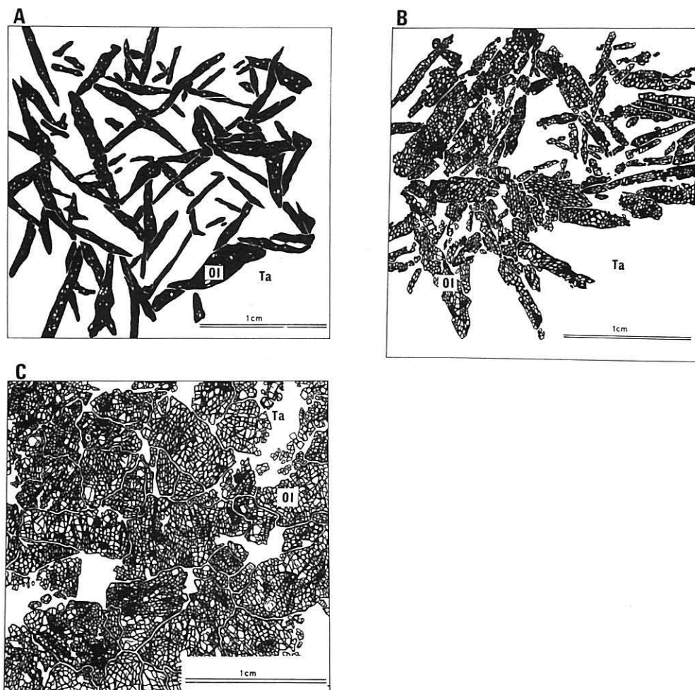
Text-fig. 7 Manner of olivine porphyroblast from the massive type (typical "Madaraishi").
