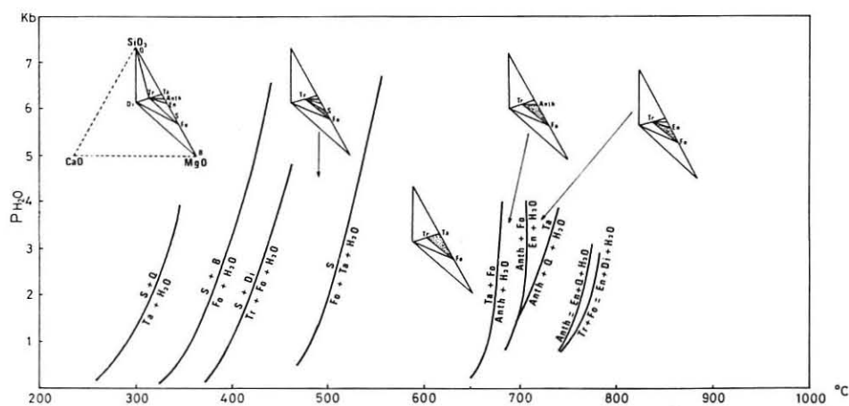
Text-fig. 14 Sequence of metamorphic reactions in serpentinite (after Evans and Trommsdorff, 1970).
