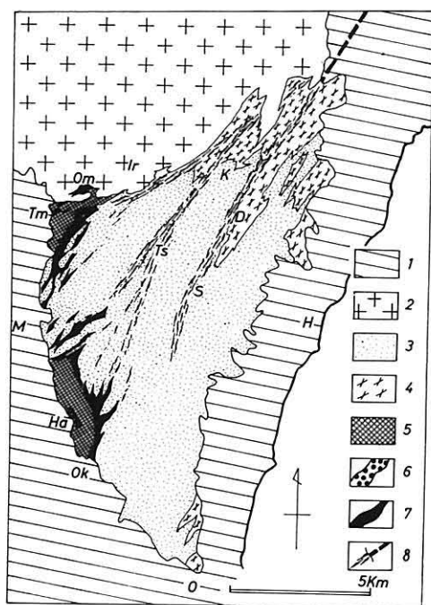
Text-fig. 1 (Left) Geological map showing distribution of the Koshidai-Takaboyama-Daioh'in Structural Belt in the Hitachi district.
