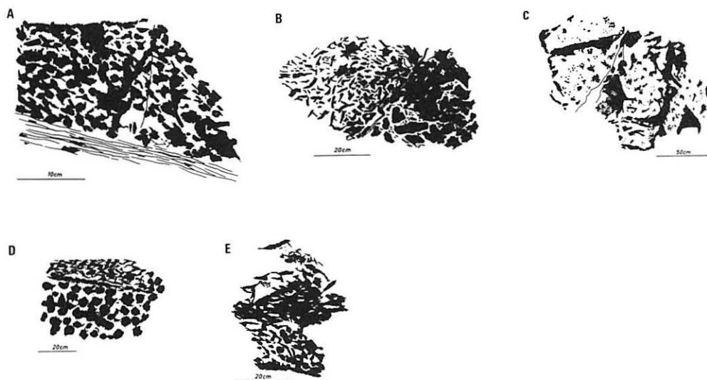
Text-fig. 3 Variation of dappled structure of "Madaraishi".
