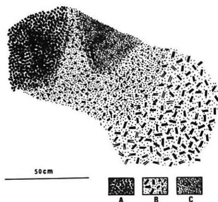
Text-fig. 5 Sketch of an outcrop showing rock facies of massive type.
