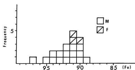
Text-fig. 9 Frequency distribution of forsterite content in olivine.
