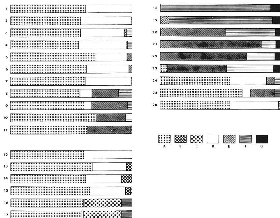
Text-fig. 4 Modal compositions of ultrabasic rocks from near Machiya Town.
