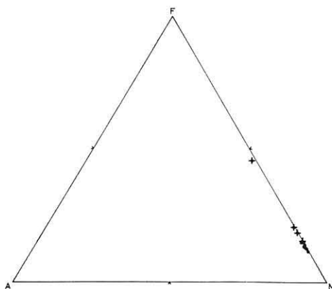
Text-fig. 11 AFM triangular plots of the ultrabasic rocks from Machiya Town. Solid circles: massive type Crosses: foliated type
