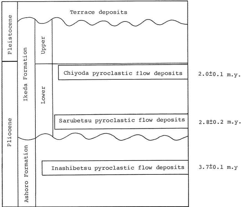
Text-fig. 2. Generalized stratigraphic column showing horizons of measured pyroclastic flow deposits in the eastern Hokkaido, Japan.
