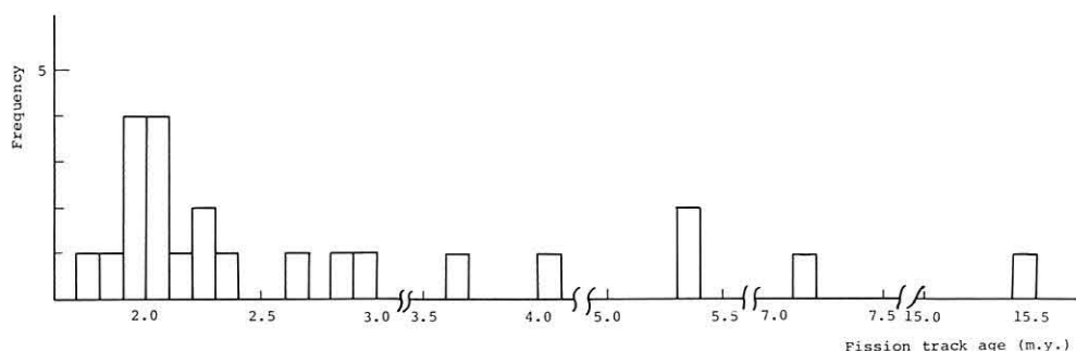
Text-fig. 5. Distribution of determined ages on 23 grains of zircon from the Chiyoda pyroclastic flow deposits (see Table 3). 14 grains in the left hand corner of the figure will consist a normal population. See explanation of Text-fig. 3.
