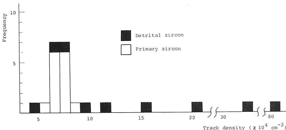
Text-fig. 8. Histogram of spontaneous fission track density of zircons from the Chiyoda pyroclastic flow deposits.
