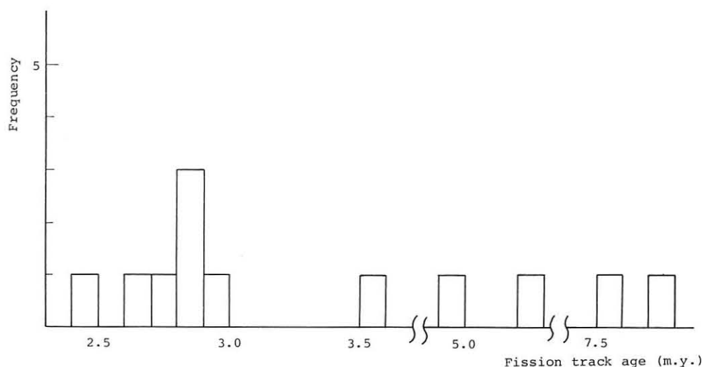
Text-fig. 4. Distribution of determined ages on 12 grains of zircon from the Sarubetsu pyroclastic flow deposits (see Table 2). Seven grains in the left hand corner of the figure will consist a normal population. See explanation of Text-fig. 3. for the equation to calculate a true fission track age.
