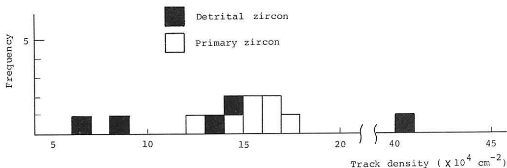
Text-fig. 7. Histogram of spontaneous fission track density of zircons from the Sarubetsu pyroclastic flow deposits.
