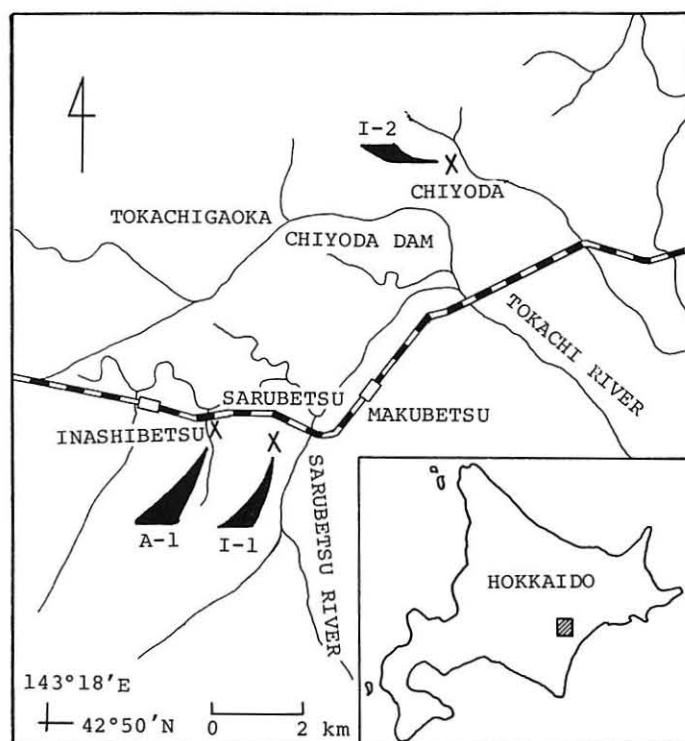
Text-fig. 1. Locality map of the studied area where the samples were collected for fission track dating.
