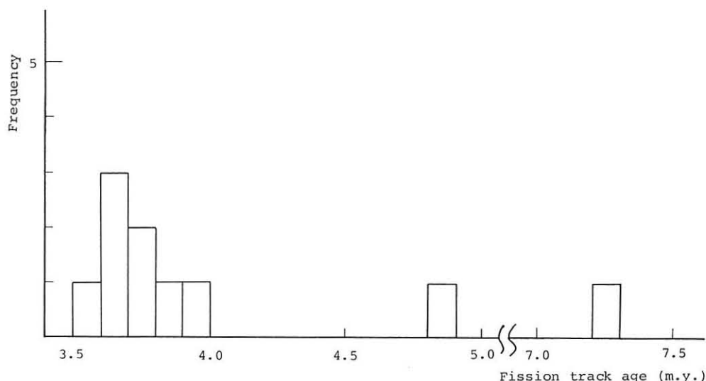
Text-fig. 3. Distribution of determined ages of 10 grains of zircon from the Inashibetsu pyroclastic flow deposits (see Table 1). Eight grains in the left hand corner of the figure will consist a normal population. A true fission track age is given by \bar{x} \pm t_{0.05} \frac{\hat{S}_x}{\sqrt{n}} where; \bar{x} : sample mean, \hat{S}_x^2 : sample variance, t_{0.05} : 5% point of t-distribution.
