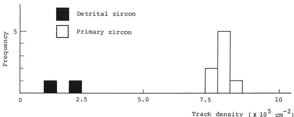
Text-fig. 6. Histogram of spontaneous fission track density of zircons from the Inashibetsu pyroclastic flow deposits.
