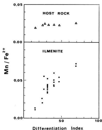
Text-fig. 3. The \text{Mn}/\text{Fe}^{2+} ratio vs. differentiation index for host rock and ilmenite.
