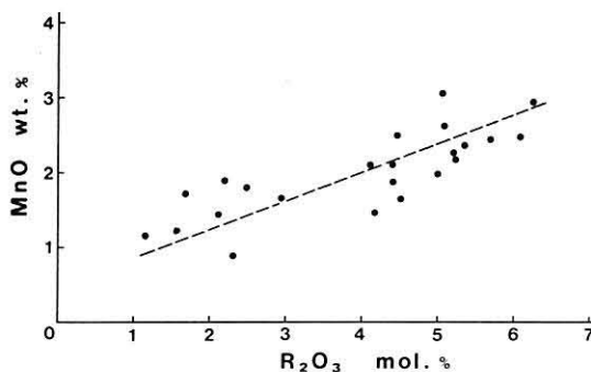
Text-fig. 4. Positive relation between MnO and \text{R}_2\text{O}_3 in ilmenite from Horoman.
