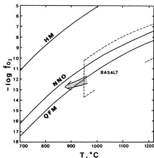
Text-fig. 5. Estimated course of crystallization of the Horoman diorite series. Field of basalt bounded by dashed lines is from Carmichael and Nicholls (1967). See the text in detail.
