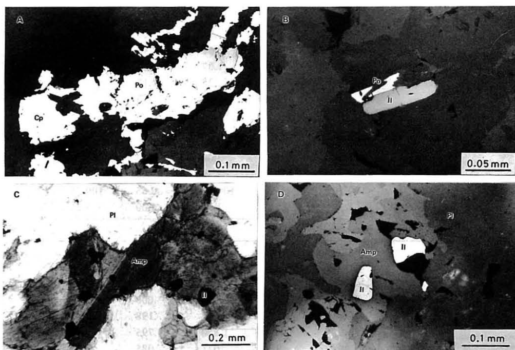
Text-fig. 2. Photomicrographs of the polished and thin sections illustrating the mode of occurrences of the ore minerals in the Horoman diorite.
