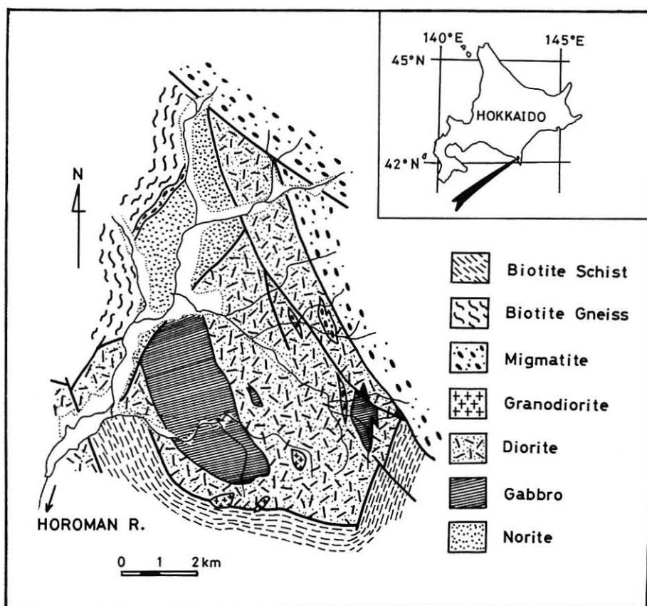
Text-fig. 1. Geological sketch map of the Horoman plutonic complex. The diorite series and the olivine gabbro series in the text are labeled 'Diorite' and 'Gabbro', respectively.
