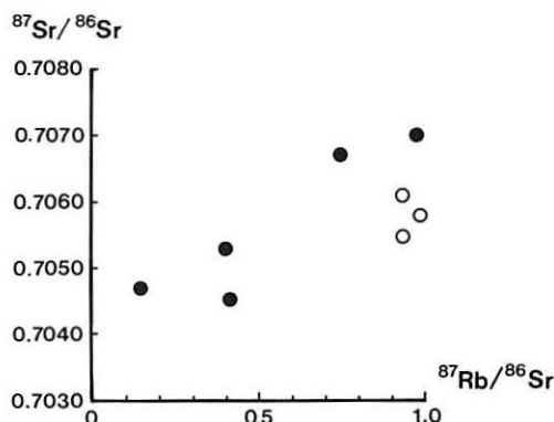
Text-figure 3 Recalculated initial ^{87}\text{Sr}/^{86}\text{Sr} ratios assuming the age of 115 Ma. solid circle: gabbroic body, and open circle: granodioritic body
