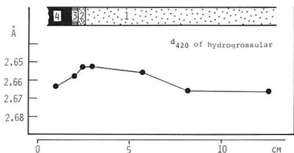
Text-fig. 12 Plots of d_{420} of hydrogrossular showing the variation in reaction zone (Sample No. 77721). Numbers 1 to 4: the reaction subzone Nos. 1 to 4 shown in Text-fig. 2.
