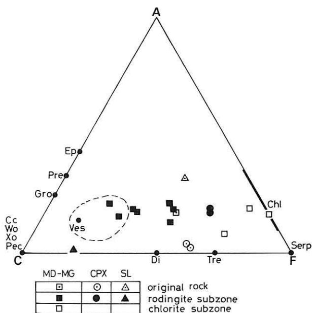
Text-fig. 6 ACF diagram showing the compositional variations of rodingites and their original rocks. The area limited by broken line shows the rodingite composition after Coleman (1977).
