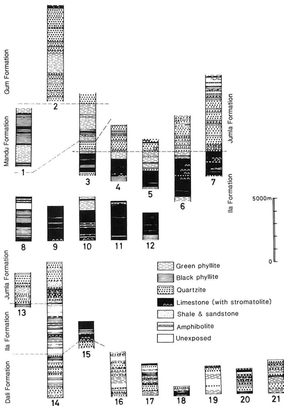
Text-fig. 3-b Lithostratigraphical columnar sections along mapped routes in the Midland meta-sediments zone. Figures under columns correspond to route numbers in Text-fig. 3-a.
