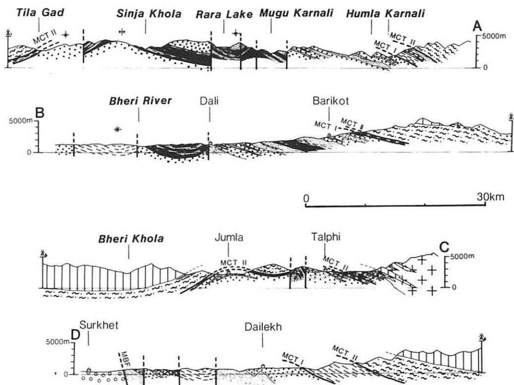
Text-fig. 4 Geological cross sections in western Nepal. Legends are the same as Text-fig. 2. MBF and MCT represent Main Boundary Fault and Main Central Thrust, respectively.
