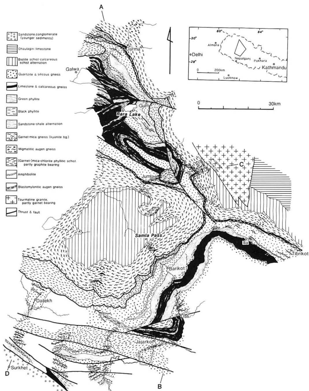
Text-fig. 2 Geological map of Surkhet-Jumla-Rara Lake region in western Nepal.
