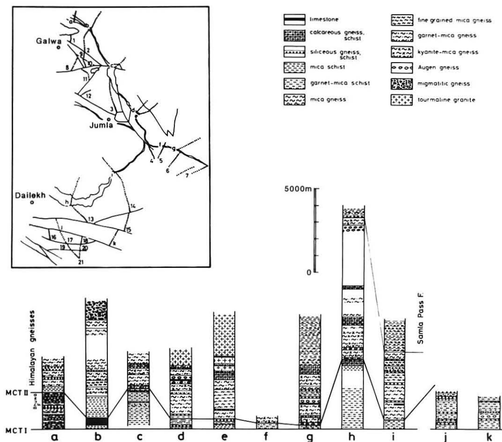
Text-fig. 3-a Lithostratigraphical columnar sections along mapped routes in the Himalayan gneiss and the Main Central Thrust zones. Dotted lines represent mapped routes. Alphabets under columns correspond to those of routes. MCT I and II represent the Main Central Thrust I and II, respectively. Figures of routes refer to Text-fig. 3-b.
