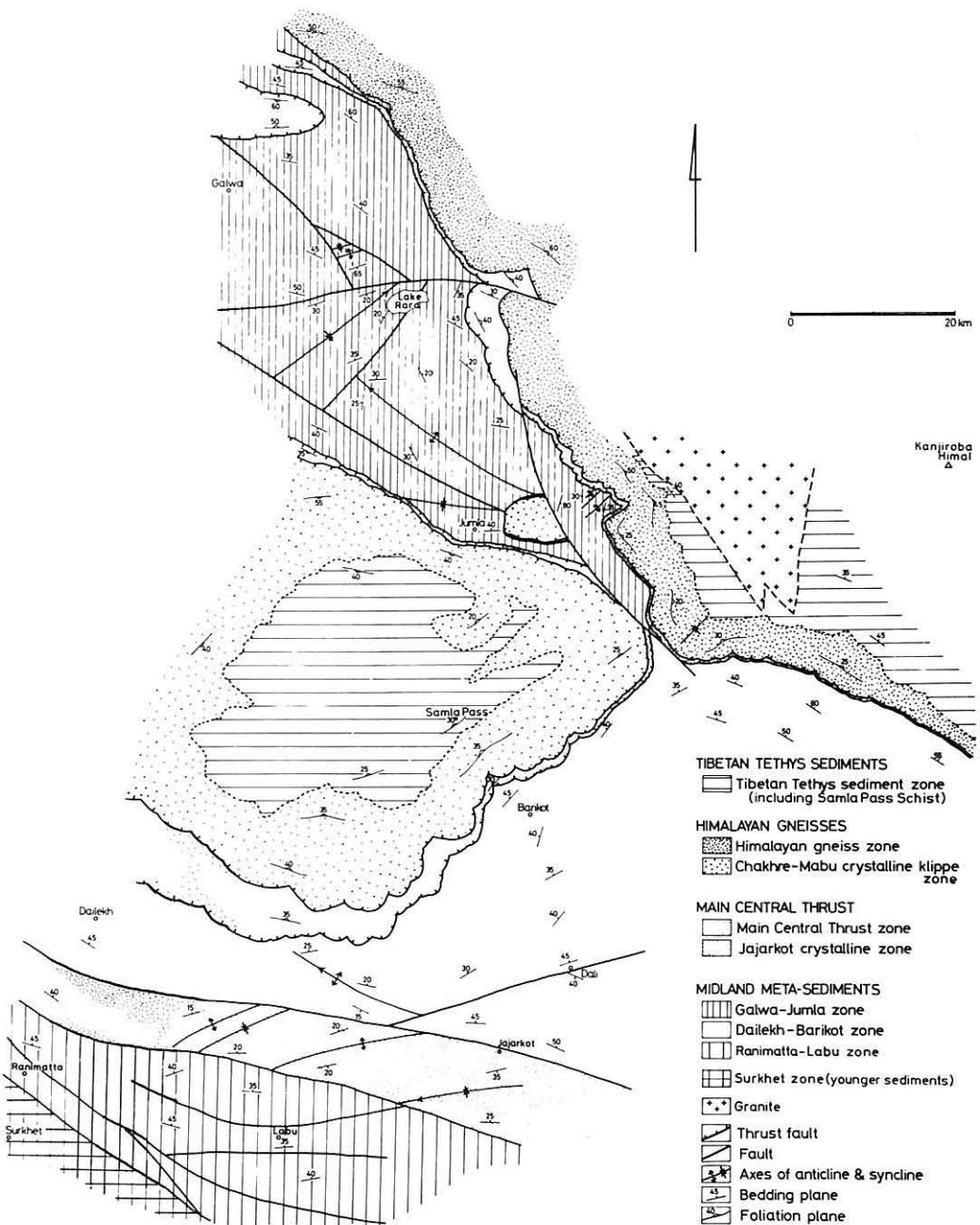
Text-fig. 1 Structural division and tectonic map of Surkhet-Jumla-Rara Lake region in western Nepal.
