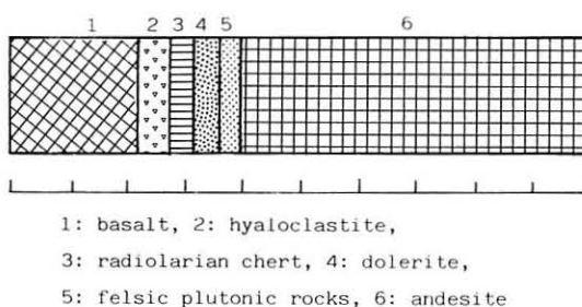
Text-fig. 8 Modal proportions of the constituent pebbles of the basal conglomerate of the Saroma Group in the northern Tokoro Belt (Narui, 1982).
