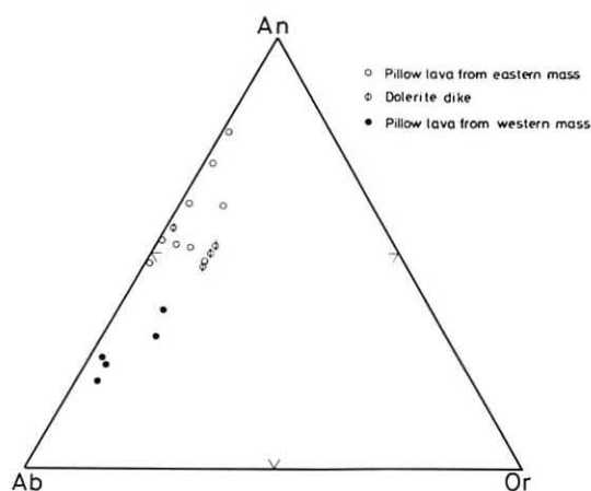
Text-fig. 6 An-Ab-Or diagram of the pillow basalts from the northern Tokoro Belt.
