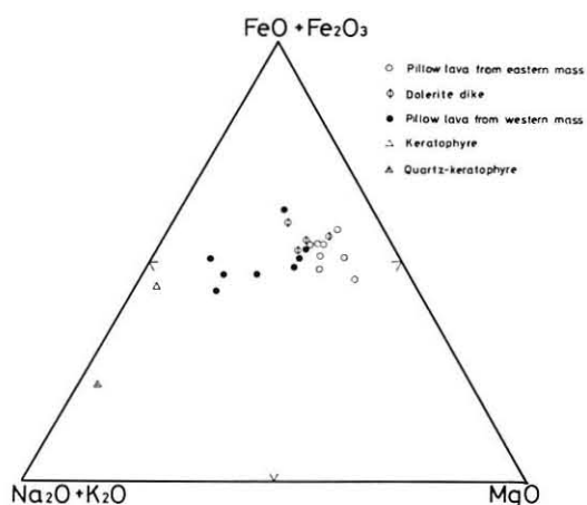
Text-fig. 7 AFM diagram of pillow basalts and related rocks from the northern Tokoro Belt.
