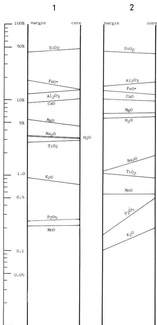
Text-fig. 4 Semilogarithmic plots of the chemical variations between the core and the rim of unit pillows of the pillow basalts from the northern Tokoro Belt.
