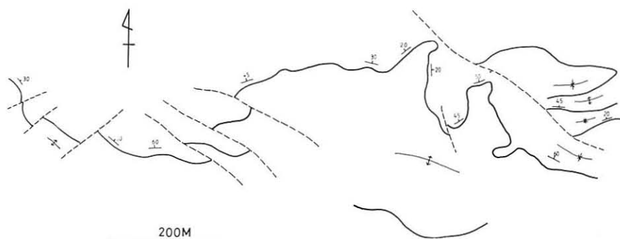
Text-fig. 10 Map showing the tectonic features of the manganiferous hematite ore bed in the Kokuriki mine. The left lateral offsets of the ore bed is observed. This tectonic pattern is a characteristic feature of the Eastern mass of the northern Tokoro Belt.
