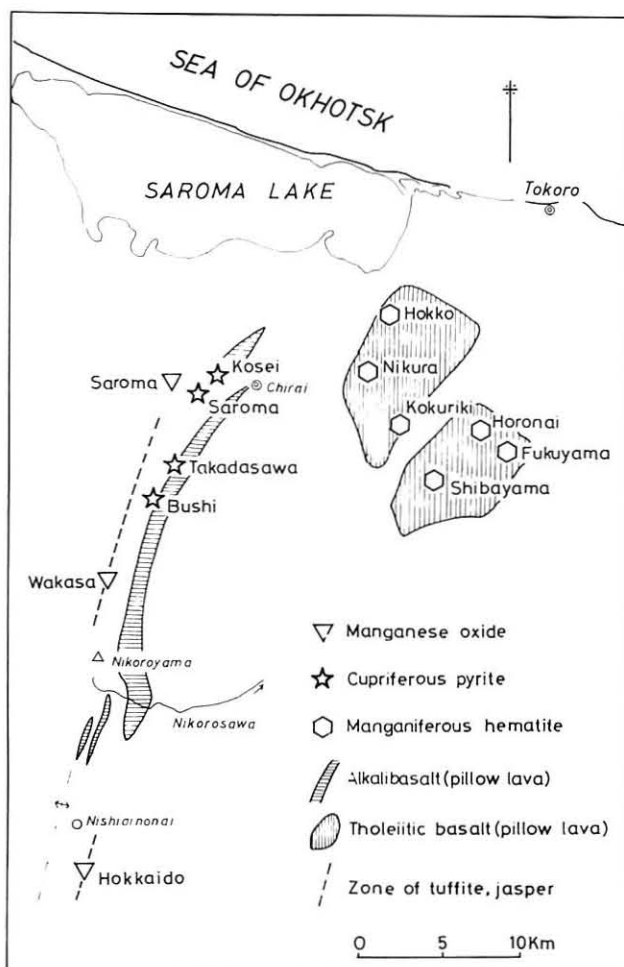
Text-fig. 12 Map showing the distributions of manganiferous hematite, massive sulfide and manganese oxide ore deposits and related volcanogenic rocks in the northern Tokoro Belt.
