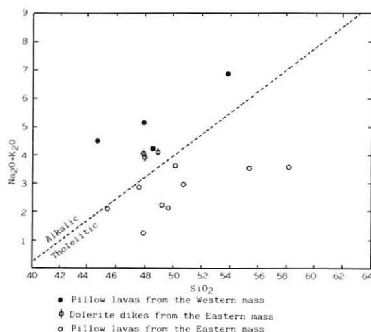
Text-fig. 5 Alkali-silica variations of pillow basalts and related rocks from the northern Tokoro Belt. All plotted in weight percent after subtracting total water and normalizing.
