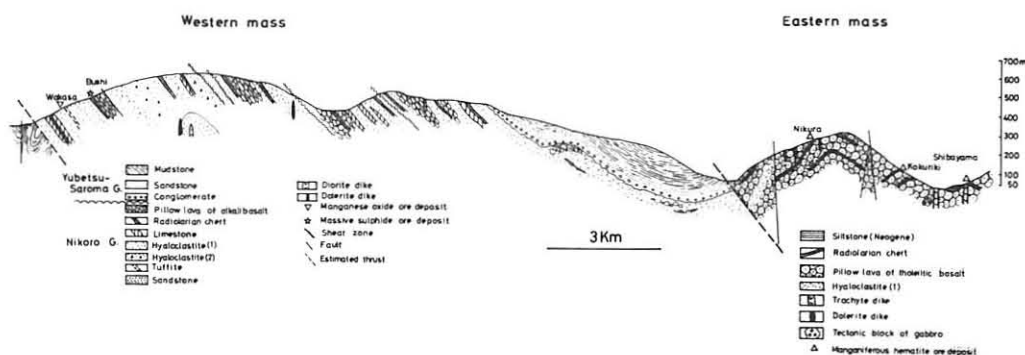
Text-fig. 2 Generalized geologic profile of the northern Tokoro Belt.
