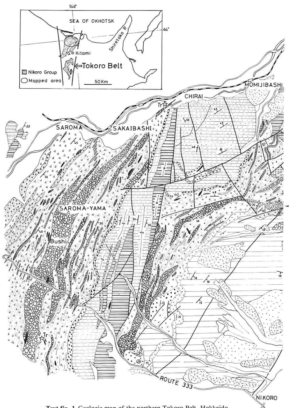
Text-fig. 1 Geologic map of the northern Tokoro Belt, Hokkaido.
