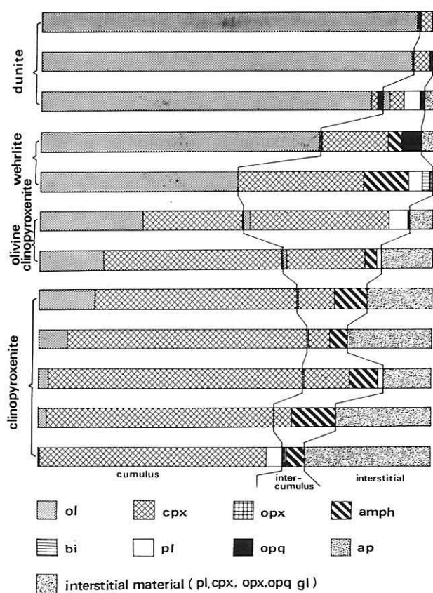
Text-fig. 3 Modal compositions of the ultramafic inclusions from Oshima-Ōshima.
