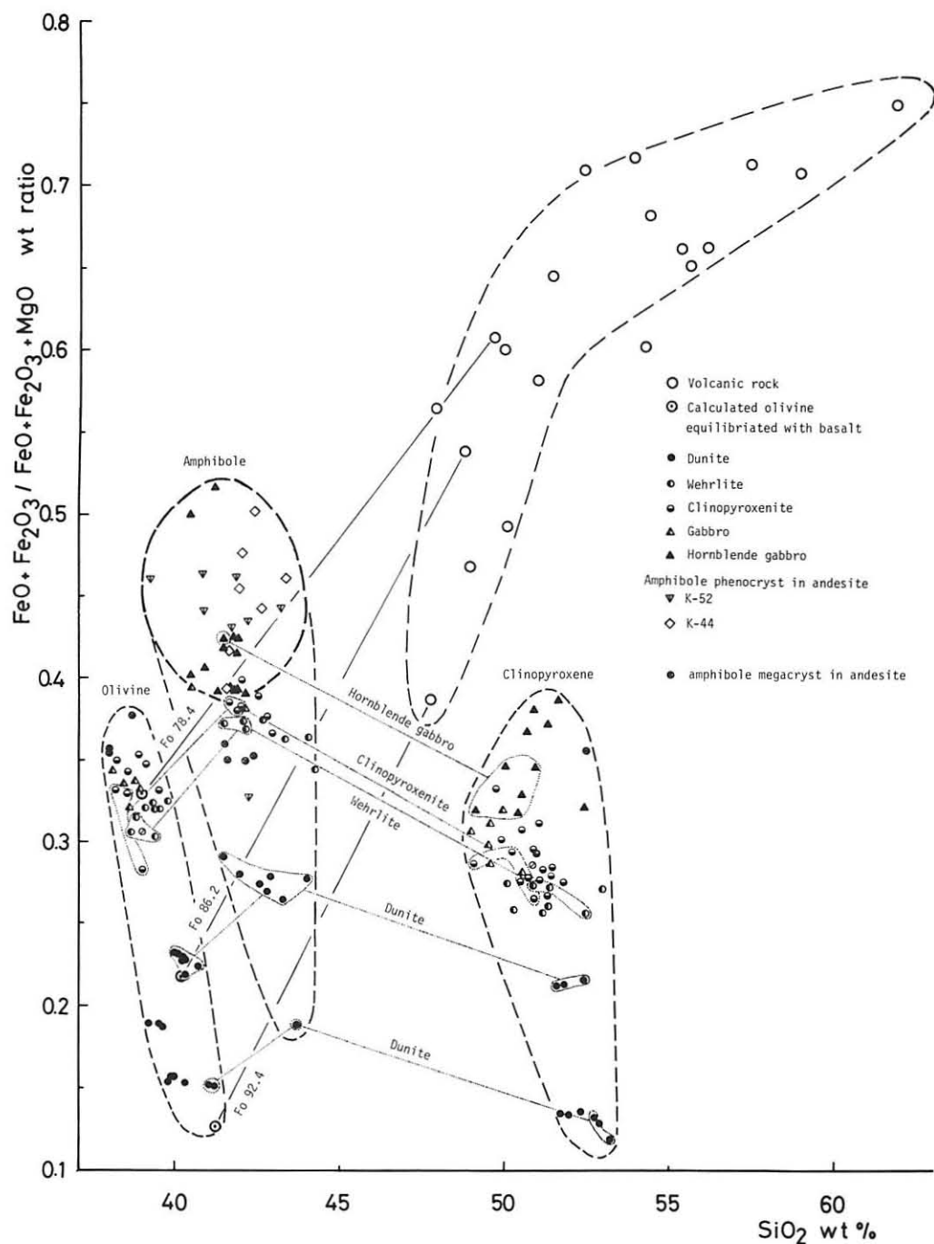
Text-fig. 32 \text{FeO} + \text{Fe}_2\text{O}_3 / \text{MgO} + \text{FeO} + \text{Fe}_2\text{O}_3 vs. \text{SiO}_2 diagram for basalt-andesite suite and minerals in the ultramafic & mafic inclusions from Oshima-Oshima. Dotted tie lines show the same specimens of the inclusions.
