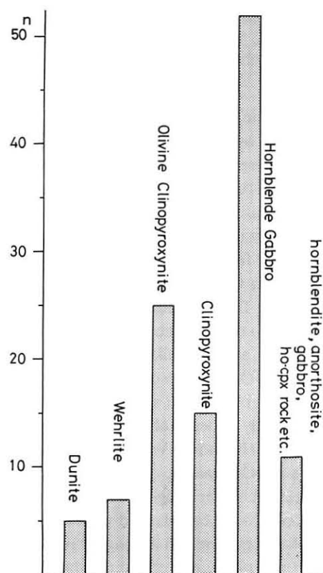
Text-fig. 5 Numbers of ultramafic and mafic inclusions found in the Nishi-yama middle lava at the coast of Aidomari, Oshima-Ōshima.
