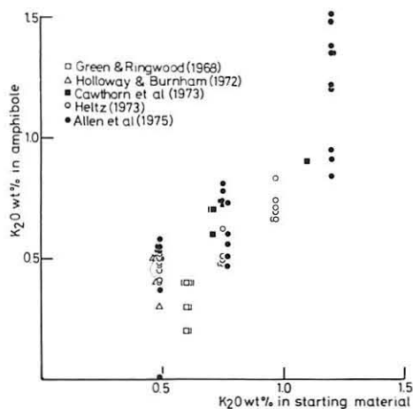
Text-fig. 17 Relation between K_2O contents of amphiboles and starting materials (natural basalts).
