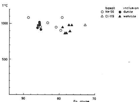
Text-fig. 31 Plot of calculated temperature by the method of Roeder et al. (1980) vs. Fo content of the olivine in contact with spinel.
