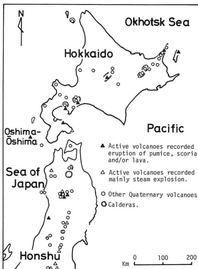
Text-fig. 1 Index map showing the location of Oshima-Ōshima Island.
