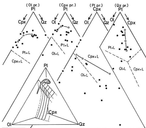
Text-fig. 23 Projection of data into the pseudo-quaternary system Ol-Cpx-Pl-Qz. Ol pr: projection from olivine, Cpx pr: projection from clinopyroxene, Pl pr: projection from plagioclase, and Qz pr: projection from quartz. The three open circles tied to each other are the pumice, felsic scoria and mafic scoria which were erupted successively in this order during 1741-1742 (Nishi-yama ejecta).
