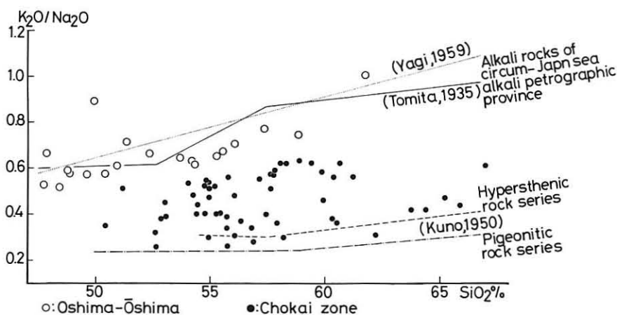
Text-fig. 7 \text{K}_2\text{O}/\text{Na}_2\text{O} vs. silica diagram for the rocks from Oshima-Ōshima and those from other volcanoes of Chōkai Volcanic Zone. The trend of principal volcanic rock series in Japan and surrounding areas are also shown (after Kuno, 1950; Tomita, 1935; Yagi, 1959).
