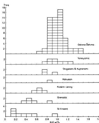
Text-fig. 15 K 2 O frequency-distribution for amphiboles associated with basic volcanic rocks.
