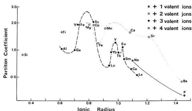
Text-fig. 21 Effective partition coefficient vs. ionic radius diagram determined by the calculation assuming Rayleigh fractionation from H_{20} to H_{21} . Ionic radii after Whittaker and Muntus (1970).
