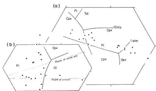
Text-fig. 24 Projection of data into phase diagram for anhydrous basalts (O'Hara, 1968).
