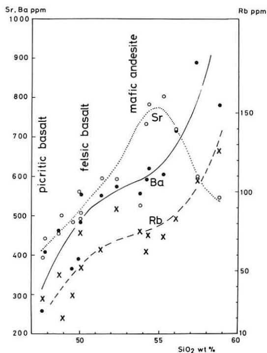
Text-fig. 11 Trends of Rb, Ba and Sr in the Oshima-Ōshima volcanic rocks.
