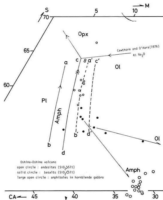
Text-fig. 25 Weight percent projection from diopside and alkali into part of the plane \text{CaAl}_2\text{O}_4\text{-MgO-SiO}_2 for the rocks from Oshima-Ōshima volcano.
