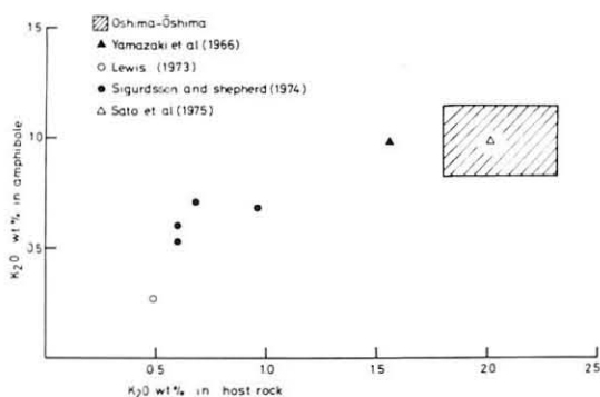
Text-fig. 16 Relation between K_2O contents in amphiboles and in host rocks. Plot of Oshima-Ōshima indicates ranges in amphiboles and rocks.
