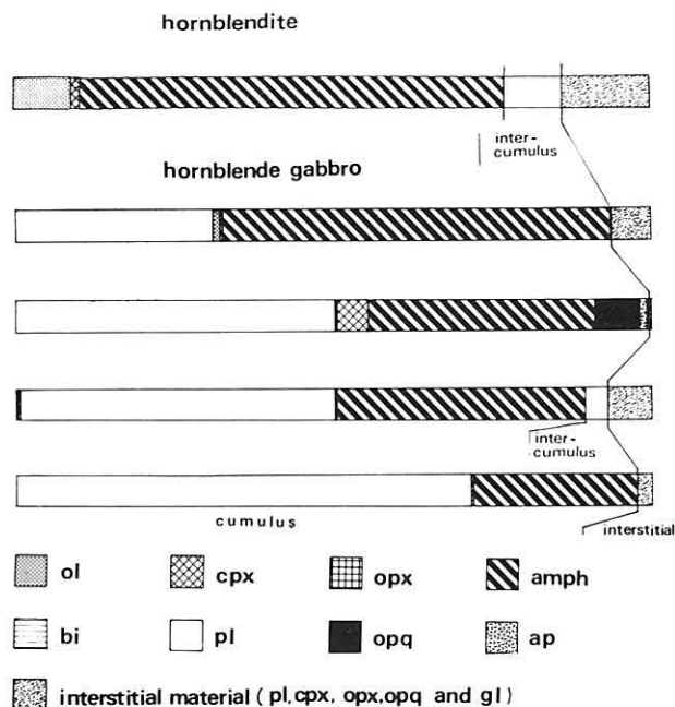
Text-fig. 4 Modal compositions of the mafic inclusions from Oshima-Oshima.
