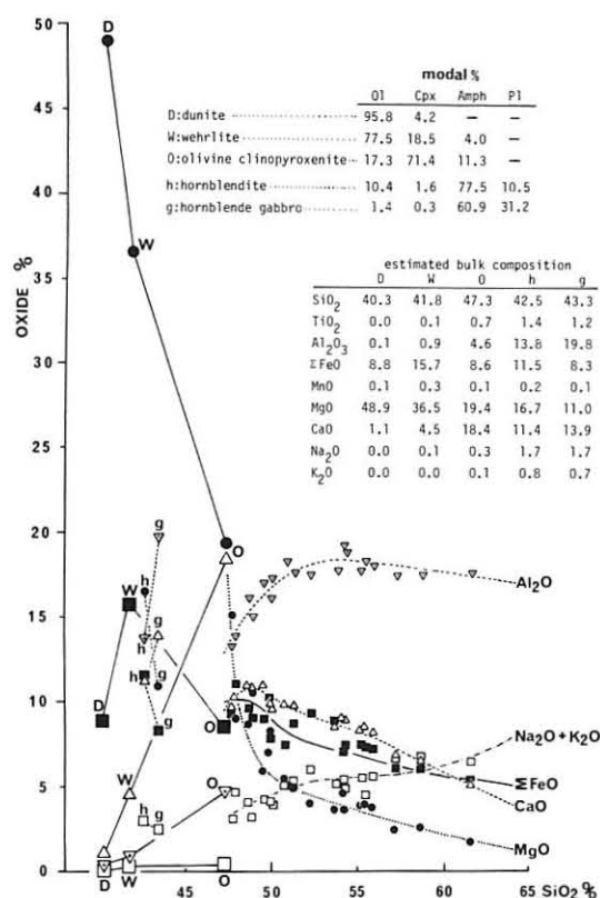
Text-fig. 19 Subtraction diagram for the Oshima-Ōshima rocks.
