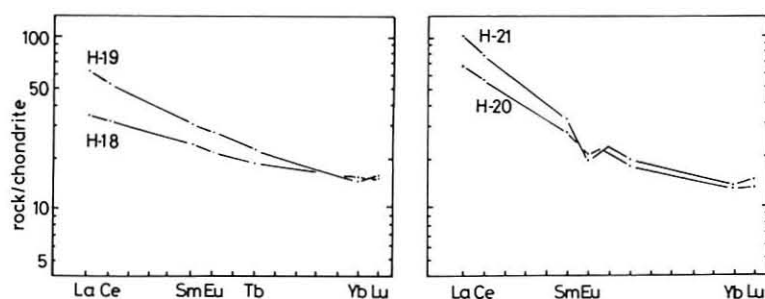
Text-fig. 10 Chondrite-normalized rare-earth elements pattern (Masuda et al., 1975).
