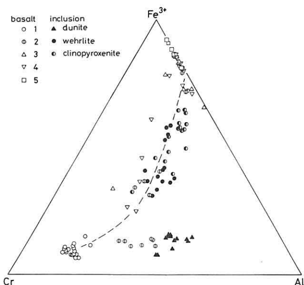
Text-fig. 28 Cr-Al- \text{Fe}^{3+} diagram of spinels.
