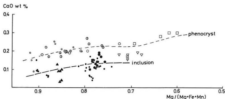
Text-fig. 29 CaO — Mg/(Mg + Fe + Mn) diagram for olivines. Symbols same as Text-fig. 28. large symbols indicate olivines in contact with spinels.
