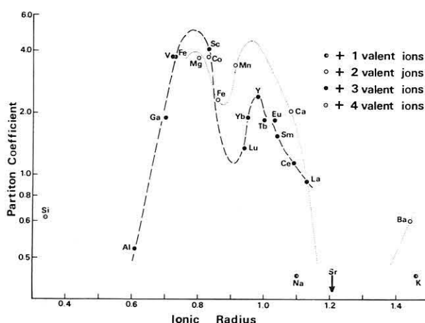
Text-fig. 22 Effective partition coefficient vs. ionic radius diagram of Dx.
