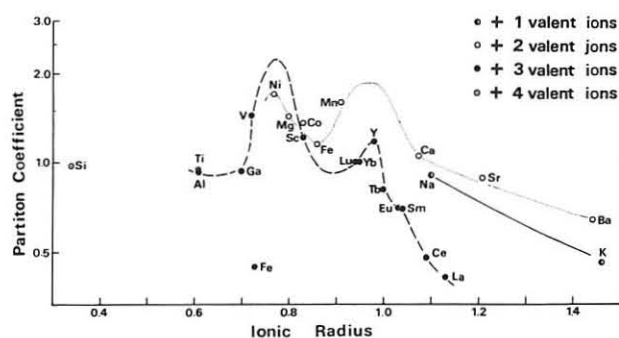
Text-fig. 20 Effective partition coefficient vs. ionic radius diagram determined by the calculation assuming Rayleigh fractionation from H_{18} to H_{19} . Ionic radii after Whittaker and Muntus (1970).
