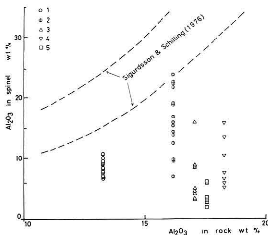
Text-fig. 27 Plot of \text{Al}_2\text{O}_3 content of spinels vs. \text{Al}_2\text{O}_3 content of whole rock. 1: augite-olivine basalt (Nu-104), 2: olivine-augite basalt (Ne-56), 3: olivine-augite basalt (Hu-100), 4: olivine-augite basalt (Cl-119), and 5: olivine-augite basaltic andesite (NI-11e).
