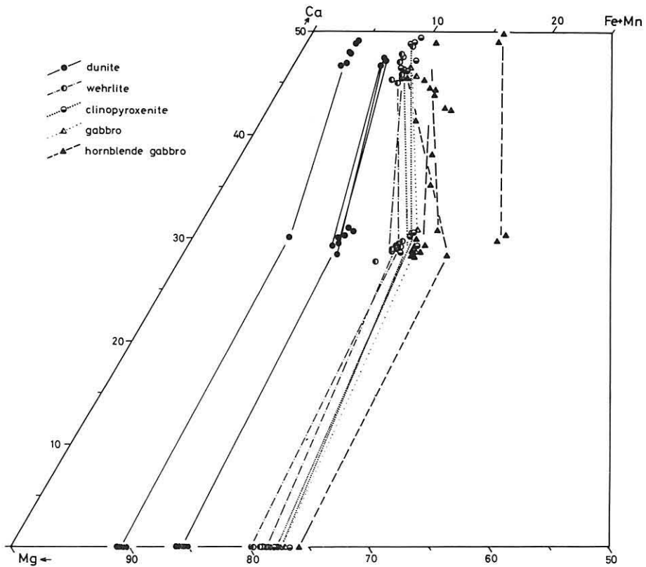
Text-fig. 12 Ca-Mg-Fe plot of clinopyroxenes, amphiboles and olivines (Ca free) from ultramafic and mafic inclusions. Tie-lines indicate minerals coexist each other.
