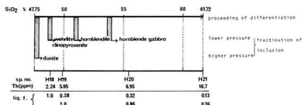
Text-fig. 33 Crystallization sequence of the basaltic-andesitic magma in Oshima-Ōshima. The Th content were determined by Masuda et al. (1975).
