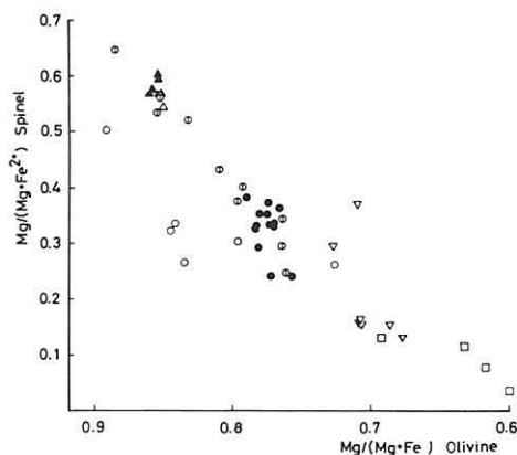
Text-fig. 30 Correlation between \text{Mg}/(\text{Mg} + \text{Fe}^{2+}) values of spinels and olivines in contact with each other. Symbols same as Text-fig. 28.
