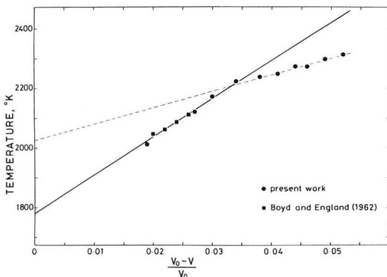
Text-fig. 5 Relation between the melting temperature and the volume change of pyrope. The solid line is illustrated by linear squares fitting of the present data below 70 kbar, and the dashed line is obtained by the fitting of the data at higher pressures.
