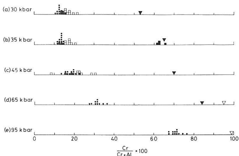
Text-fig. 3 Compositions of coexisting garnet and low pressure phases at 1200°C as a function of pressure. Circles and squares are results of EPMA analysis, and triangles are those based on lattice parameters. ●, garnet solid solution; □, orthopyroxene solid solution; ■, ▼, spinel solid solution; △, corundum solid solution.
