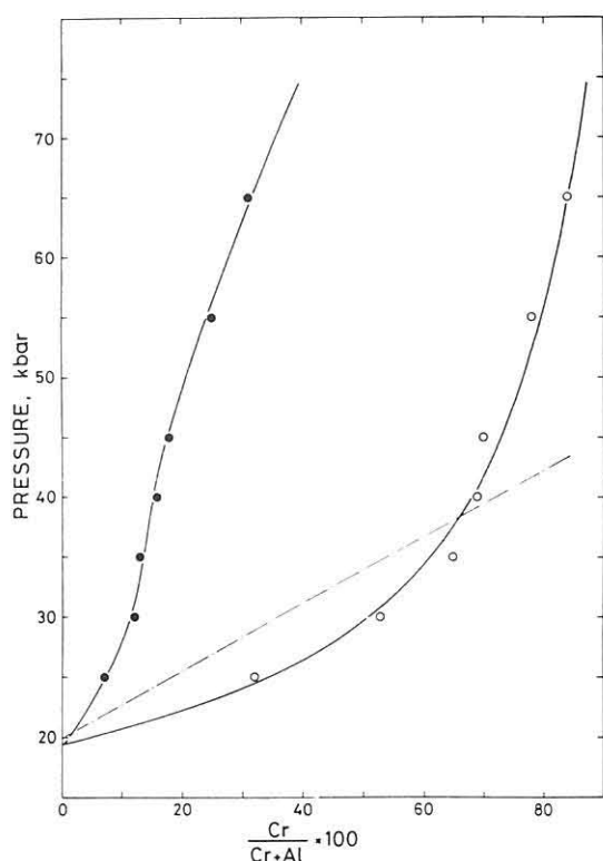
Text-fig. 10 Chemical compositions of coexisting spinel and garnet solid solutions at various pressures at 1200°C. Open circles are the results for the spinel, and closed ones are those for the garnet. The solid lines are to guide the reader's eye. The chain line is illustrated on the basis of the results for the spinel in CMAS- \text{Cr}_2\text{O}_3 system by O'Neill (1981).
