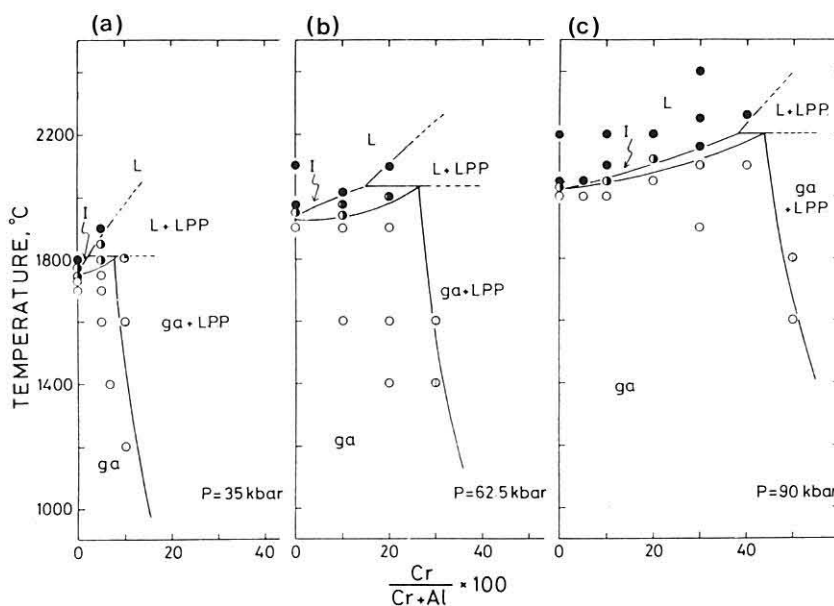
Text-fig. 6 Melting relation of garnet solid solution between pyrope and knorringite at (a) 35 kbar, (b) 62.5 kbar, and (c) 90 kbar. "I" indicates the field of garnet solid solution + liquid. L, liquid; ga, garnet solid solution; L.P.P., low pressure phases.
