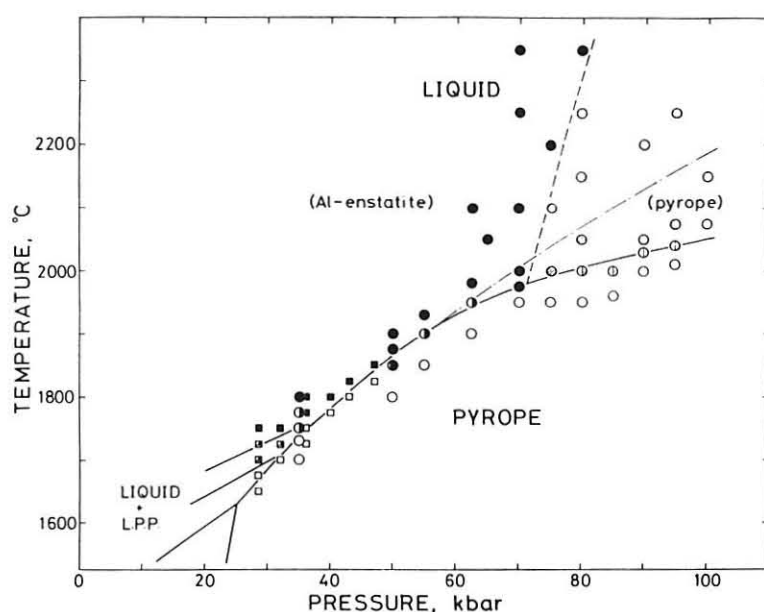
Text-fig. 4 Melting relation of pyrope up to 100 kbar. The dashed line indicates the apparent boundary between two quench crystals, aluminous enstatite and pyrope. The chain line is an extrapolated melting curve by the Kraut-Kennedy equation (see, text). Circles are the results of the present study, and squares are those by Boyd and England (1964).
