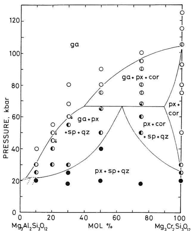
Text-fig. 2 Subsolidus phase relation between pyrope and knorringite at 1200°C (after Irifune and Hariya, 1983).
