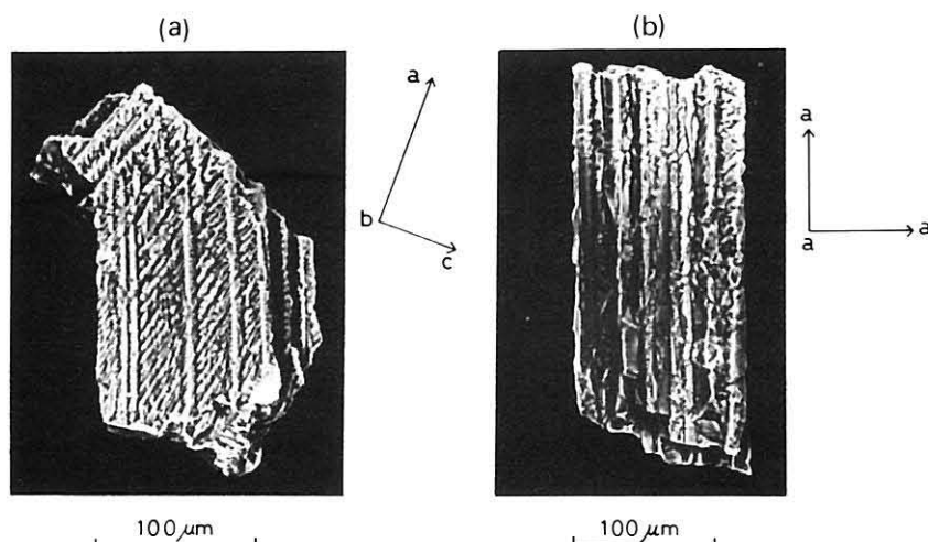
Text-fig. 7 SEM images of quench crystals from pyrope melt. (a) aluminous enstatite: The elongated direction of the lamellae disagrees with any axes; the included angle is 69.3^\circ \pm 0.5^\circ . (b) pyrope: The crystal elongates in parallel with the a-axis.
