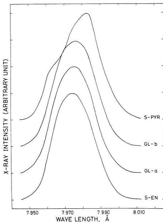
Text-fig. 9 Comparison of Al K\beta bands between pyrope glasses and synthetic crystals. The profile of Al K\beta band was illustrated on the basis of the results of curve fitting shown in Text-fig. 8.
