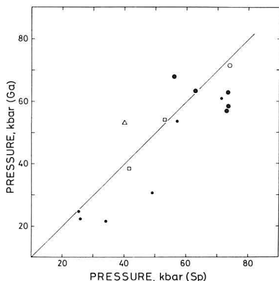
Text-fig. 11 Correlation between the equilibrium pressures obtained by the spinel and the garnet geobarometers (see, text). Data source: Sobolev (1974). ○, from diamond; ●, from peridotite; ●, from garnet-pyroxene-chromite intergrowth; □, from porphyritic peridotites of the Udachnaya pipe; △, from pyrope peridotite of metamorphic complex.
