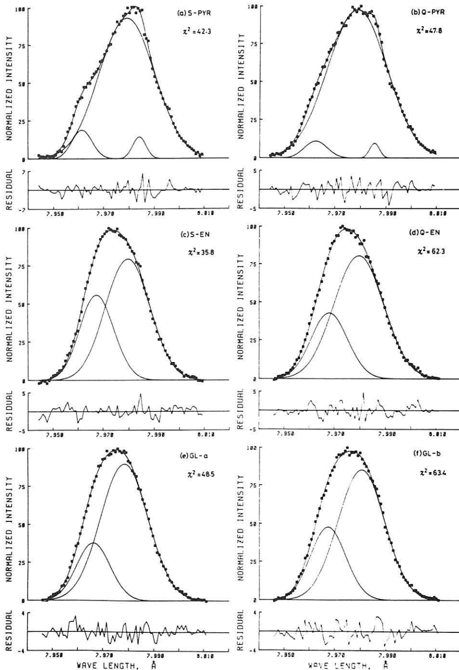
Text-fig. 8 Results of deconvolution for Al K\beta bands of synthetic and quench phases. (a) synthetic pyrope; (b) quench pyrope; (c) Synthetic aluminous enstatite; (d) quench aluminous enstatite; (e) pyrope glass obtained at 35 kbar; (f) pyrope glass obtained at 55 kbar.
