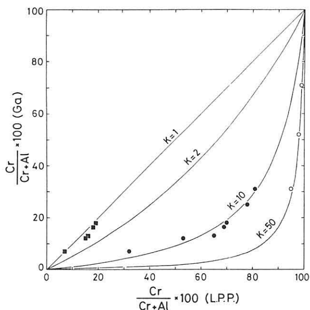
Text-fig. 13 Distribution features of Cr and Al between garnet and other low pressure phases (L.P.P.). K denotes the apparent partition coefficient. Data are those obtained in the present experiment for the pyrope-knorringite system. ●, garnet-spinel; ■, garnet-orthopyroxene; ○, garnet-corundum.
