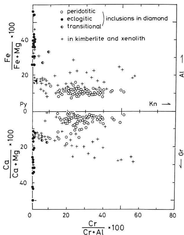
Text-fig. 12 Compositions of garnet inclusions in diamonds and those from kimberlites and associated xenoliths (after Irifune et al., 1982). Py, pyrope; Kn, khorringite; Al, almandine; Gr, grossular.
