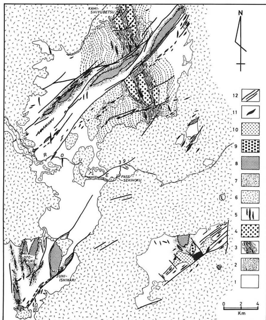
Text-fig. 1 Structural map in the vicinity of the OKETO RHYOLITE mass (showing both of the Shirataki structural line and the Kamishiyubetsu structural one).
