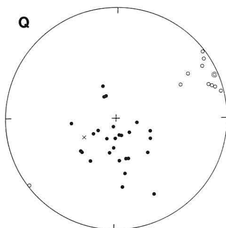
Text-fig. 9 Schmidt net (lower hemisphere) plots for clast long axes and ab-plane poles.
