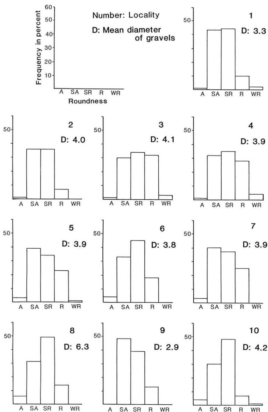
Text-fig. 5 Mean diameter of gravels (cm) and the frequency distribution of roundness grades.
