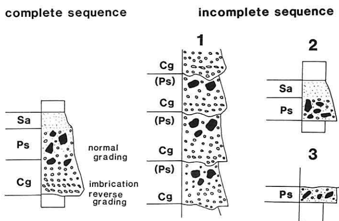
Text-fig. 3 Types of the sequence of coarse clastic bed (after Hoyanagi & Ohkami, 1986).
