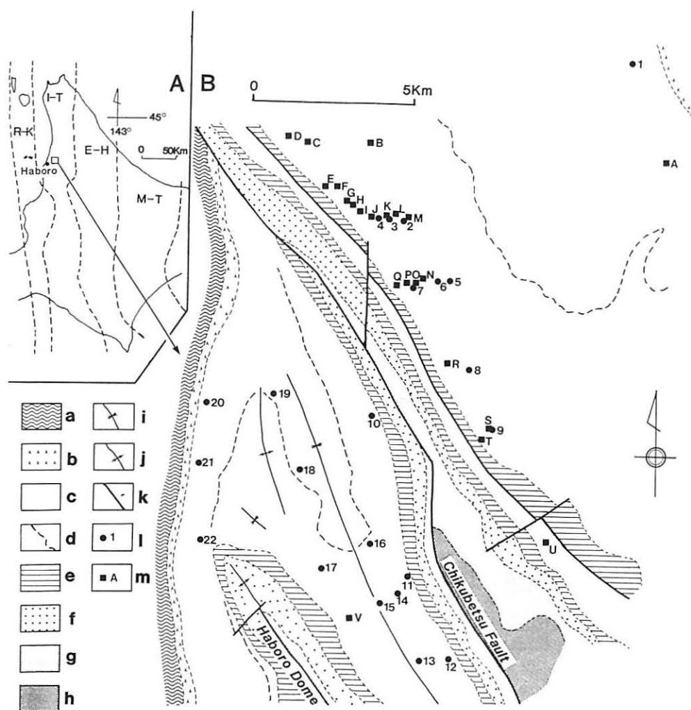
Text-fig. 1 A; Geotectonic division of central Hokkaido in the Miocene (after Hoyaagi et al., 1986).
