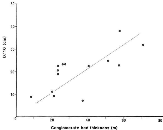
Text-fig. 4 Graph of coarse clastic bed thickness versus mean of the ten largest clasts ( D/10 ).
