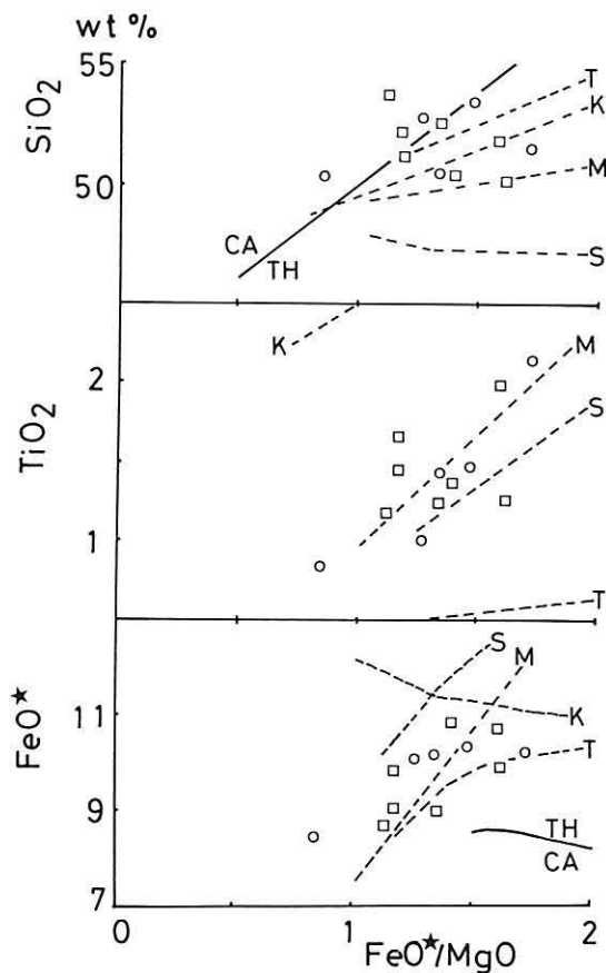
Text-fig. 5 \text{SiO}_2 , \text{TiO}_2 and \text{FeO}^* versus \text{FeO}^*/\text{MgO} diagrams
