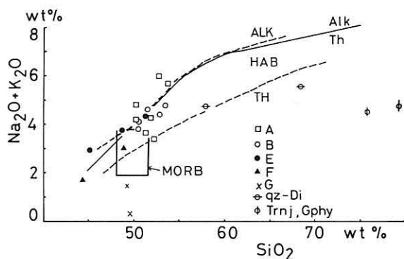
Text-fig. 3 Na 2 O+K 2 O — SiO 2 diagram. Solid line is the boundary between the alkaline (Alk) and tholeiitic (Th) rock suites (Macdonald and Katsura, 1964). Broken lines are the boundaries among the alkali (ALK), high-alumina basalt (HAB) and tholeiite (TH) rock series (Kuno, 1966). Rectangular field represents MORB (Miyashiro, 1973). Symbols with A to G: ultramafic and mafic rocks of the metamorphic zones A to G. qz-Di: quartz diorite, Trnj: trondhjemite, Gphy: granophyre.
