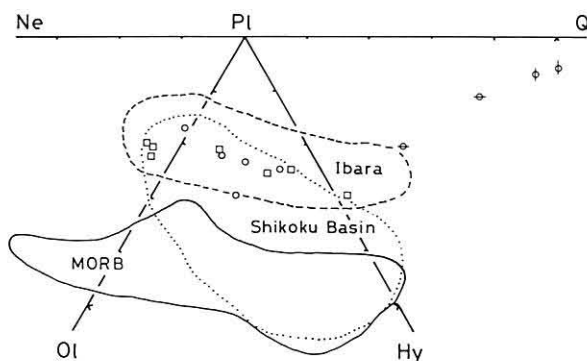
Text-fig. 4 Ne-Pl-Ol-Hy-Q diagram of C.I.P.W. norm
