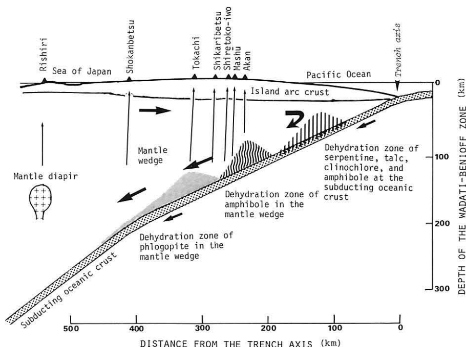
Text-fig. 6 Cartoon to illustrate arc magmatism and subducting oceanic crust across the Kurile arc. Arrows in the mantle wedge indicate the convective current.
