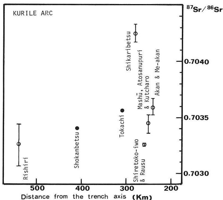
Text-fig. 2 Variations in ^{87}\text{Sr}/^{86}\text{Sr} ratios of Quaternary volcanic rocks across the Kurile arc. Open circles: mean values.
