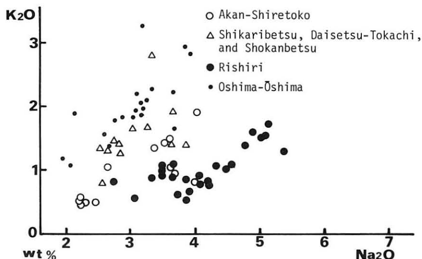
Text-fig. 5 K 2 O vs. Na 2 O diagram for Quaternary volcanic rocks from Hokkaido (data from Katsui, 1953; Matsui et al., 1967; Katsui et al., 1978; Yamamoto, 1984).
