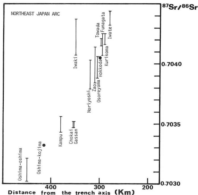
Text-fig. 3 Variations in ^{87}\text{Sr}/^{86}\text{Sr} ratios of Quaternary volcanic rocks across the Northeast Japan arc (data from Notsu, 1983; H. Kurasawa, unpublished data, Oshima-Ōshima, ^{87}\text{Sr}/^{86}\text{Sr} = 0.70302 — 0.70321, Oshima-Kojima, ^{87}\text{Sr}/^{86}\text{Sr} = 0.70332).
