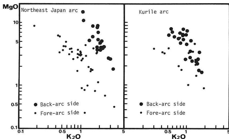
Text-fig. 4 MgO vs. \text{K}_2\text{O} log-log diagram for Quaternary volcanic rocks from the Northeast Japan and Kurile arcs in Hokkaido (data from Katsui, 1953; Matsui et al., 1967; Katsui et al., 1978; Yamamoto, 1984).
