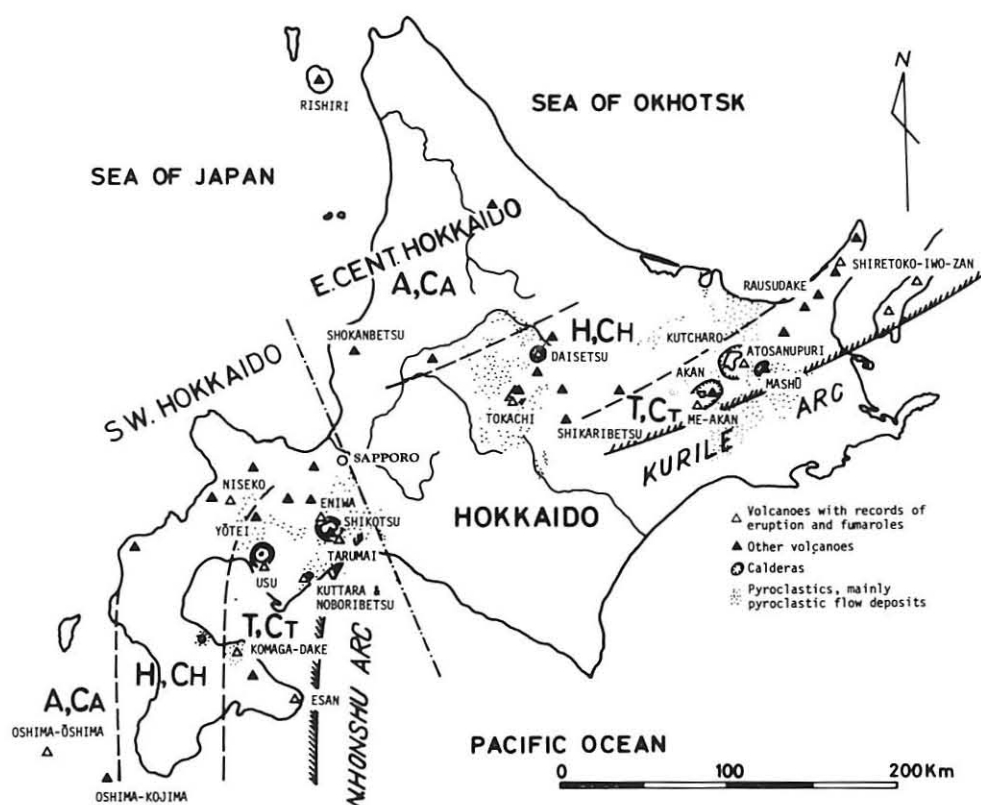
Text-fig. 1 Distribution of Quaternary volcanoes in Hokkaido (after Katsui et al., 1978). Petrographic provinces are shown by the symbols of rock series as follows: T (tholeiite basalt) & C_T (calc-alkali rock associated with T), H (high-alumina basalt) & CH (calc-alkali rock associated with H), and A (alkali basalt) & CA (calc-alkali rock associated with A).
