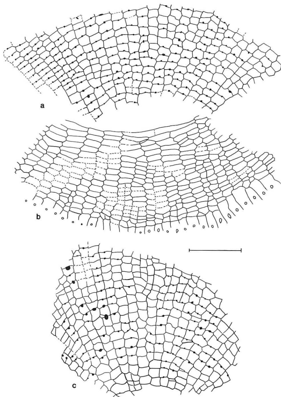
Text-fig. 1 Brachial plate arrangement of Pernerocrinus hayasakai (Minato and Minoura) (scale-bar is 10 mm).
