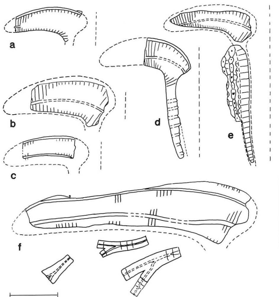
Text-fig. 4 Reconstructed vertical cross section of the Japanese Pernerocrinus . Broken lines are estimated portion and probable center of each specimen. (scale-bar is 20 mm) a: P. hayasakai based on Paratype UHR 30189. b: P. hayasakai based on UHR 30669. c: P. hayasakai based on UHR 30672. d: P. hayasakai based on UHR 30668. e: P. perforatus based on Holotype UHR 30671. f: P. sp. based on UHR 30670.
