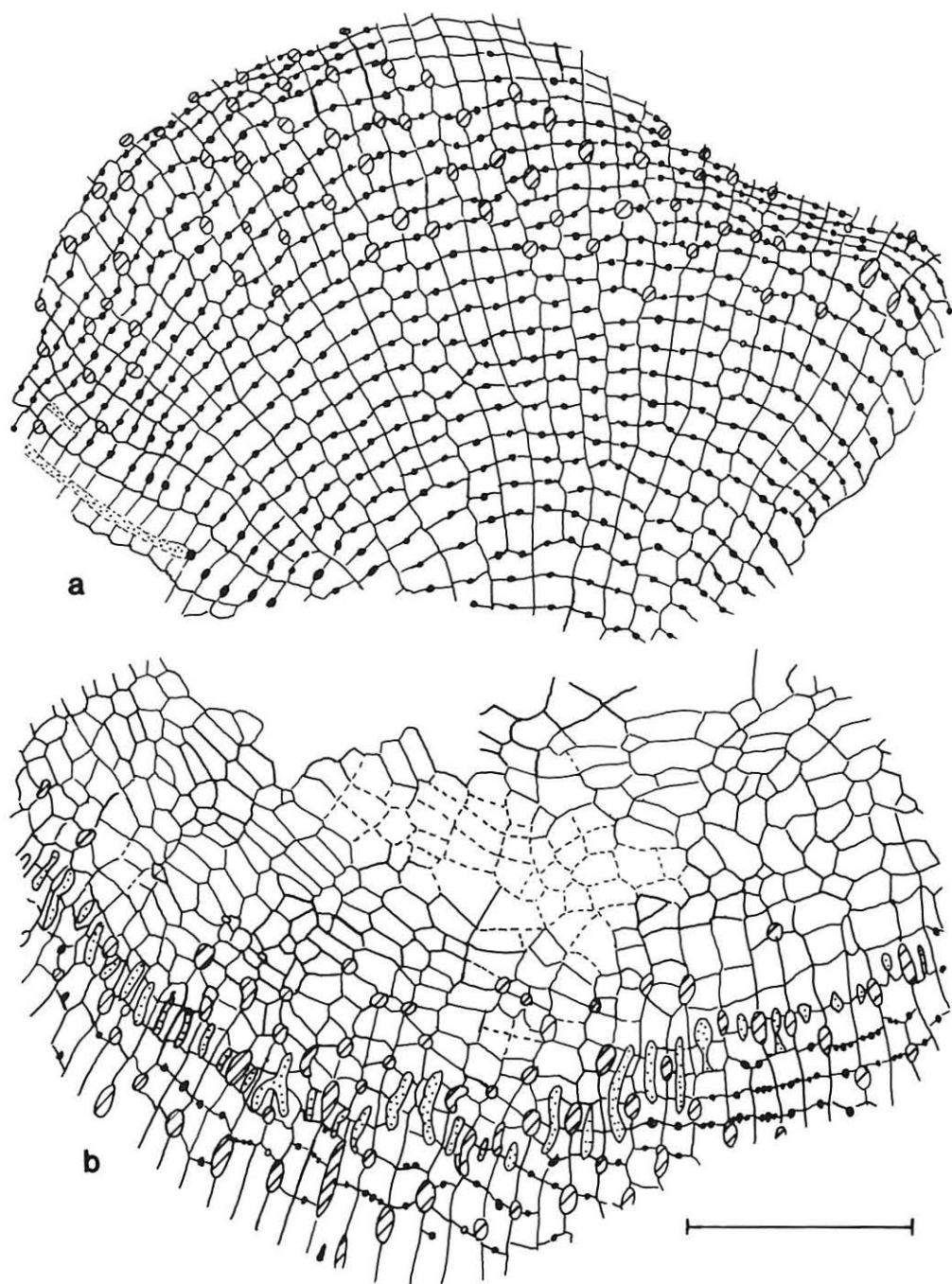
Text-fig. 2 Brachial plate arrangement of Pernerocrinus perforatus sp. nov. (scale-bar is 10 mm). a: ventral side drawn from photo shown as plate 2, fig. 1a. b: dorsal side from plate 2, fig. 1b. Axial canals are stippled and interarticular canals are diagonally ruled.
