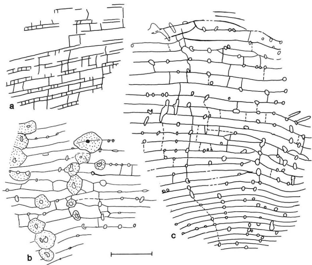
Text-fig. 3 Sketch showing the plate arrangement of column. (scale-bar is ca. 10 mm) a: internal surface of the lumen of Pernerocrinus hayasakai (Minato and Minoura) drawn from photo shown as plate 3, fig. 1a. b: Weathered external surface of column of Pernerocrinus perforatus sp. nov. from plate 2, fig. 3b. c: internal surface of the lumen of Pernerocrinus perforatus sp. nov. from plate 2, figs 3a, b.
