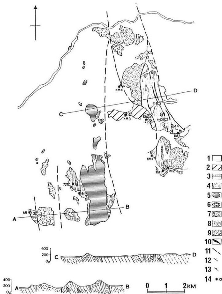
Text-fig. 5 Geological map of Sakuraoka — Toma region.
