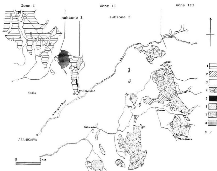
Text-fig. 2 Simplified geological map of the studied region.
