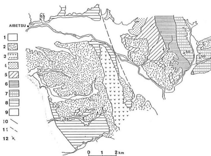
Text-fig. 8 Geological map of the Aibetsu area (referred from Kato & Iwata, 1987).
