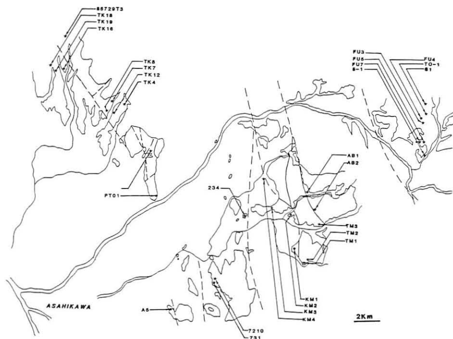
Text-fig. 7 Locality map of radiolarians in the studied region.
