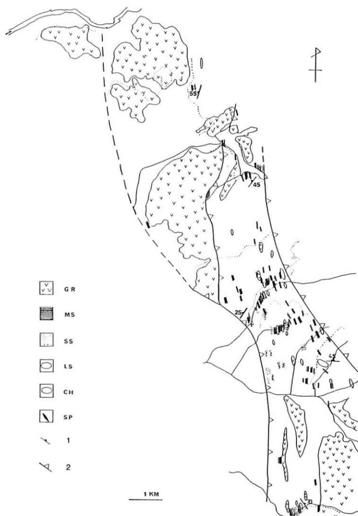
Text-fig. 6 Lithological map within the Toma Formation of the Kaimei — Todoyama region. GR: greenstones, MS: mudstone, SS: sandstone, LS: limestone, CH: chert, SP: serpentine, 1 : foliation, 2 : thrust.
