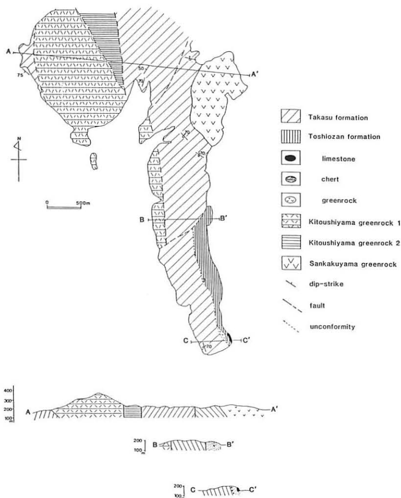
Text-fig. 4 Geological map of the Pippu region.
