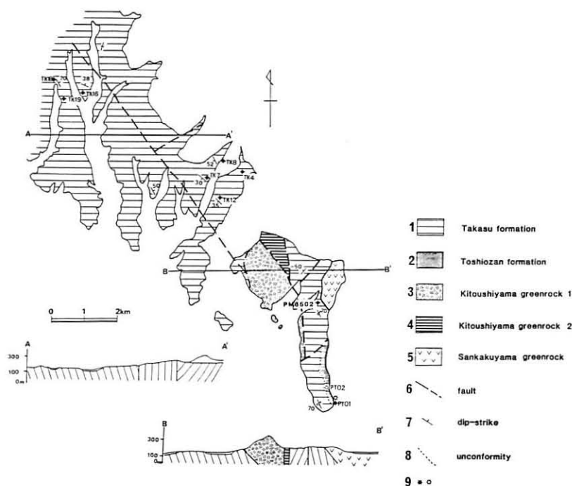
Text-fig. 3 Simplified geological map of the Takasu — Pippu area. Black circles showing localities of radiolarian fossils from shale. Open circles showing locations of radiolarians from chert blocks.
