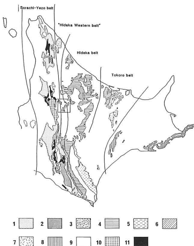
Text-fig. 1 Distribution of the Mesozoic Systems in the Axial zone of Hokkaido and the structural subdivision. A rectangle space showing the studied area.
