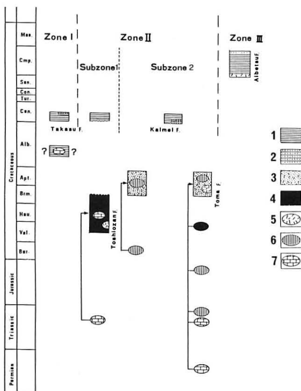
Text-fig. 9 Revised stratigraphy of the pre-Tertiary System in the Pippu-Toma region. Encircled symbols show exotic blocks.
