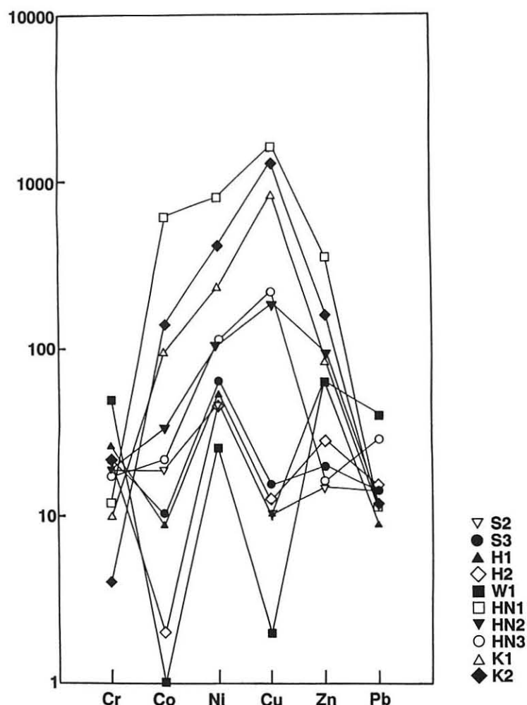
Text-Fig. 3 Representative trace element profiles for manganese ores from the Tokoro Belt. Samples from the Hinode and the Koryu mines have rather higher chemical composition than those of the Syototsibetu, the Hokkaido, and the Wakasa mines. S: Syototsibetu mine H: Hokkaido mine W: Wakasa mine HN: Hinode mine K: Koryu mine
