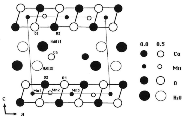
Text-fig. 4 Projection down b of todorokite crystal structure. The light line show the unit cell. In this model, the occupancy of H 2 O[1], H 2 O[2] and Ca are 0.5, 0.5 and 0.4, respectively.
