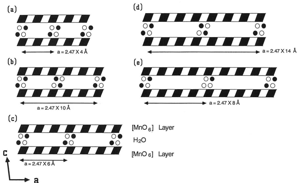
Text-fig. 5 Schematic diagrams of layer structure models. The line below each model indicates the length of a-axis.
