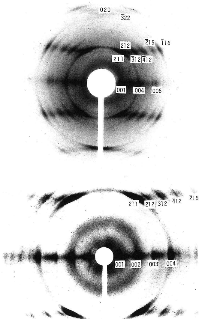
Text-fig. 2 X-ray diffraction photograph of todorokite from the Todoroki mine.
