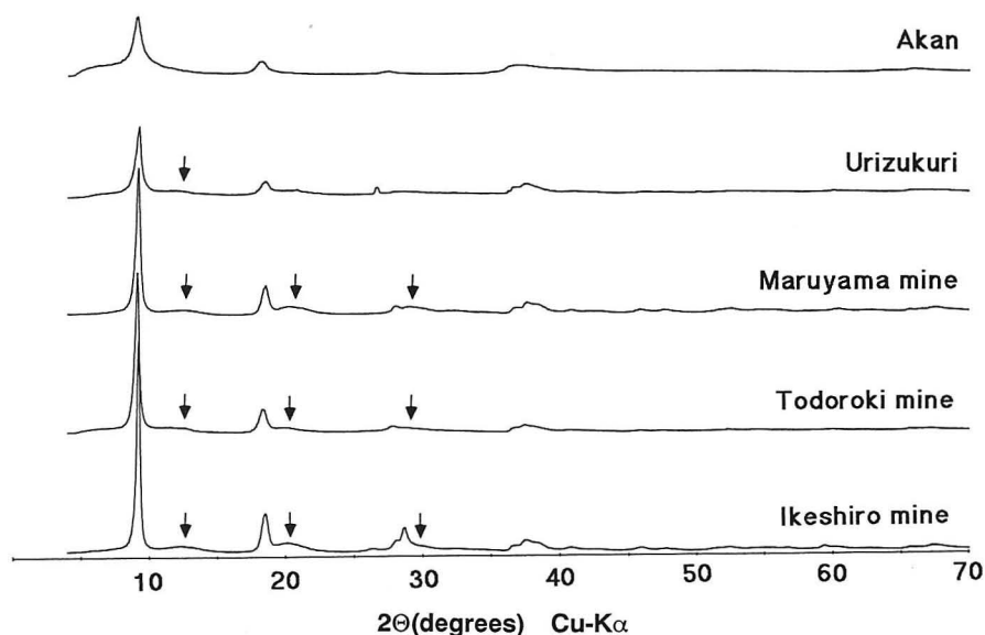
Text-fig. 1 X-ray powder diffraction profiles of todorokites from Japan. Arrows locate weak and broad diffraction peaks. Experimental conditions: Radiation: \text{Cu-K}\alpha , 35 Kv, 20 mA; Monochromator: graphite; Scanning method: step scanning; step size: 0.05^\circ ; Counting time: 30 sec.
