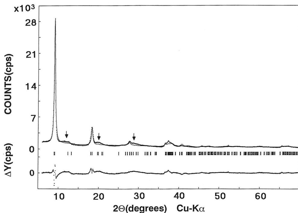
Text-fig. 3 Observed and calculated diffraction profiles of todorokite from Todoroki mine. The dots are observed data and solid lines are calculated profiles. The vertical bar-marks indicate the positions of the calculated diffraction peaks. The difference between the observed and the calculated data ( \Delta Y ) is plotted below the vertical bar-marks. Arrows locate the observed weak and broad diffraction peaks derived from the disorder toward a or c direction.
