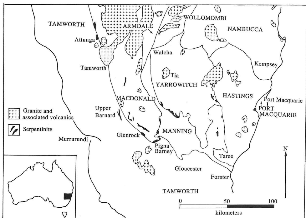
Text-fig. 1 Paleozoic structural blocks of the southern New England Fold Belt (modified from Leitch et al., 1990)
