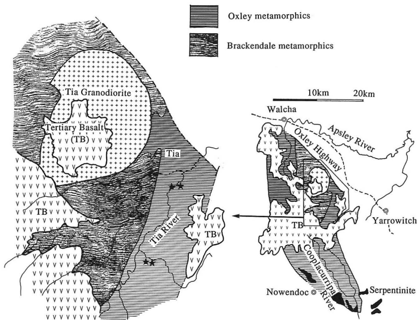
Text-fig. 2 Distribution of the Oxley and Brakendale metamorphics in the Tia area (after Gunthorpe, 1970) and localities of sheath folds (star symbols).
