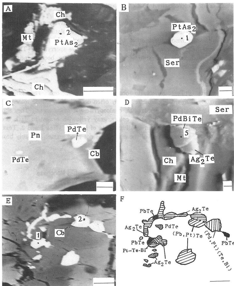
Text-fig. 1 Back-scattered electron images (A, B, C, D and E) of PGM and sketch map (F). A and B: different occurrence of sperrylites (PtAs 2 ); C: merenskyite (PdTe 2 ) occurred in the pentlandite; D: michenerite (PdBiTe) and hessite (Ag 2 Te) occurred in margin of the chalcopyrite; E and F: PGM occurred in sulfide and its sketch map. Scale bar: 10 \mu\text{m} . Abbreviations: Cb=Cubanite; Mt=Magnetite; Pn=Pentlandite; Ch=Chalcopyrite; Ser=Serpentine. See Table 1 for Nos. 1 in B & 2 in A; Tables 2 & 4 for Nos. 1 & 2 in E, respectively; Table 3 for 5 in D.
