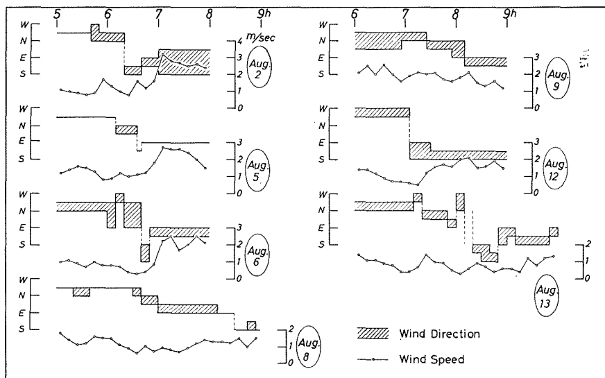
Fig. 15. Variation of wind speed and direction at Akebono in the morning in August.
