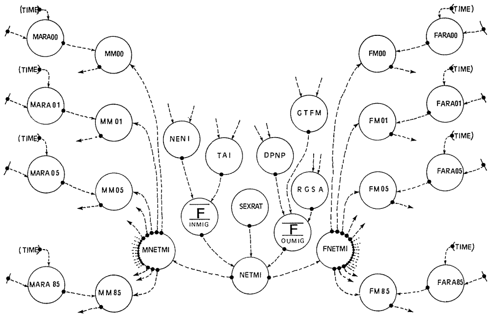
Fig. 15. Flow Diagram of Migration Sub-sector of Population Sector.
