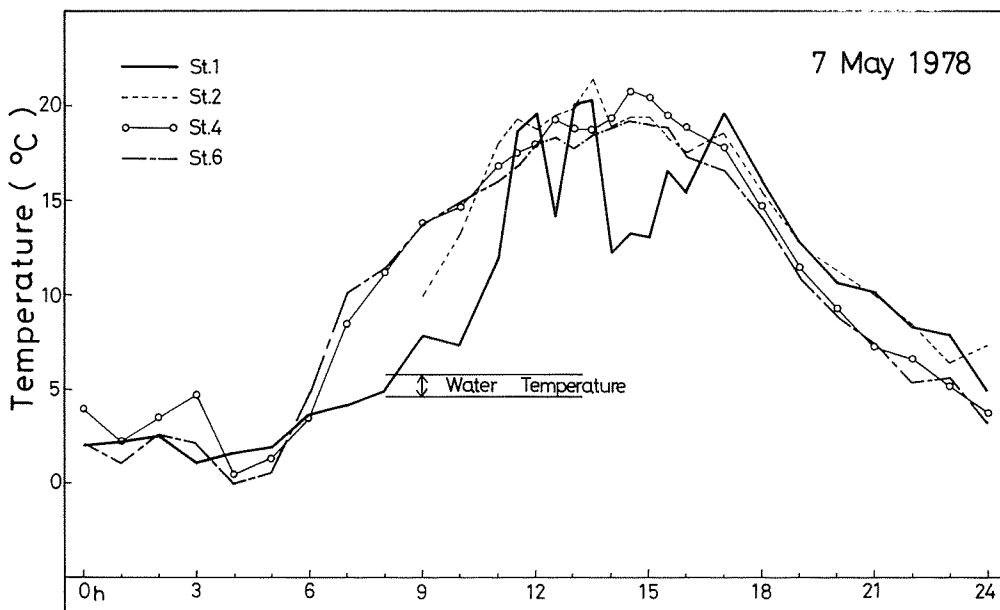
Fig. 10. Same as fig. 7 except for 7 May 1978.
