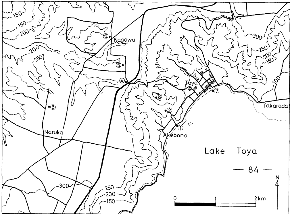
Fig. 4. Location of observation stations (Heights in meter).
