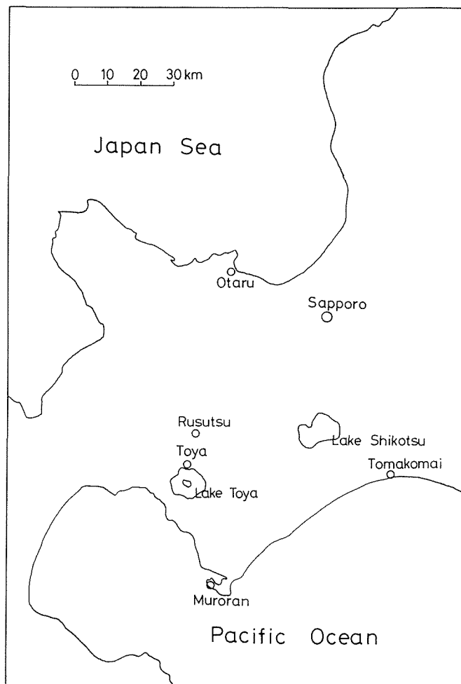
Fig. 1. Location of Lake Toya.
