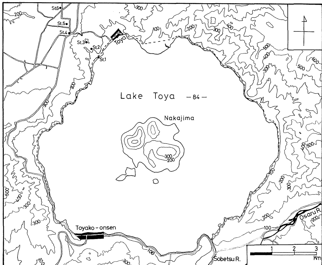
Fig. 2. Station locations and topography of Lake Toya (Heights in meter).
