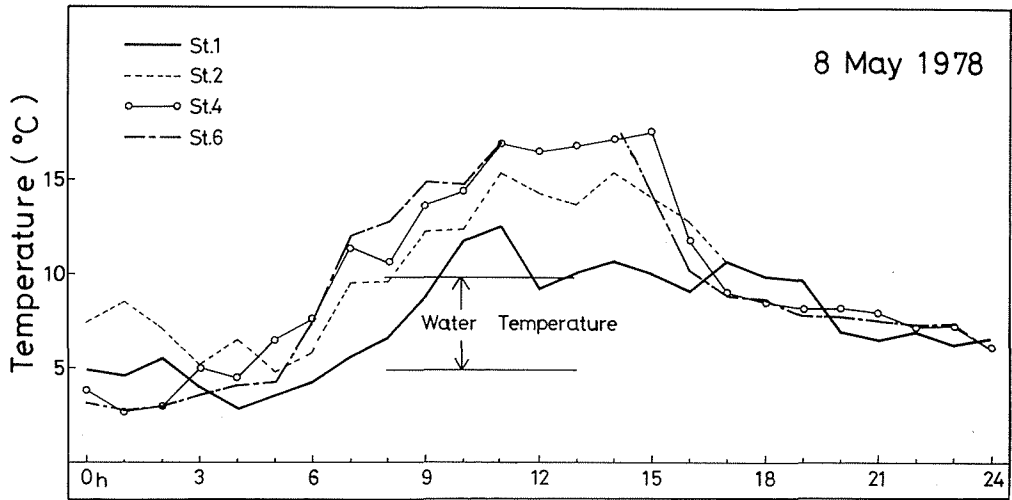
Fig. 11. Same as fig. 7 except for 8 May 1978.
