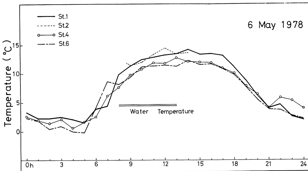
Fig. 9. Same as fig. 7 except for 6 May 1978.
