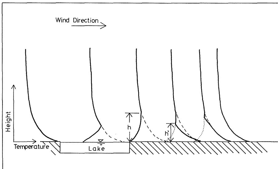
Fig. 14. Simple model of development and vanishing of cold layer.
