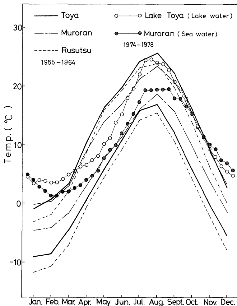
Fig. 3. Annual change of air and water temperature of Lake Toya and neighbouring region.
