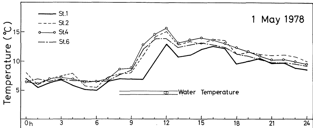
Fig. 7. Diurnal variation of air and water temperature on 1 May 1978.
