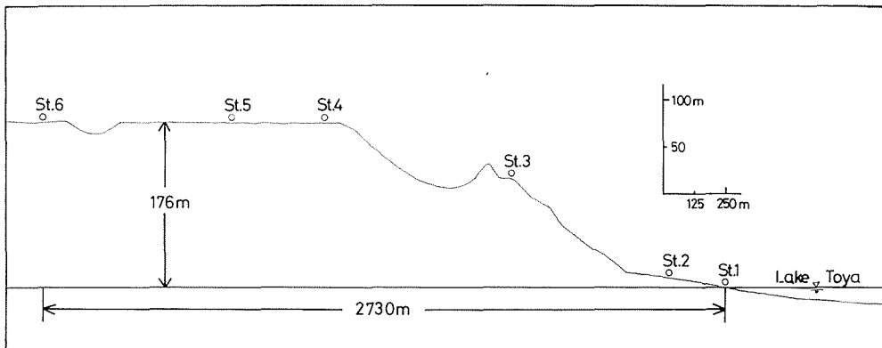
Fig. 5. Cross section of observation site.
