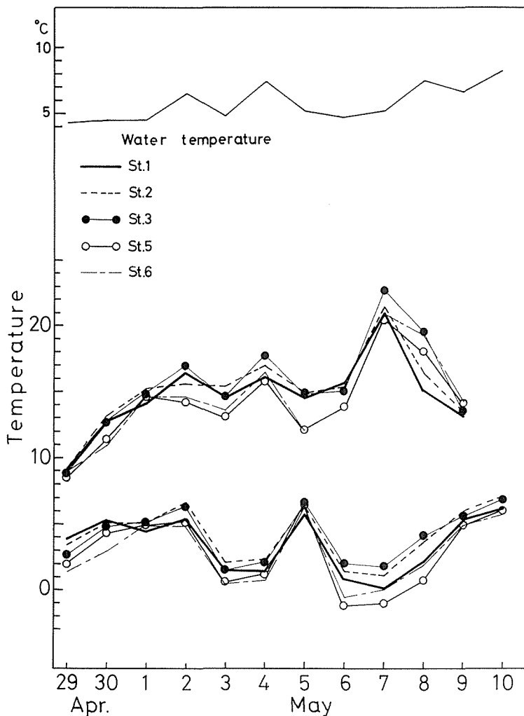
Fig. 6. Daily maximum and minimum temperature at each station and water temperature.
