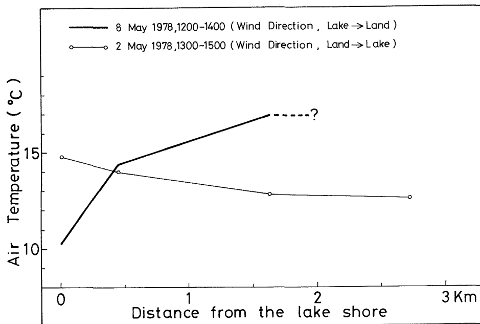
Fig. 12. Air temperature change as function of distance from the lake shore.
