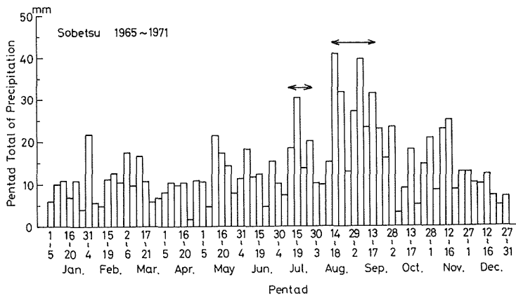
Fig. 4. Annual change of pentad total of precipitation at Sobetsu.
