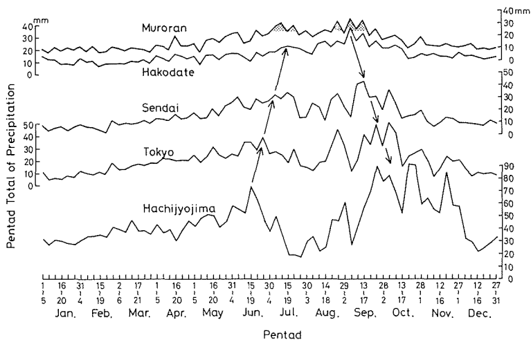
Fig. 5. Movement of rainy season.
