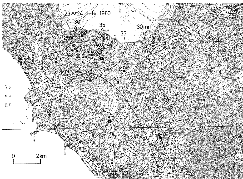
Fig. 10. Distribution of rainfall amount on 23~24 July 1980.
