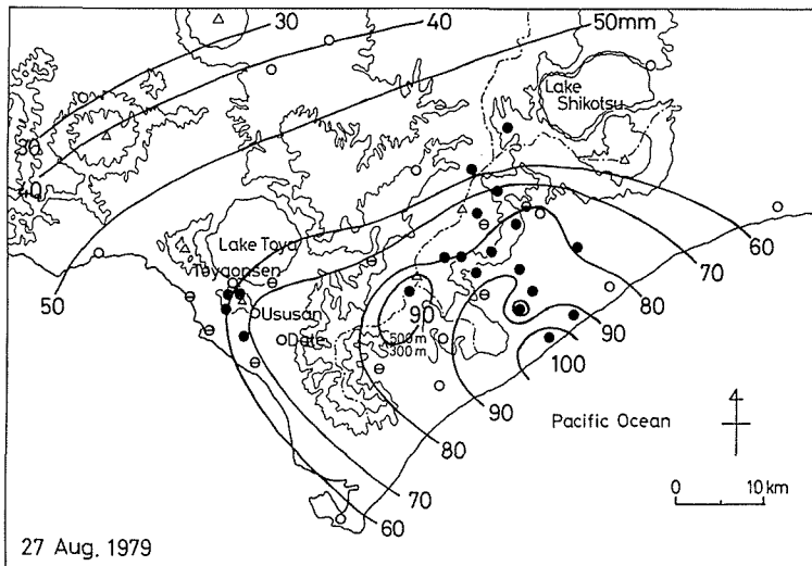
Fig. 6. A typical example of the distribution of rainfall amount by "Seaside rainfall".
