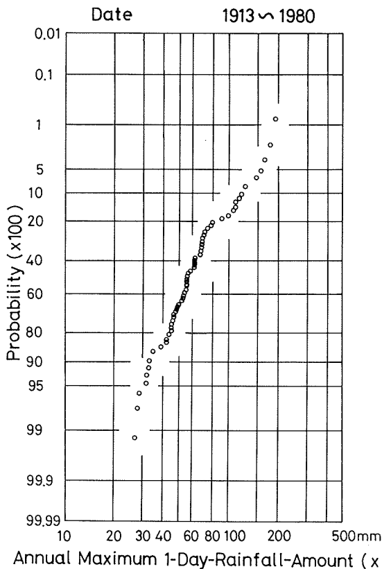
Fig. 2. Probability that an annual maximum 1-day-rainfall-amount at Date is more than x.
