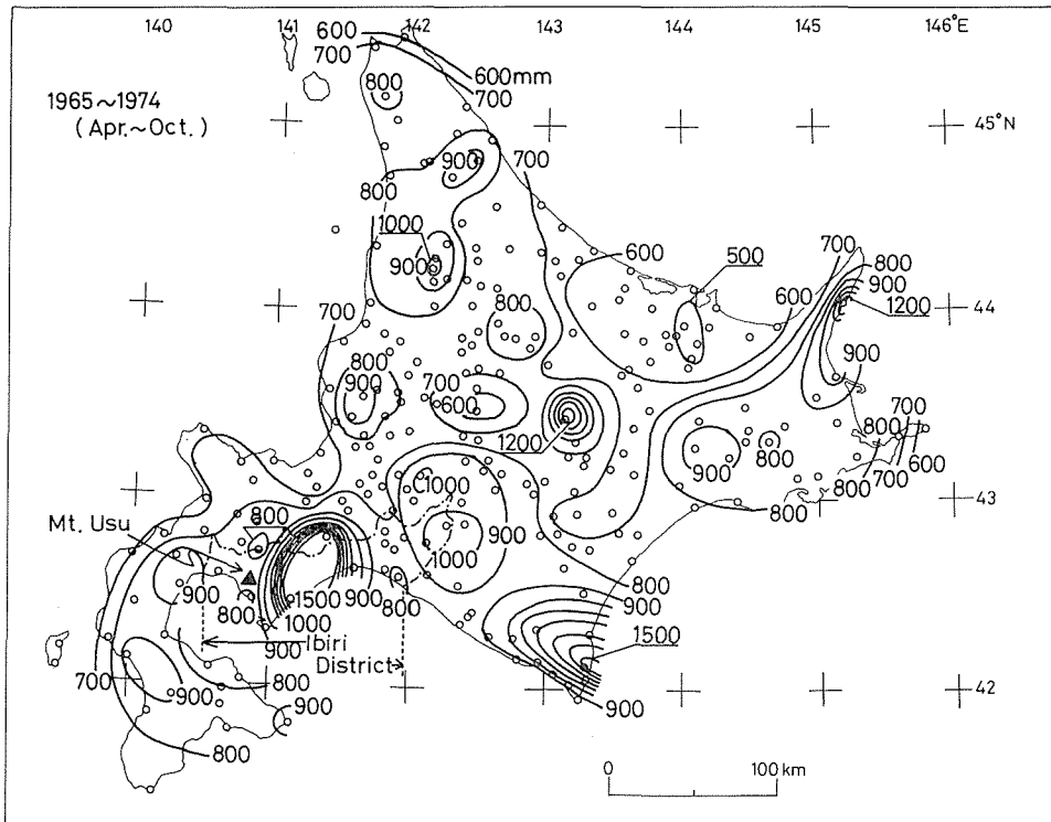
Fig. 1. Annual mean rainfall amount (April-October) from 1965 to 1974.
