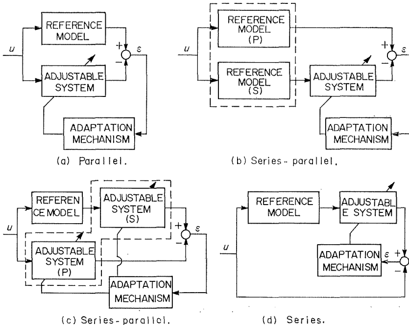
Fig. 2. Basic structures of model reference adaptive systems.
