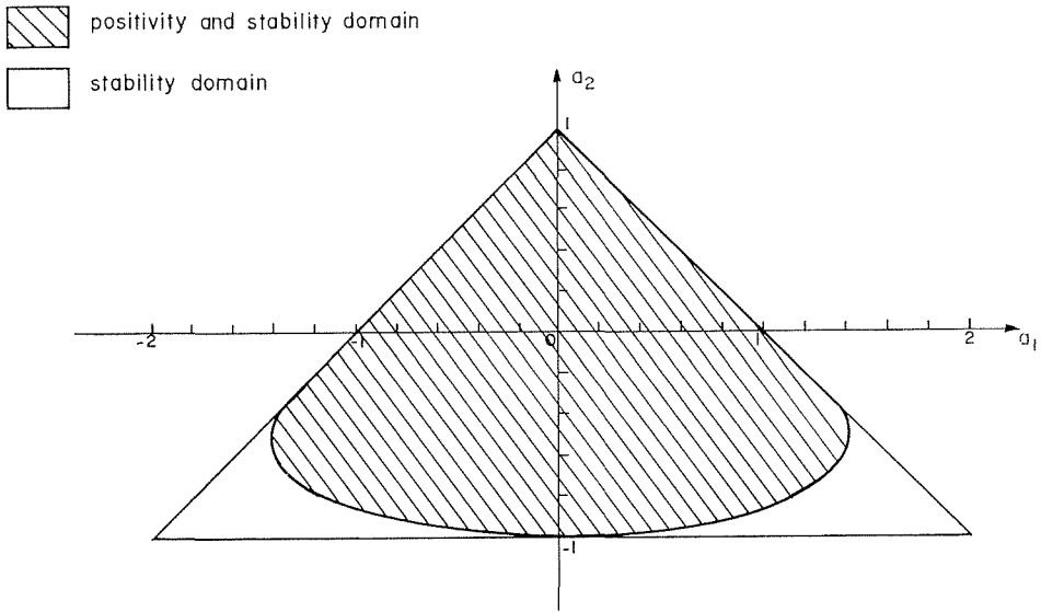
Fig. 3. Stability and positivity domain in the parameter plane for the discrete transfer function.
