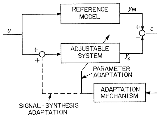
Fig. 1. Basic configuration of a model reference adaptive system.
