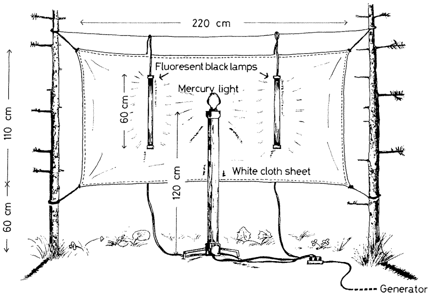
Figure 3. Sampling apparatus. The mercury light and two fluorescent black lamps were 20 W/50 Hz and 40 W/50 Hz, respectively. The power-source, a portable generator, was 30 m away from the sampling site.
