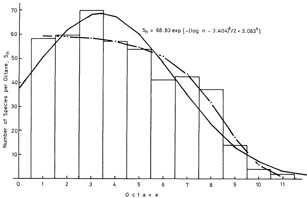
Figure 8. Species-abundance relationship. Histogram represents observations. Solid curve: a lognormal distribution, dash-dotted curve: a logseries distribution.
