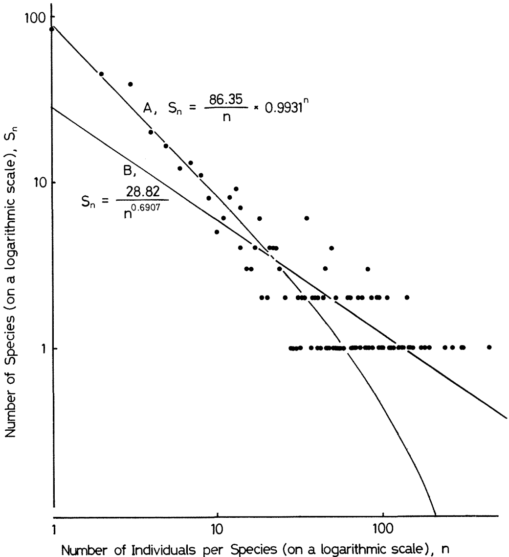
Figure 7. Species-abundance relationship. Solid circles represent observations. Curve A: a logseries distribution, curve B: a harmonic series distribution.
