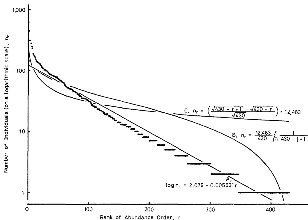
Figure 6. Species-abundance relationship. Solid circles represent observations. Curve A: a niche preemption model, curve B: a broken-stick model, curve C: a niche overlapping model.
