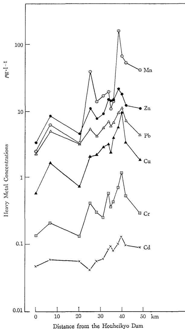
Figure 2. Distribution of Heavy Metal Concentrations in Snow of the Toyohira River Basin.
