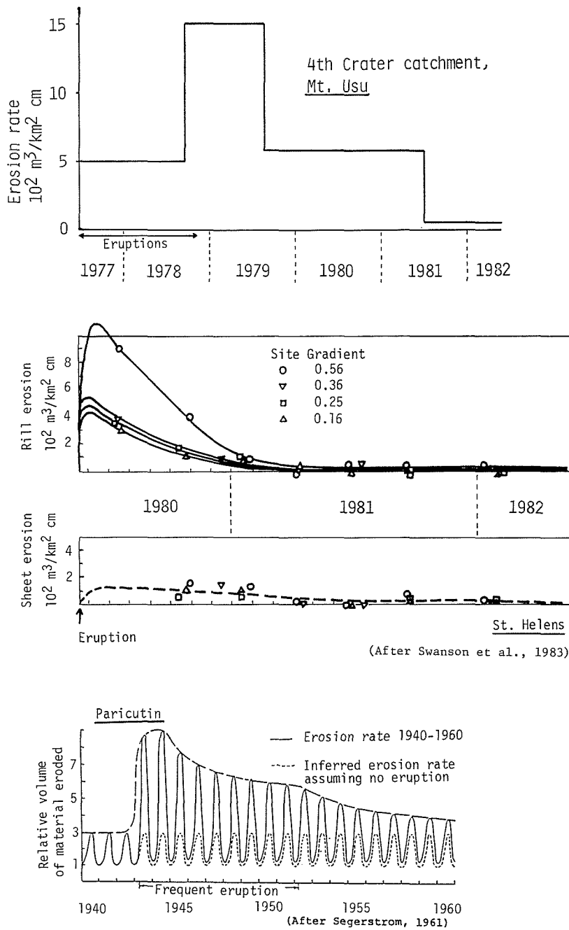
Figure 6. Erosion rate as a function of time observed at Mt. Usu (Chinen and Kadomura in press), Mt. St. Helens (Swanson et al. 1983), and Parícutin (Segerstrom 1961). Erosion rates on Mts. Usu and St. Helens in sediment volume per \text{km}^2 and cm of rainfall.
