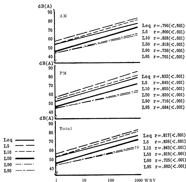
Figure 4. Correlations between Noise Levels ( L_x and L_{eq} ) and Weighted Number of Vehicles.
