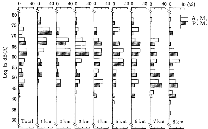
Figure 3(a). Histograms of City Noise Levels in Sapporo in Leq.
