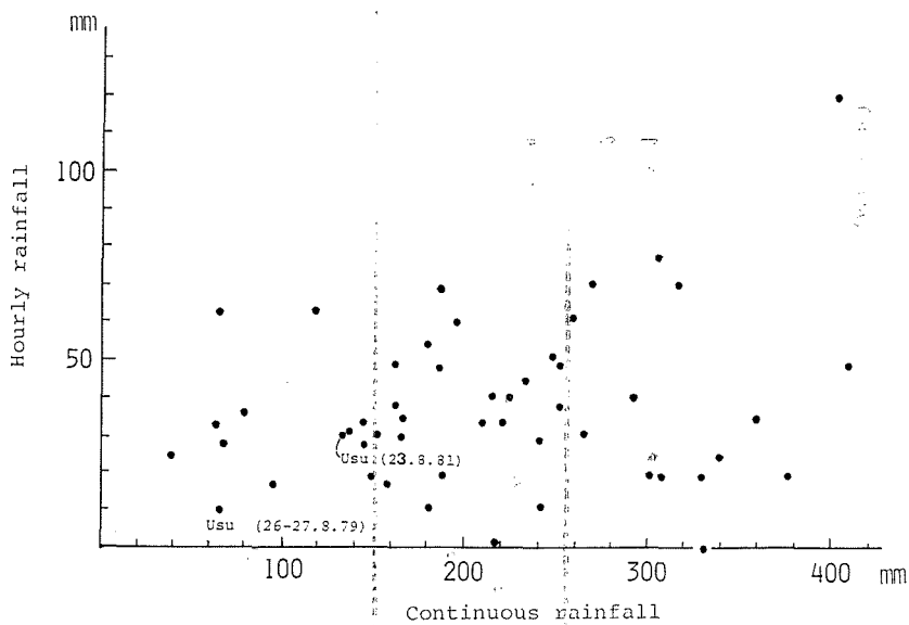
Figure 5. Relationship between continuous and hourly rainfalls related to mass movement occurring.
