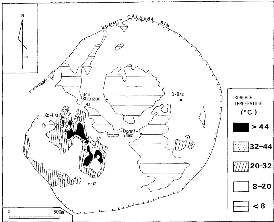
Figure 4. Surface temperatures of the caldera. As of 15. 9. 1983, 06 a.m.
