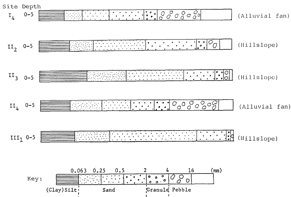
Figure 3. Grain size distribution of surficial material.
