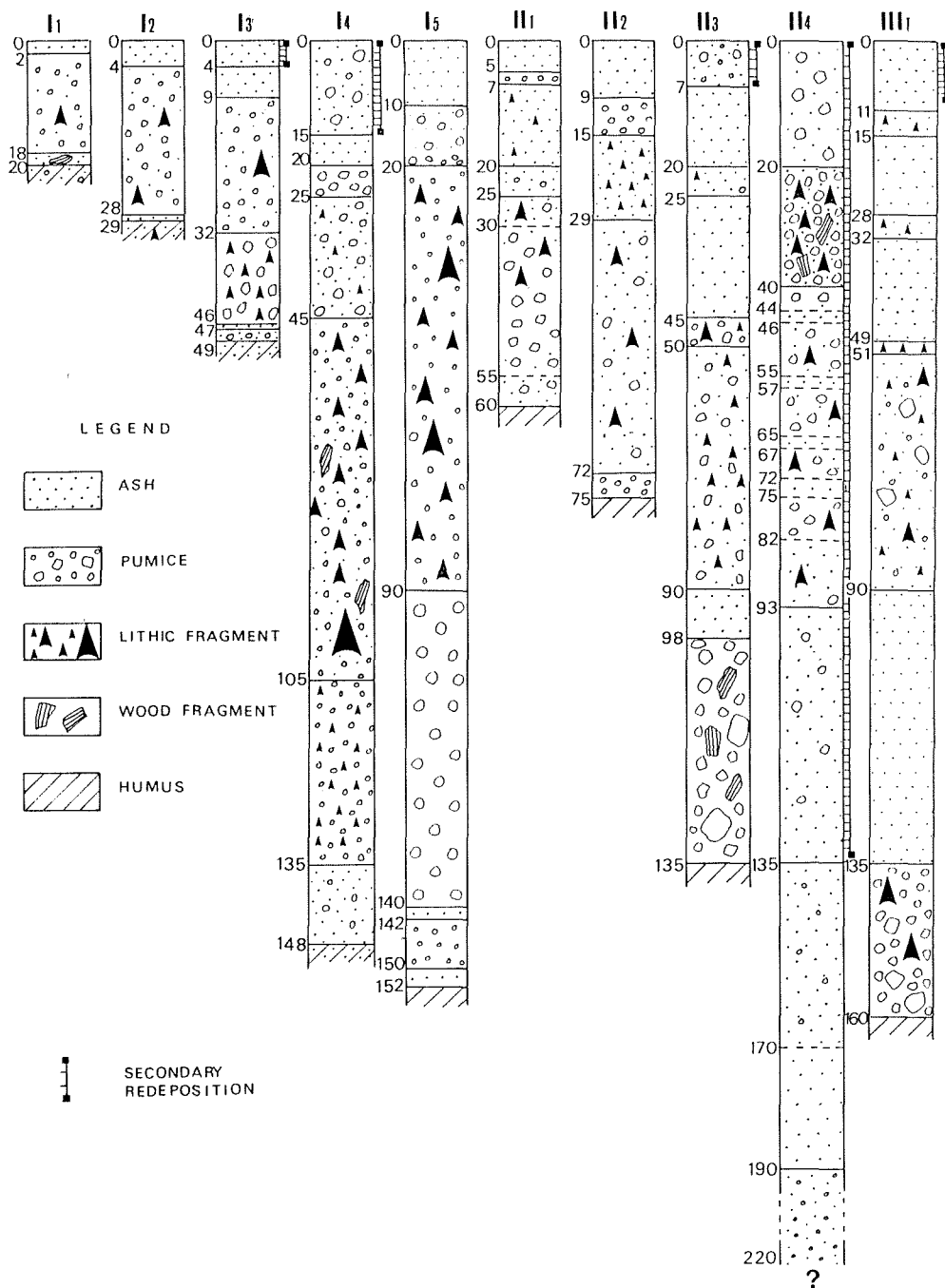
Figure 2. Air fall tephra and estimated secondary redeposition at ten sites of the summit caldera, as of May 1984. (The depth of the various layers is expressed in cm).
