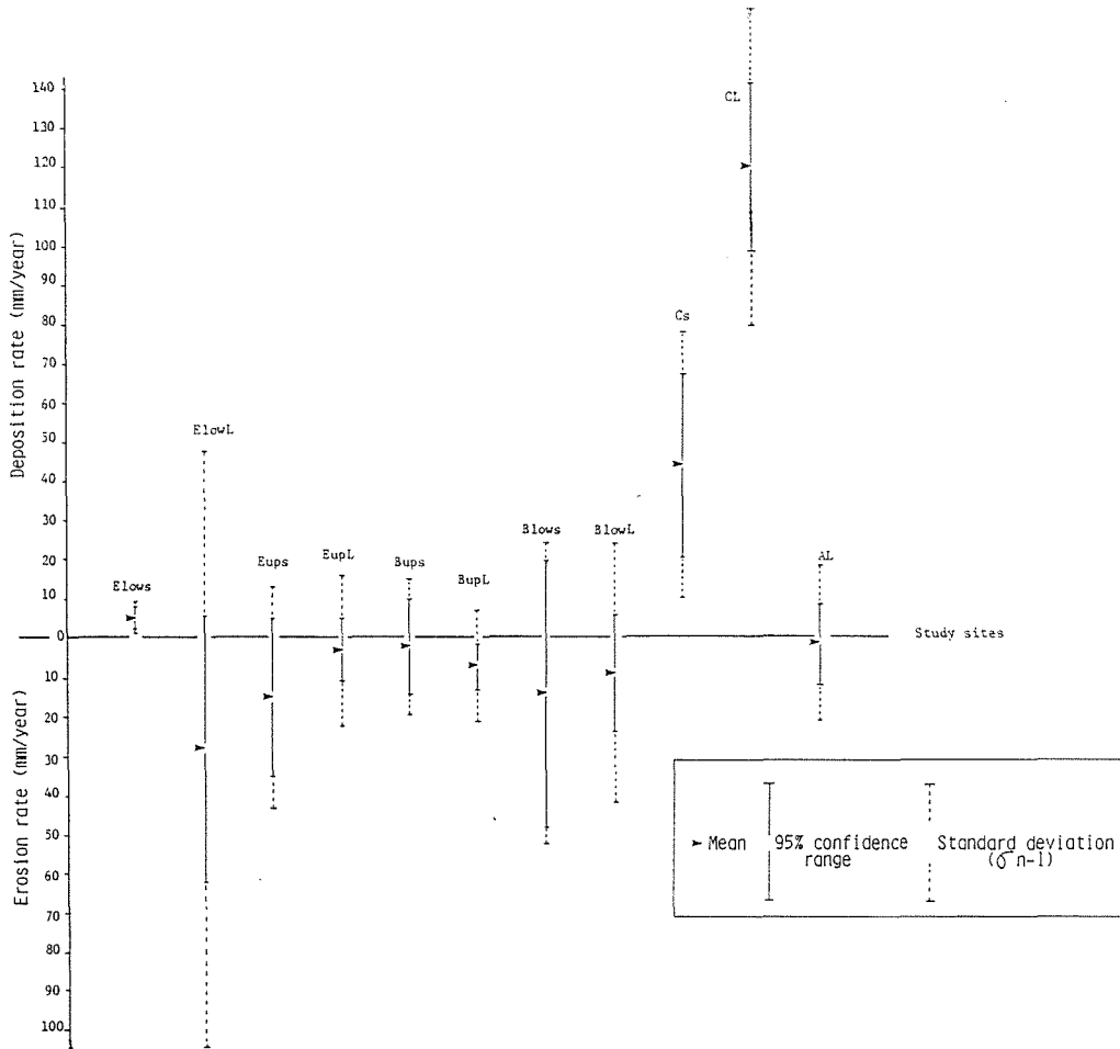
Figure 6. Ground erosion and redeposition measured by the erosion pin method at 11 sites of the caldera.
