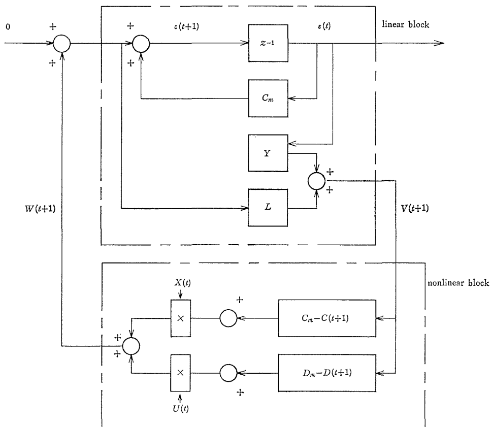
Figure 2. Discrete Equivalent Feedback System.
