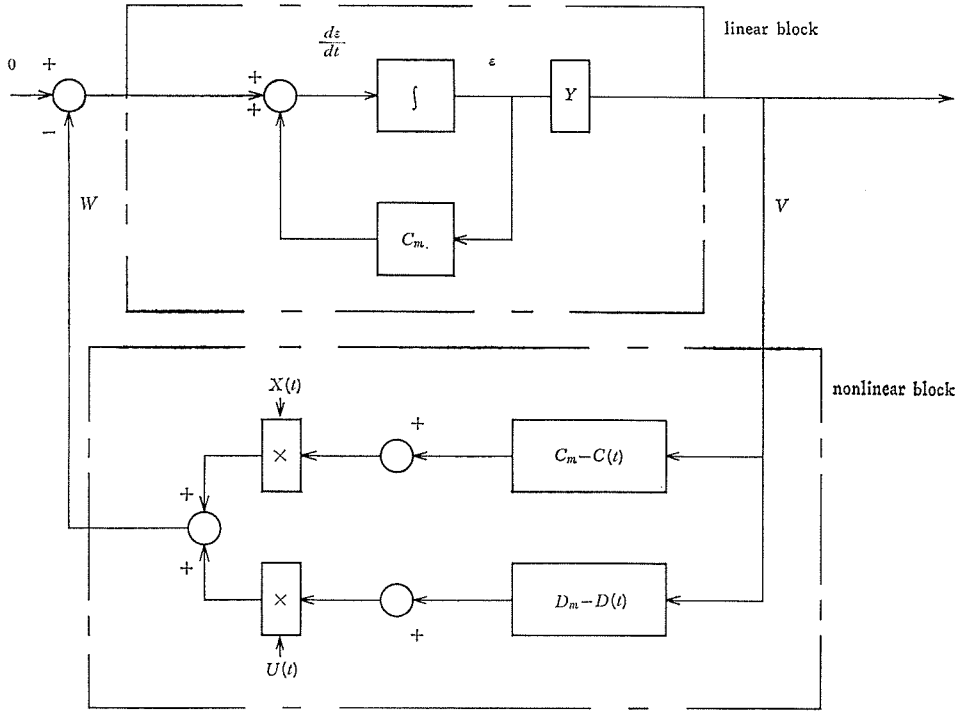
Figure 1. Equivalent Feedback System.
