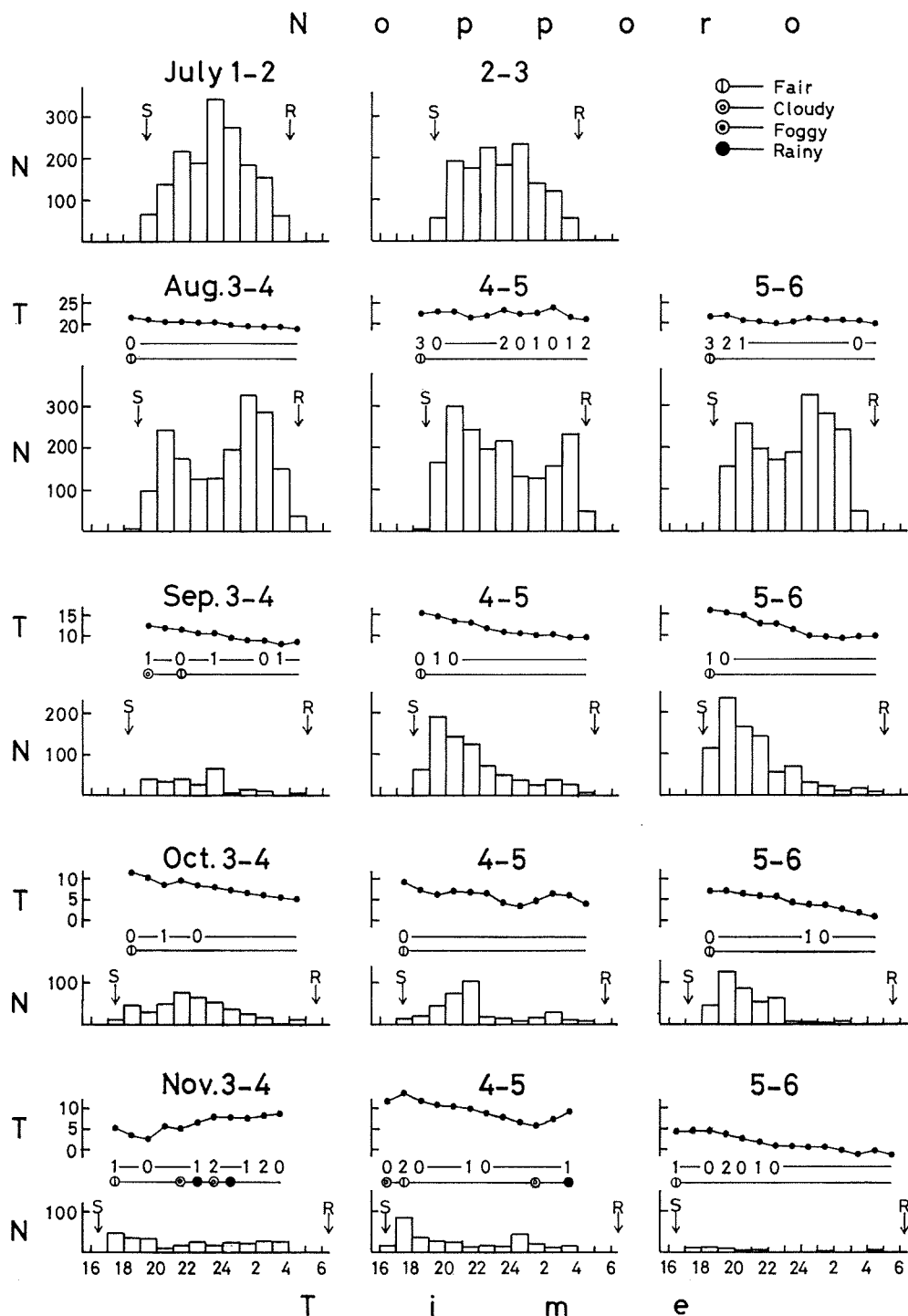
Figure 1. Fluctuation of nocturnal flight activity of moths in Nopporo Forest Park, with the changes of weather conditions. N, T, S, and R represent the number of specimens, air temperature ( ^{\circ}\text{C} ), sunset and sunrise, respectively. Wind force is also given by using Beaufort's scale.
