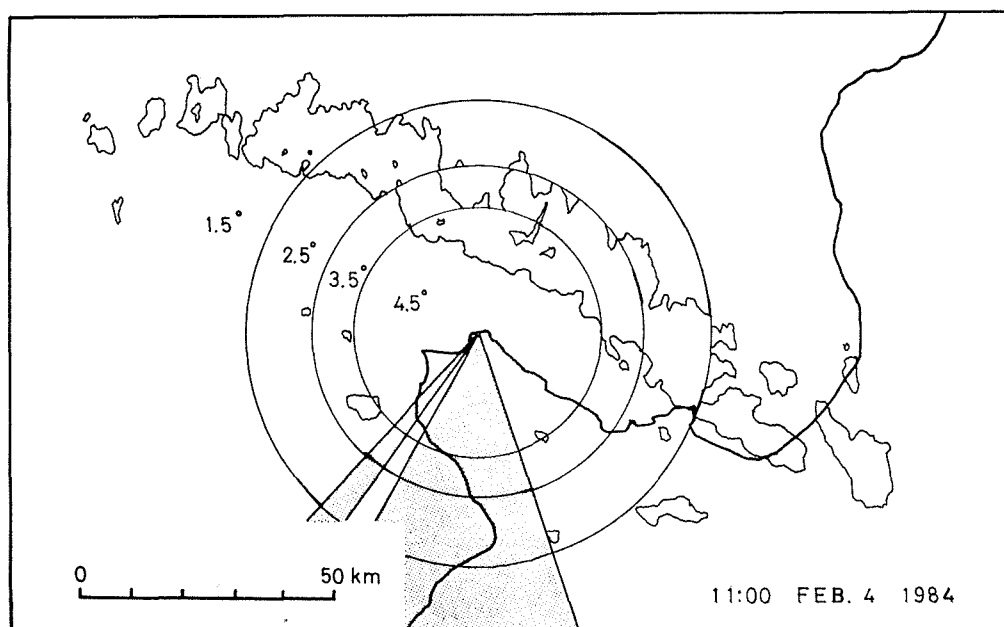
Figure 11. CAPPI echo pattern at 2 km above sea level. 1100 JST Feb. 4, 1984.
