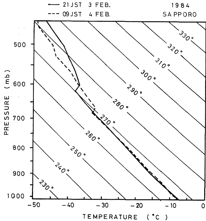
Figure 15. Temperature profiles at Sapporo, 2100 JST Feb. 3 (solid line) and 0900 JST Feb. 4 (dashed line), 1984.
