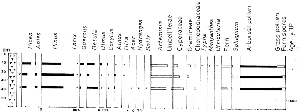
Figure 6. Pollen diagram from Dailing Section
