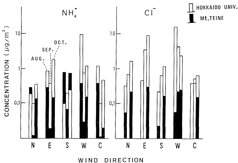
Figure 6. The same as Fig. 4 for \text{NH}_4^+ and \text{Cl}^- .
