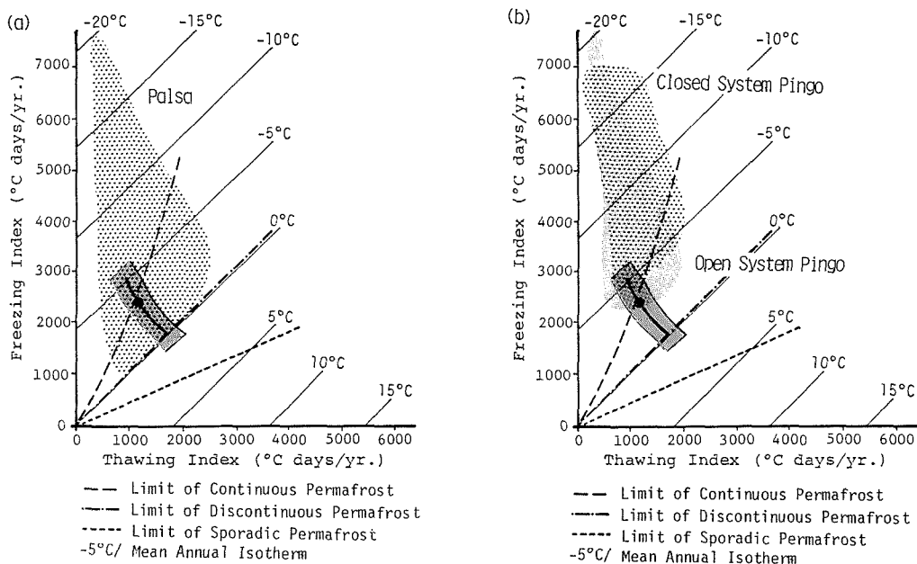
Figure 12 Possibility of the occurrence for palsas (a) and pingos (b) in the Daisetsu Mountains in relation to freezing and thawing indexes (after Harris, 1982).
