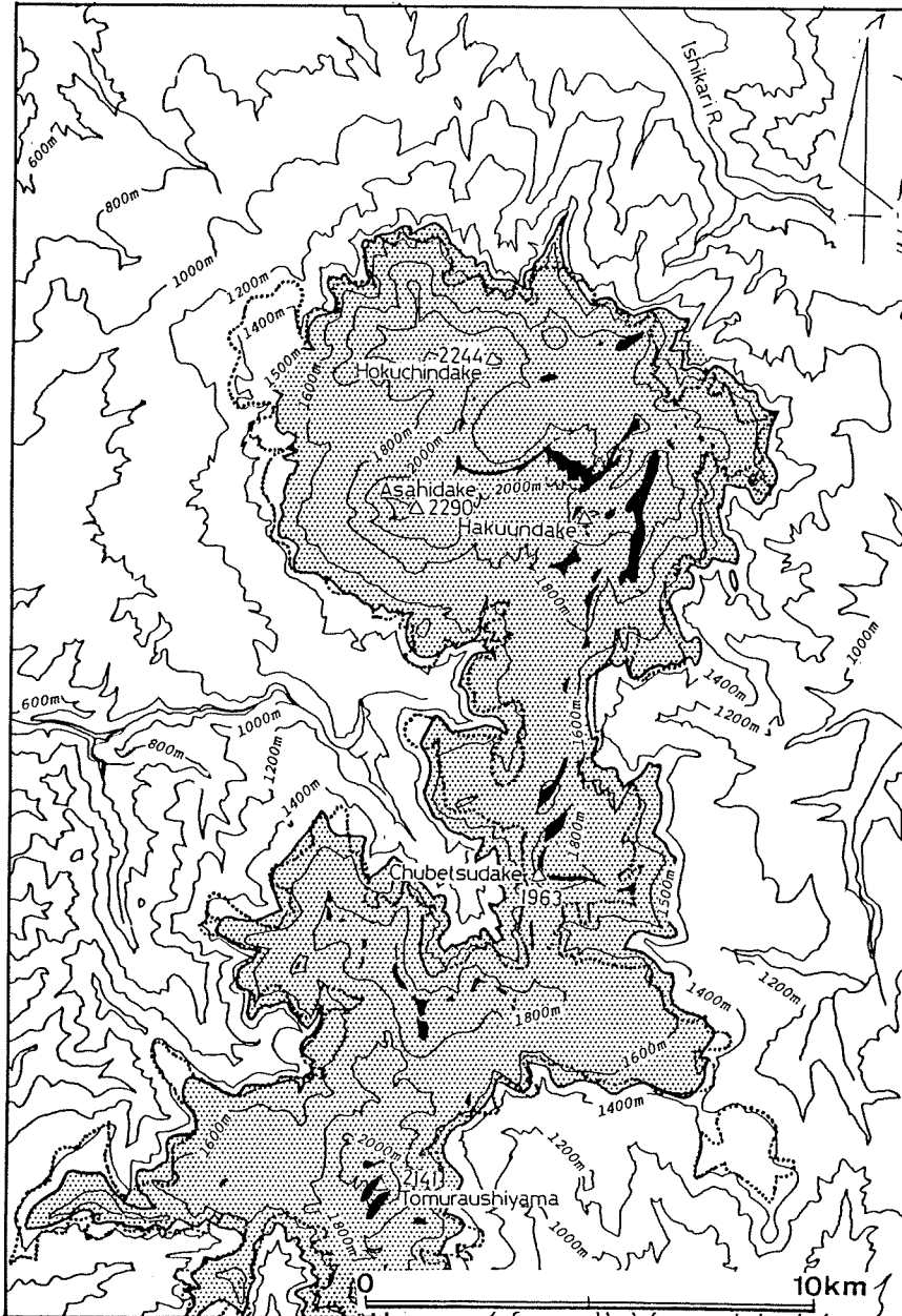
Figure 9 Inferred distribution of permafrost in the Daisetsu Mountains. shaded part: the area above 1,500 m a.s.l. dotted line: timber line (after Takahashi, 1990)
