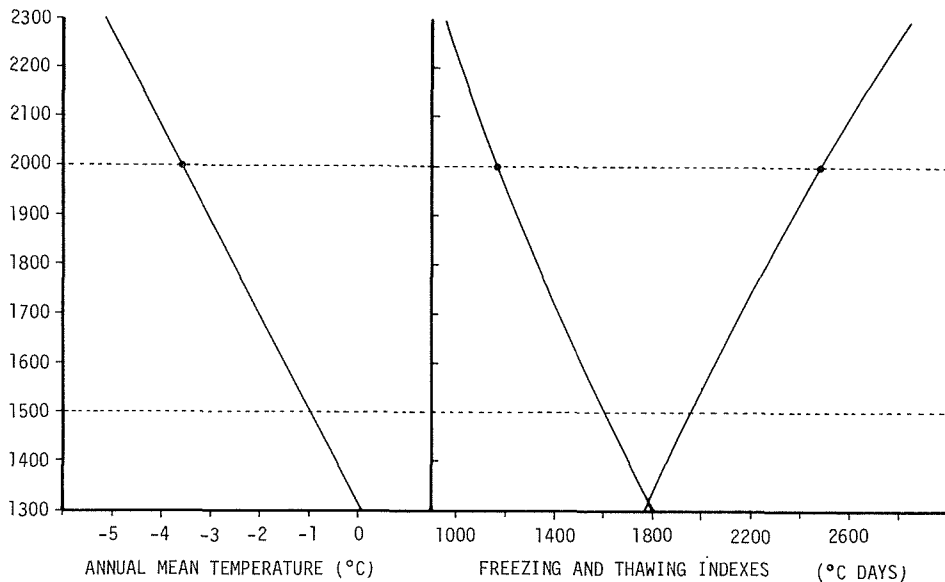
Figure 7 Estimated mean annual air temperatures, freezing and thaw indexes in the Daisetsu Mountains.
