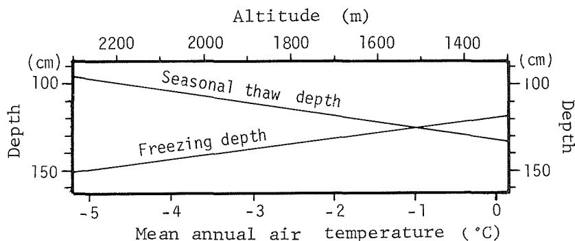
Figure 8 Potential depth of seasonal freezing and thawing versus altitude in the Daisetsu Mountains.
