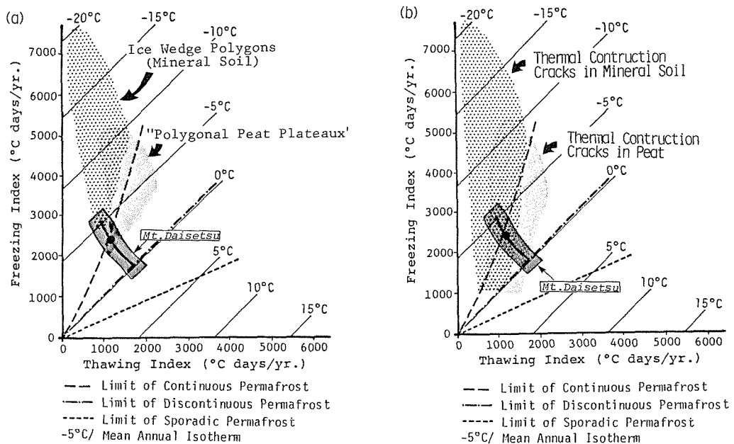
Figure 11 Possibility of the occurrence for ice wedges (a) and frost cracks (b) in the Daisetsu Mountains in relation to freezing and thawing indexes (after Harris, 1982).
