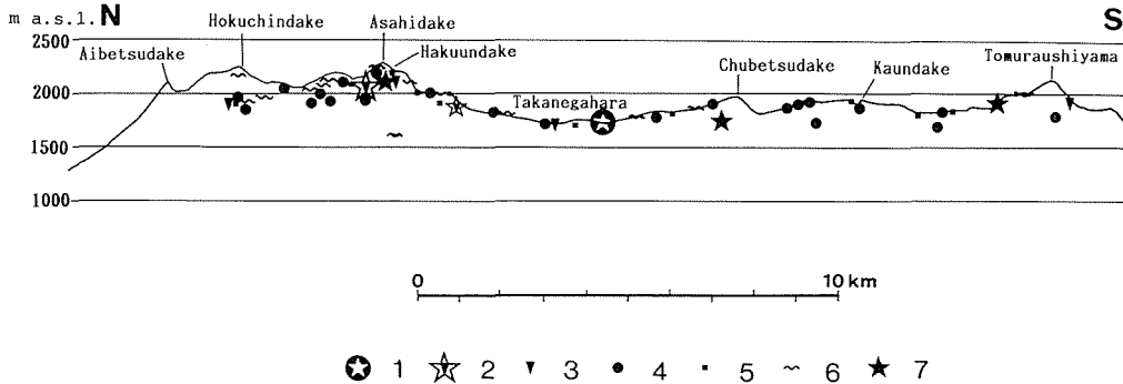
Figure 3 Vertical distribution of periglacial landforms in the Daisetsu Mountains. Legend is shown in Figure 2.
