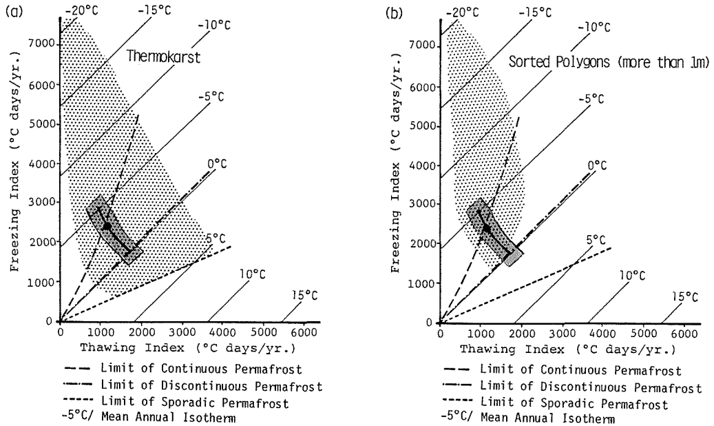
Figure 14 Possibility of the occurrence for thermokarst features (a) and sorted polygons (b) in the Daisetsu Mountains in relation to freezing and thawing indexes (after Harris, 1982).
