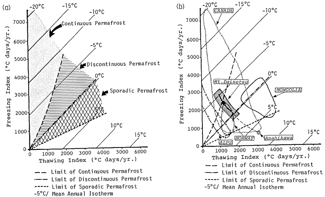
Figure 10 a) Relationship between permafrost zones and freezing and thawing indexes (after Harris, 1981a). b) Range of freezing and thawing indexes of the Daisetsu Mountains plotted on the diagram of Harris (1981a) with the data for Canada, Mongolia, Norway, and the Alps.
