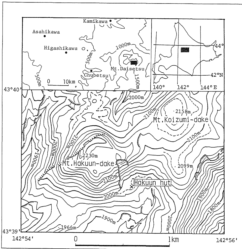
Figure 4 Location of Hakuun hut.
