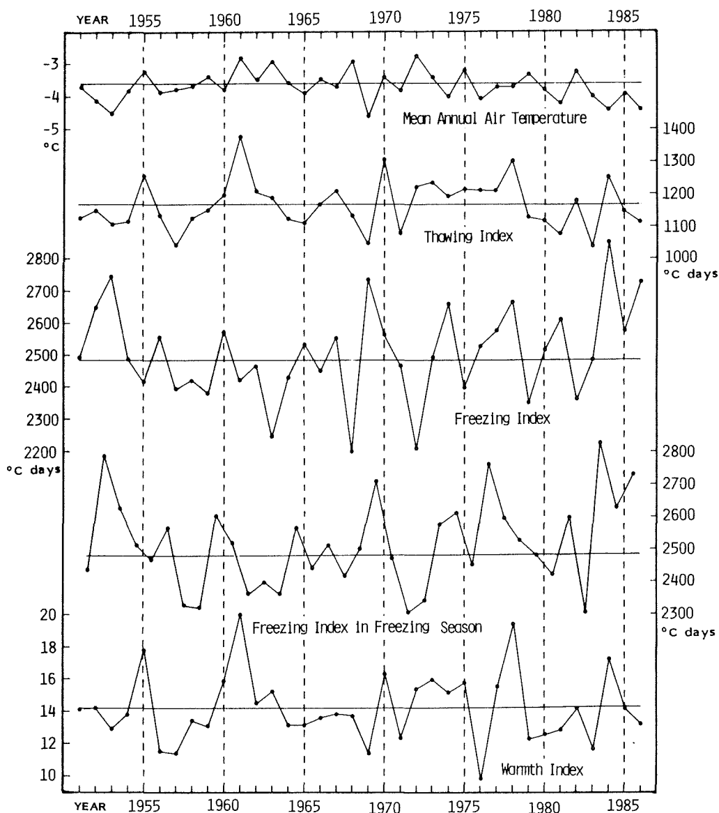
Figure 6 Year-to-year variations of air temperature and warmth, freezing and thawing indexes at Hakuun hut.
