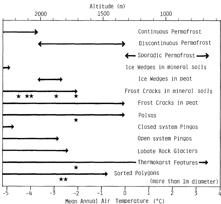
Figure 15 Possibility of the occurrence for permafrost zones and periglacial landforms, and the actual distribution of periglacial landforms (star) in the Daisetsu Mountains.
