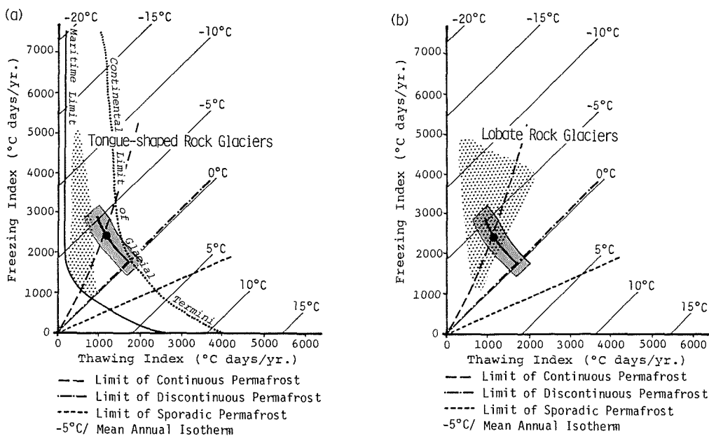
Figure 13 Possibility of the occurrence for tongue-shaped rock glaciers (a) and lobate rock glaciers (b) in the Daisetsu Mountains in relation to freezing and thawing indexes (after Harris, 1981a).
