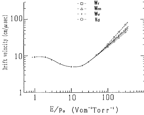
Figure 1. The electron drift velocities in methane : ( W_r ) the centre-of-mass drift velocity, ( W_v ) the mean drift velocity, ( V_d ) the drift velocity for the steady-state-Townsend experiment and ( W_m ) the mean arrival time drift velocity.
