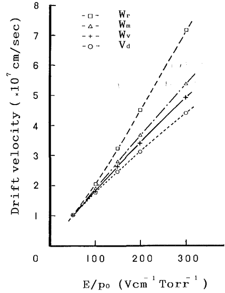
Figure 2. The electron drift velocities re-plotted on linear scales. The symbols for drift velocity are the same as in figure 1.
