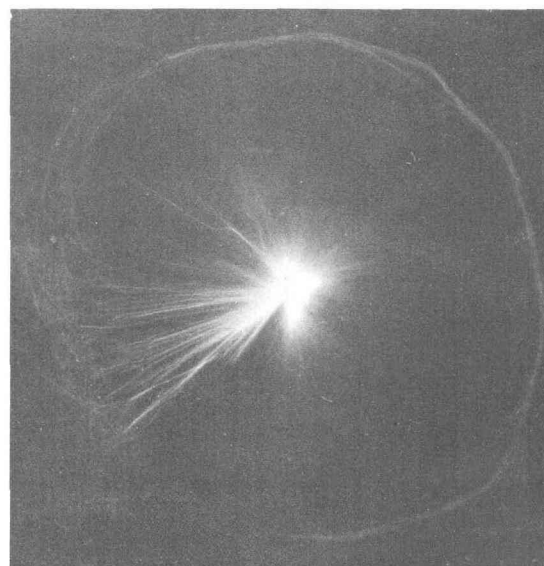
Porcelain : l = .65 cm. (Transformer)
