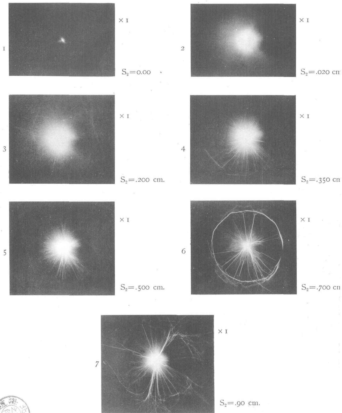
Fig. 7. Spark figure at different widths of the series spark gap.
