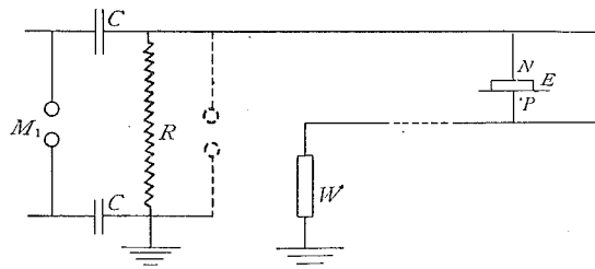
M_1 : Sphere gap. C : Meirowsky Condenser. R : Water Rheostat. W : Resistance (equivalent to Surge Impedance of line). N-E-P : Apparatus for surface charge figure.
