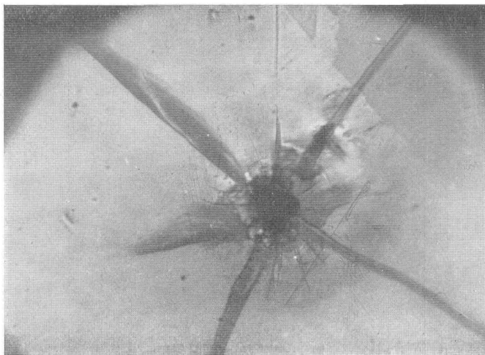
Fig. 50. Scabs due to the "second negative streamer" on the cover glass plate. (magnification 100)
