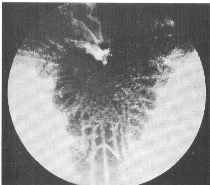
Fig. 26. Positive streamer in mica. (magnification 50)
