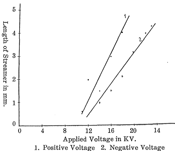
Fig. 16. Streamer in glass.
