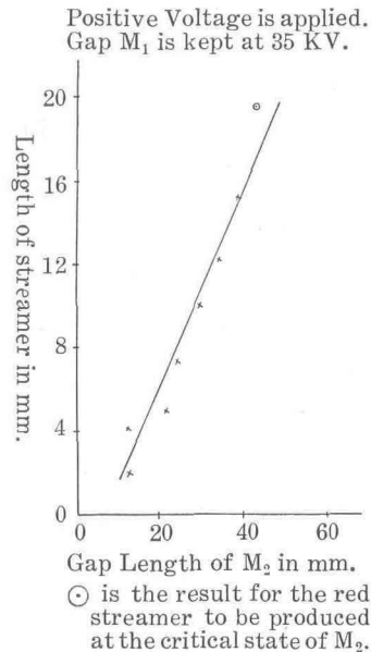
Fig. 8. Streamer in water to be produced with the chopped wave.
