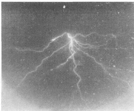
Fig. 12. Streamer in glass. (magnification 30)
