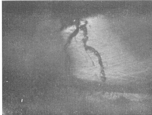
Fig. 14. Scabs due to the streamer left in the glass. (magnification 150)
