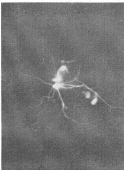
Fig. 55. A drop of petroleum is blazed up with the streamer along the water surface.
