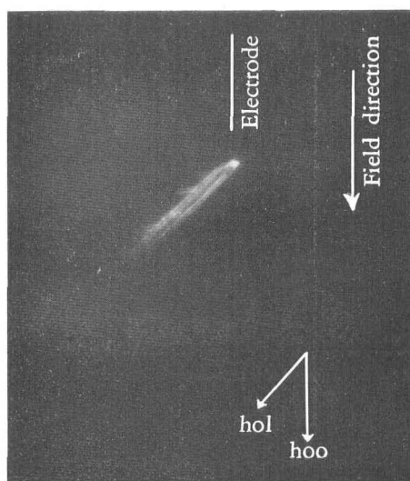
Fig. 24. Streamer in tartaric acid. (magnification 10)
