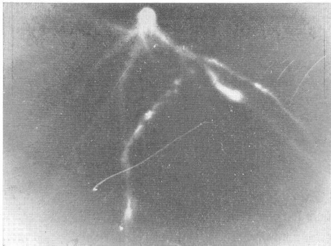
Fig. 15. Streamer in glass. (magnification 30)
