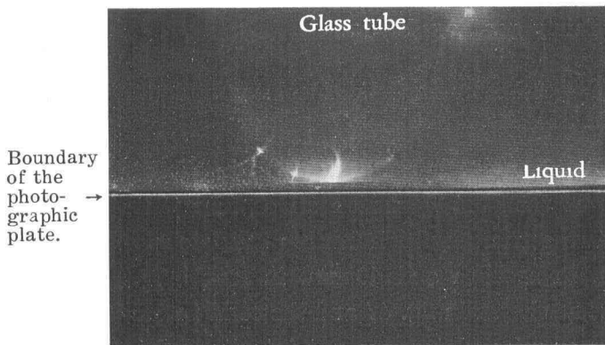
Fig. 45. Streamers in the glass tube and in the liquid (water). (magnification 3)
