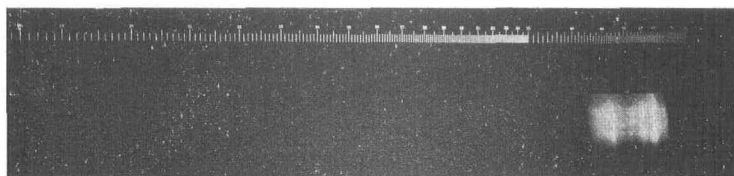
Fig. 41. Spectrum of the spark in transformer oil due to the long wave.
