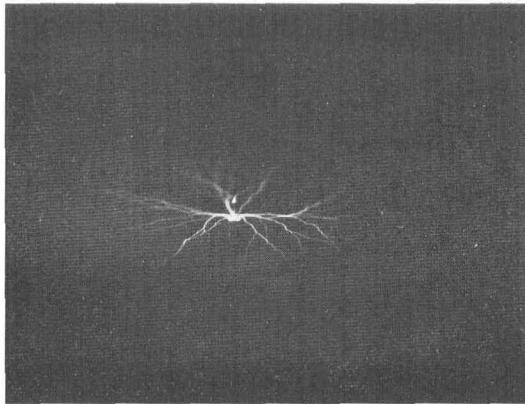
Fig. 54. Positive streamer along water surface.
