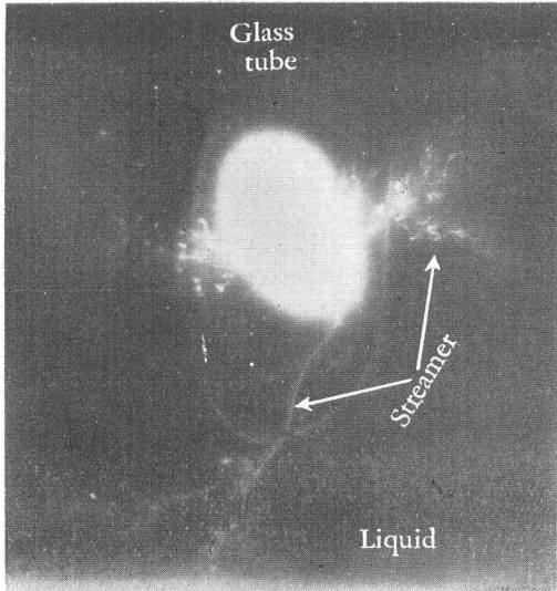
Fig. 43. Streamer in the glass tube and in the liquid (glycerine). (magnification 3)
