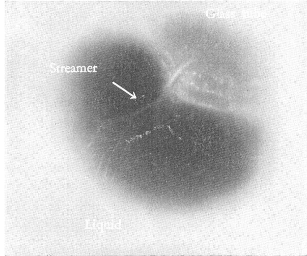
Fig. 44. Streamers in the glass tube and in the liquid (glycerine).
