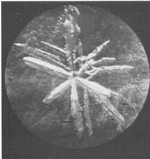
Fig. 29. Negative streamer in mica. (magnification 50)
