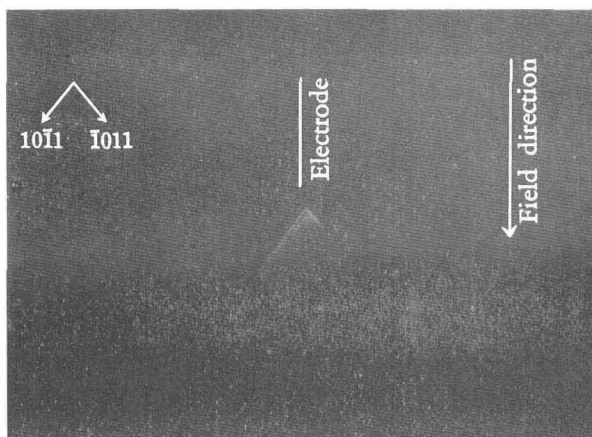
Fig. 25. Streamer in calcite. (magnification 5)
