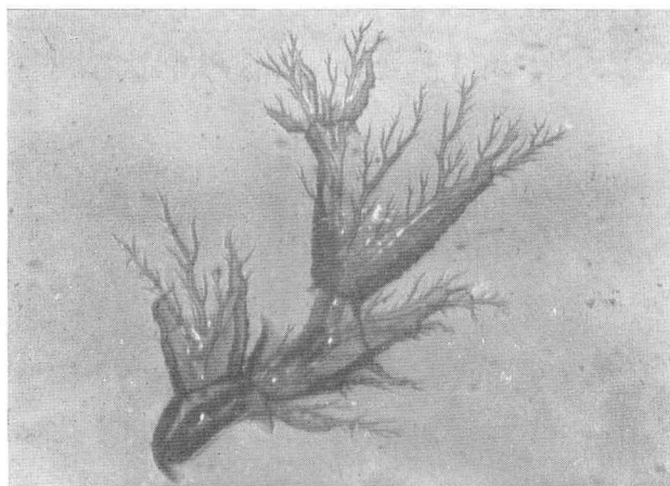
Fig. 13. Scabs due to the streamer left in the glass. (magnification 50)
