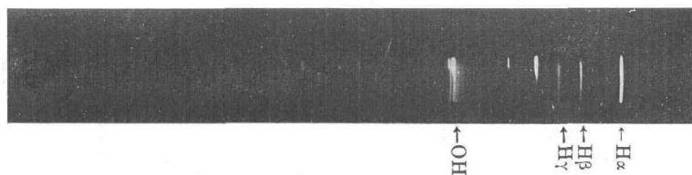
Fig. 32. Red streamer in water due to the unchopped wave.
