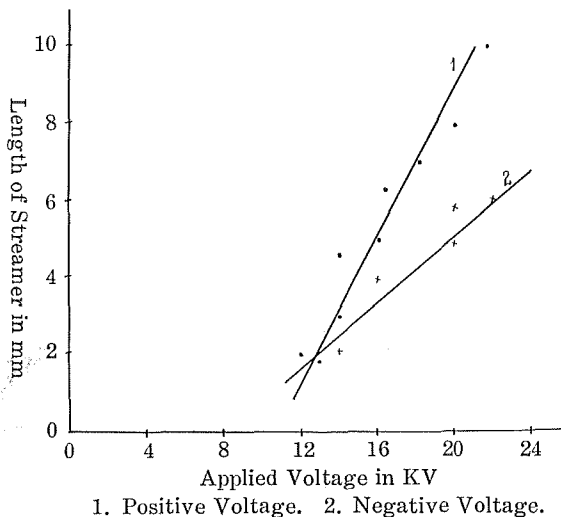
Fig. 6. Streamer in water to be produced with the unchopped wave.
