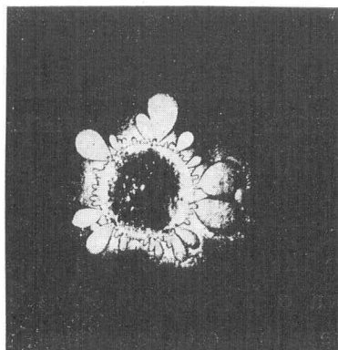
Fig. 2. Negative Dust Figure on Window Glass in Transformer Oil. D.C. Voltage 28 kV. R.H. 43% T. 18°C
