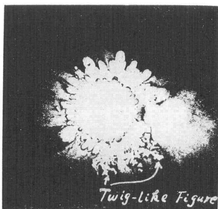
Fig. 9. Positive Dust Figure on Window Glass in Transformer Oil.
