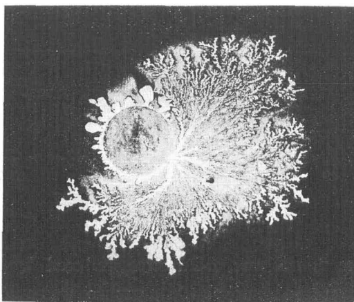
Fig. 10. Positive Dust Figure on Window Glass in Transformer Oil. Pulsating Voltage 28 kV. Atmospheric Pressure 30 cm. Hg. R.H. 43% T. 18°C
