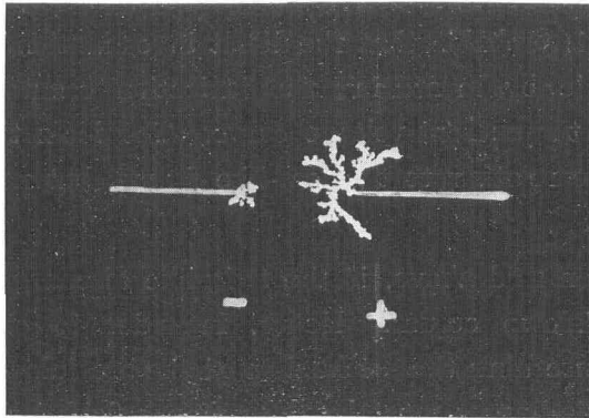
Fig. 6. Dust Figure on Window Glass in Petroleum. Impulse Voltage 38.5 kV. max. R.H. 48% T. 18°C
