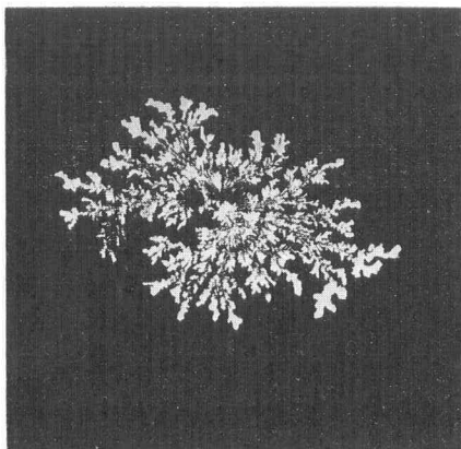
Fig. 1. Positive Dust Figure on Window Glass in Transformer Oil. Impulse Voltage 39.5 kV. max. R.H. 47% T. 21°C
