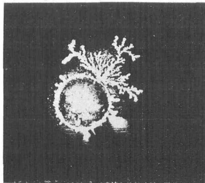
Fig. 4. Positive Dust Figure on Window Glass in Petroleum. Pulsating Voltage 24.5 k.V. R.H. 55% T. 20°C
