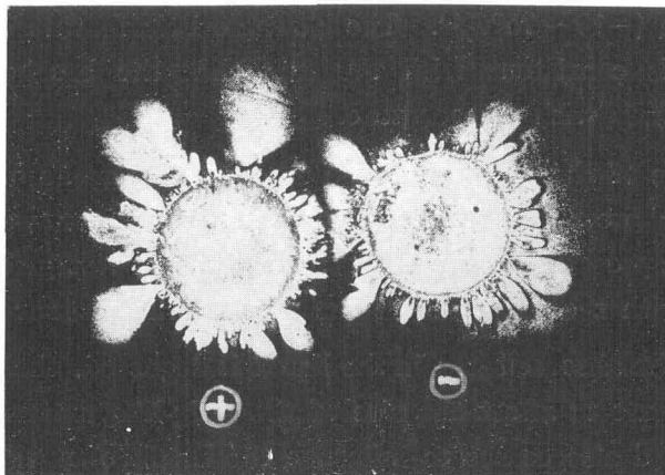
Fig. 7. Dust Figure on Pyrex Glass in Petroleum. Pulsating Voltage 40.5 kV. R.H. 57% T. 19°C
