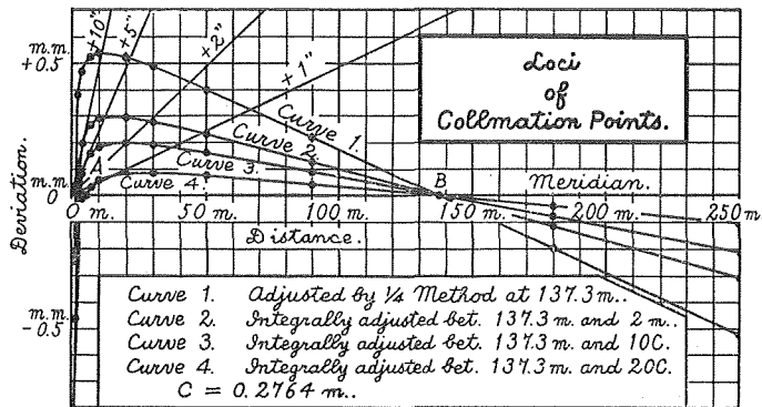
Fig. 34. Illustration of Integral Adjustment of the Vertical Cross-Hair of Transit No. 4.
