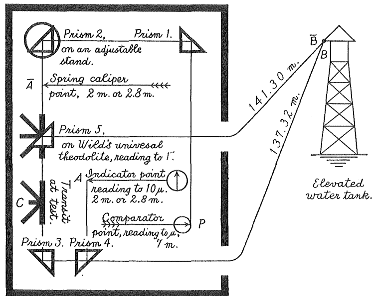
Fig. 21. Apparatus for the First Experiment.
