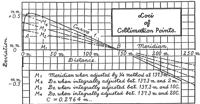
Fig. 40. Method for Determining E_A .
