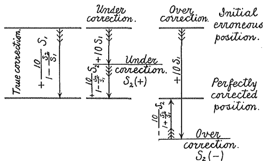
Fig. 12. Illustration of the Trial Method of Integral Adjustment of the Horizontal Cross-Hair in a Transit.
