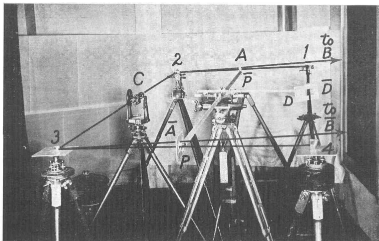
Fig. 25. Apparatus for the Second and the Fourth Experiments.
