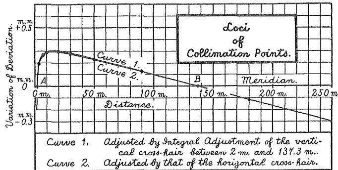
Fig. 38. Variations of Deviations of Collimation Points in Transit No. 4 after Integral Adjustment.
