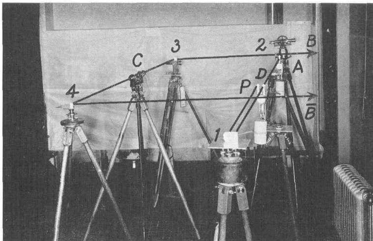
Fig. 46. Apparatus for Test and Integral Adjustment of the Horizontal Cross-Hair in a Wye Level.
