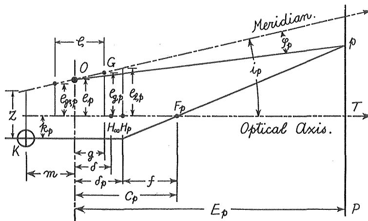
Fig. 14. Deviation of a Collimation Point.
