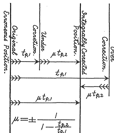
Fig. 31. Illustration of the Trial Method of Integral Adjustment.
