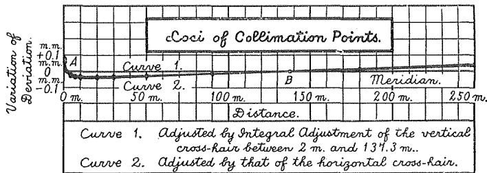
Fig. 39. Variations of Deviations of Collimation Points in Transit No. 7 after Integral Adjustment.
