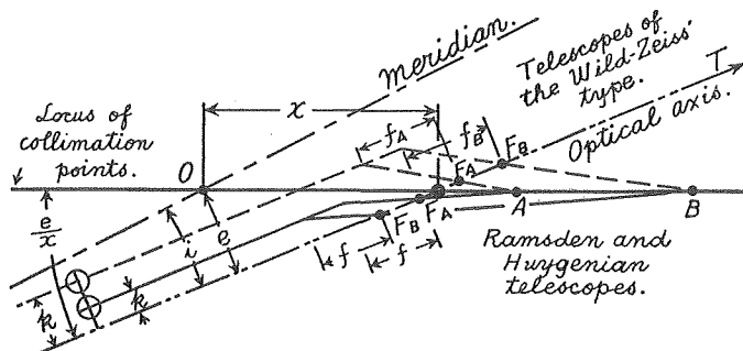
Fig. 20. Optical Relations when the Cross-Hair is adjusted by the Method of Integral Adjustment of the Horizontal Cross-Hair.
