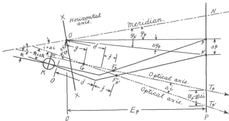
Fig. 17. Adjustment of the Inclination of the Optical Axis of the Objective Lens System.
