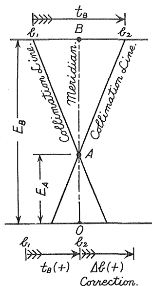
Fig. 30. Fourth Method of Integral Adjustment.
