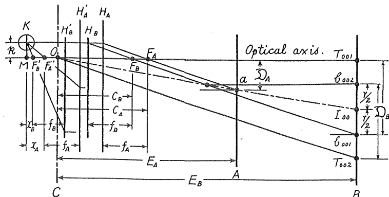
Fig. 11. Optical Relations when the Horizontal Cross-Hair is adjusted by the Second Method of Integral Adjustment in case of e = 0 and i = 0 .
