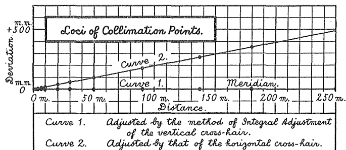
Fig. 36. Illustration of Integral Adjustment of the Vertical Cross-Hair of Transit No. 4.
