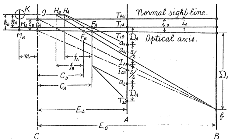
Fig. 7. Optical Relations when the Horizontal Cross-Hair is adjusted by the First Method of Integral Adjustment.
