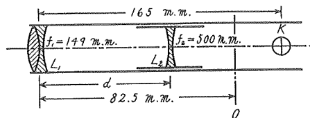
Fig. 5. Wild-Zeiss' Telescope.
