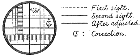
Fig. 13. Simultaneous Adjustment of the Cross-Hairs in a Transit.
