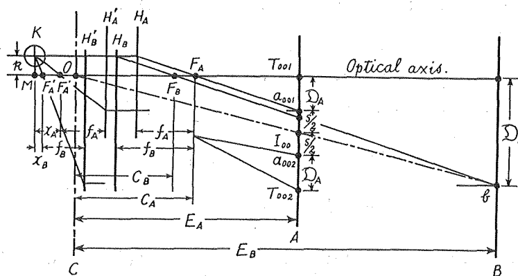
Fig. 8. Optical Relations when the Horizontal Cross-Hair is adjusted by the First Method of Integral Adjustment in case of e = 0 and i = 0 .
