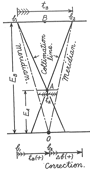
Fig. 29. Third Method of Integral Adjustment.
