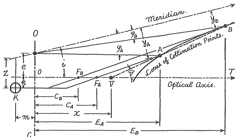
Fig. 18. Illustration of the Point V.
