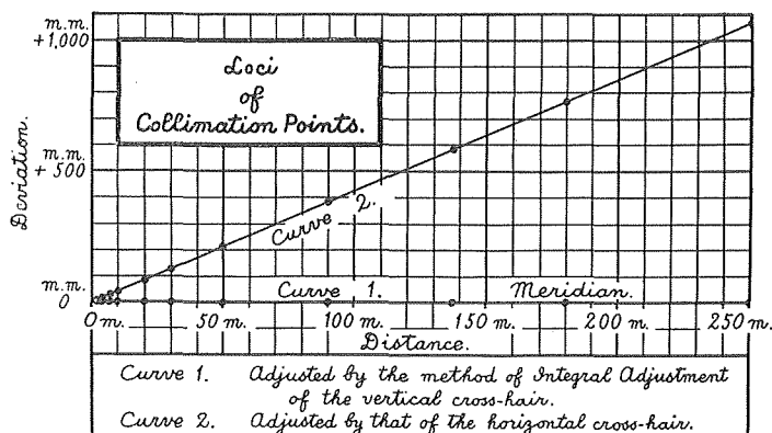
Fig. 37. Illustration of Integral Adjustment of the Vertical Cross-Hair of Transit No. 7.
