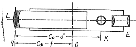
Fig. 2. Ramsden's Telescope.
