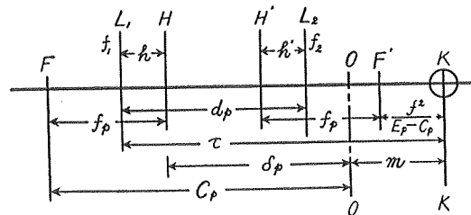
Fig. 1. General Optical Relations in the Objective Lens System.
