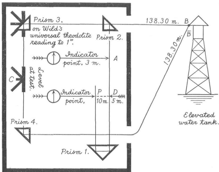
Fig. 45. Apparatus for Test and Integral Adjustment of the Horizontal Cross-Hair in a Wye Level.
