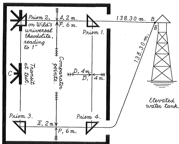
Fig. 24. Apparatus for the Second and the Fourth Experiments.
