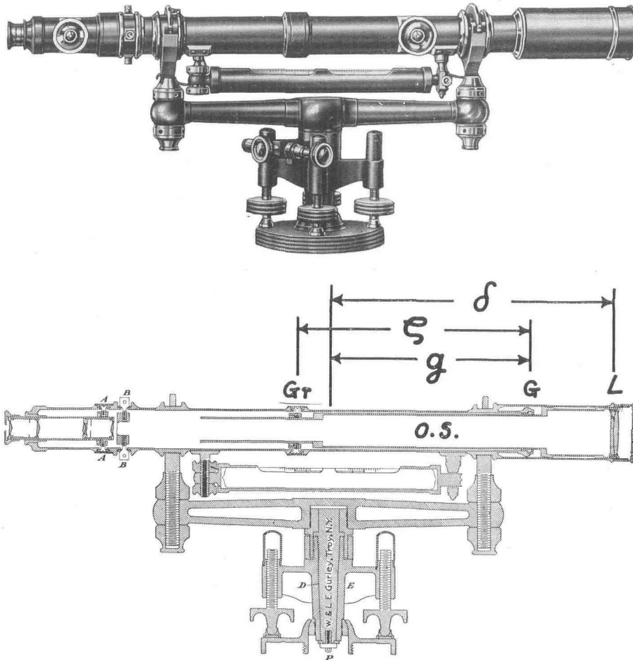
Fig. 47. Sectional View of a Wye Level.
