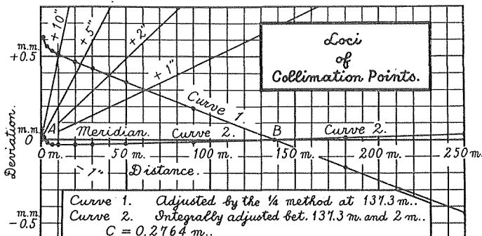
Fig. 35. Illustration of Integral Adjustment of the Vertical Cross-Hair of Transit No. 7.
