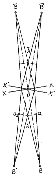
Fig. 44. Illustration of the Adjustment by Old Method A.
