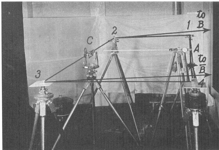
Fig. 32. Apparatus for Test Experiments of Integral Adjustment of the Vertical Cross-hairs.
