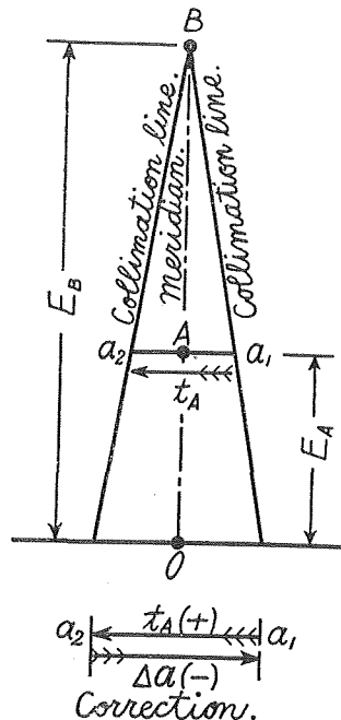
Fig. 28. Second Method of Integral Adjustment.
