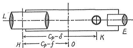
Fig. 4. Porro's Telescope.
