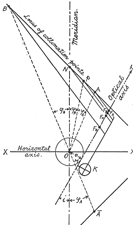
Fig. 19. Optical Relations when Point N is brought on the Meridian of the Transit.
