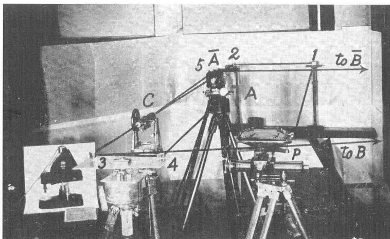
Fig. 22. Apparatus for the First Experiment.
