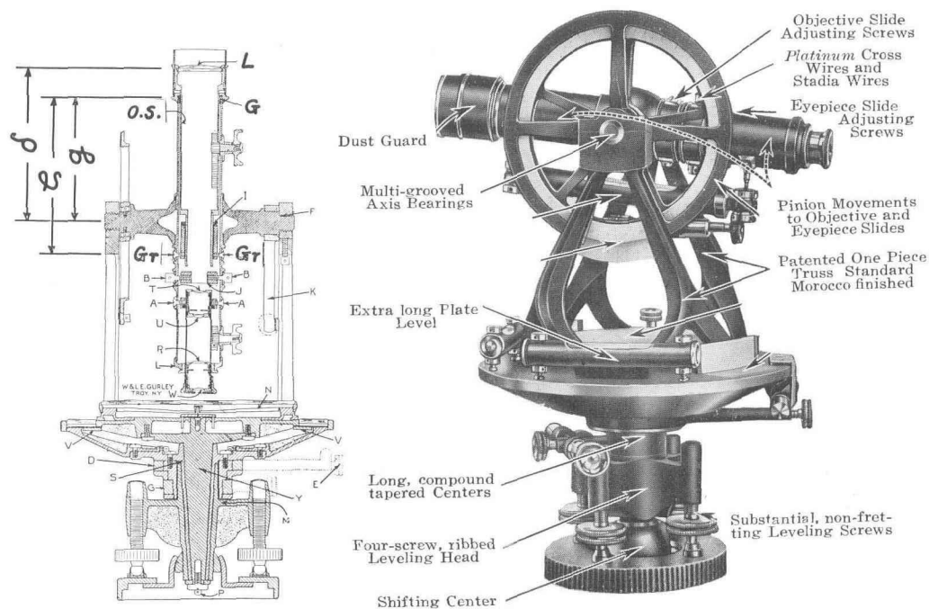
Fig. 16. Cross-Section of a Transit.
