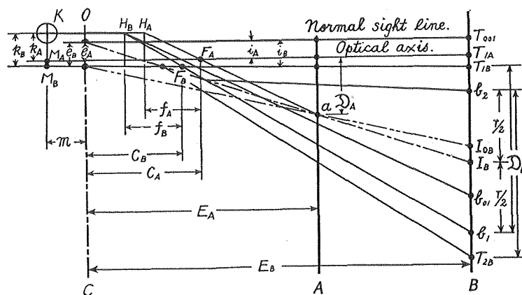
Fig. 10. Optical Relations when the Horizontal Cross-Hair is adjusted by the Second Method of Integral Adjustment.
