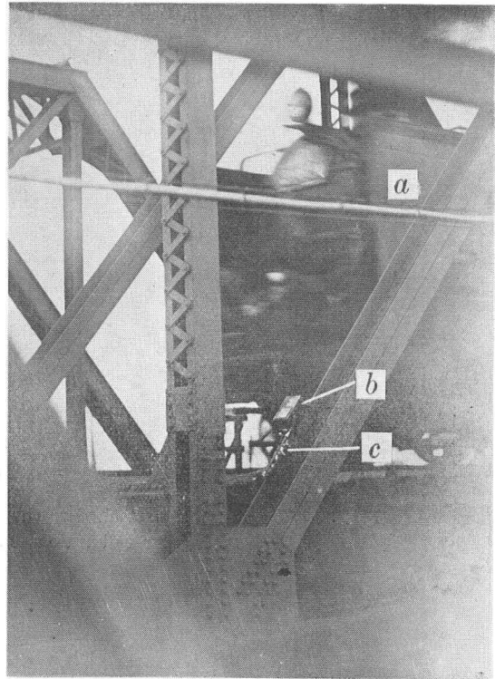
Fig. 11. Strain meters of the writers' and Leuner's in working position.
