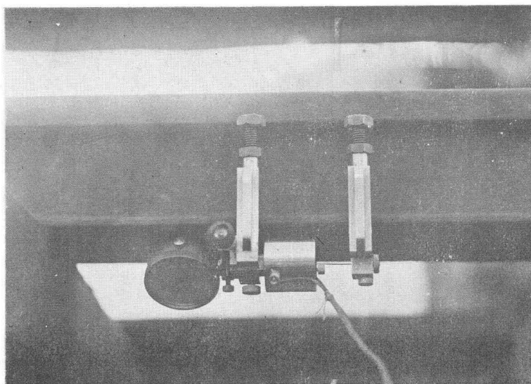
Fig. 9. The apparatus attached to the rail with dial indicator for calibration (2).
