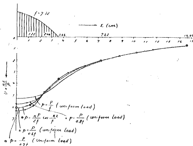
Fig. 20 Comparison of Displacements of Boundary Surface.
