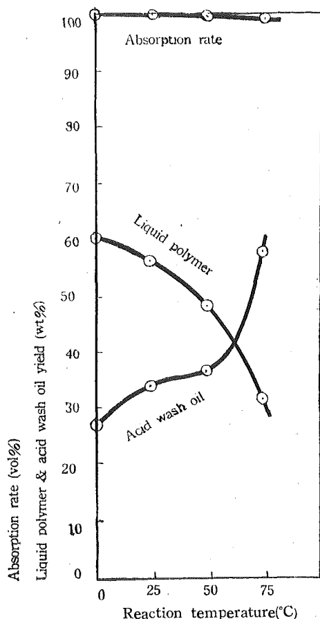
Fig. 3-1 Polymerization of i-butene with 85% acid.
