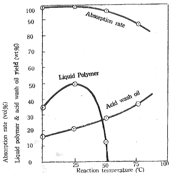
Fig.1-4 Effect of Reaction Temperature with 99% Acid.
