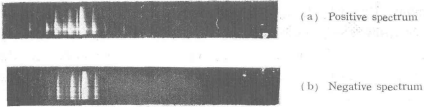
Fig. 13 Spectrum of impulse corona on transformer oil floated on water
