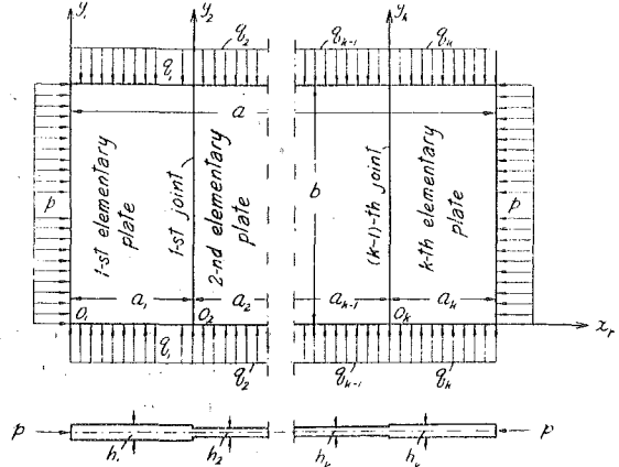
Fig. 1.—Composite plate and system of coordinates.
