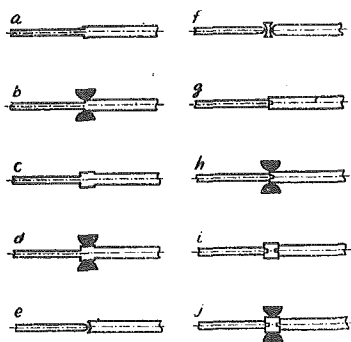
Fig. 2.—Types of intermediate joints.
