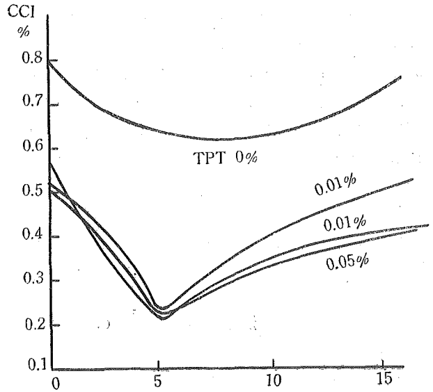
Fig. 4-16 Carbon increase after oxidation.
