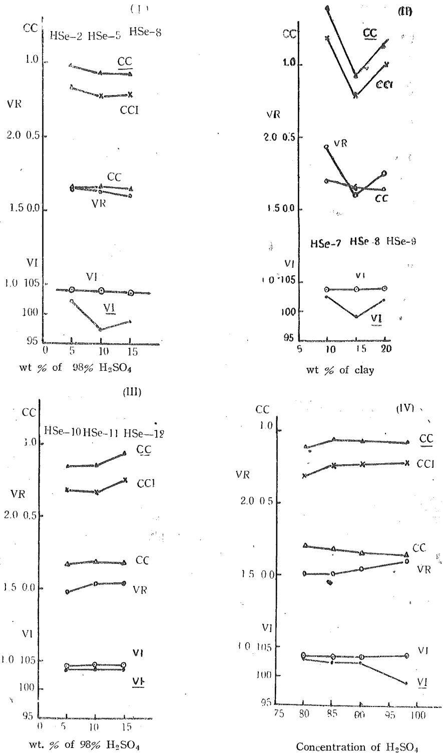
Fig. 3-1 Variation of effect of additives owing to their course of refining. (wt. % of additives are fixed as 10%)
