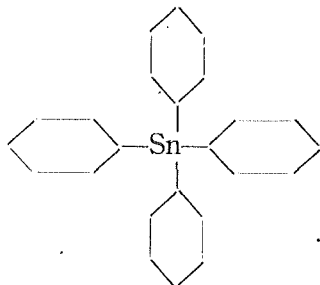
Tetraphenyl tin
