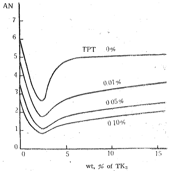
Fig. 4-12 Acid number after oxidation.
